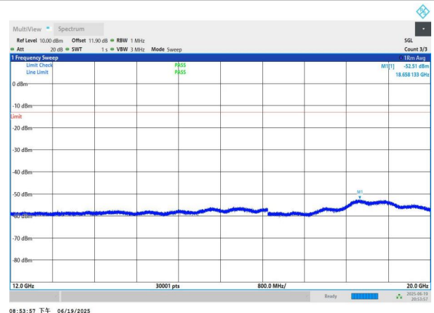
NTNV-n5-PC3-15-5-H-DFT-BPSK-Edge_1RB_Left-12000-20000-P ASS
