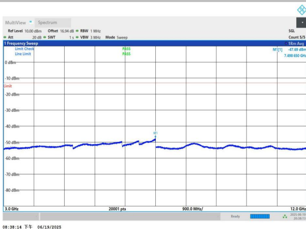
NTNV-n5-PC3-15-5-L-DFT-BPSK-Edge_1RB_Left-3000-12000-P ASS
