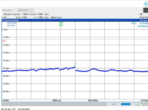
NTNV-n5-PC3-15-5-H-DFT-BPSK-Edge_1RB_Left-3000-12000-P ASS
