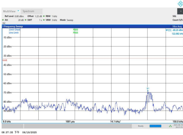
NTNV-n5-PC3-15-5-L-DFT-BPSK-Edge_1RB_Left-0.009-0.15-PA SS
