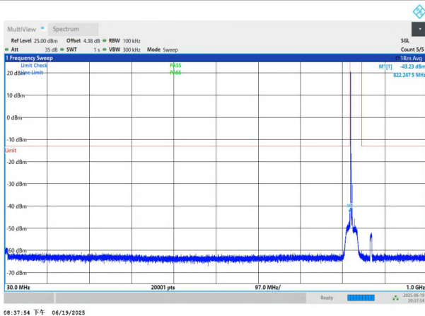
NTNV-n5-PC3-15-5-L-DFT-BPSK-Edge_1RB_Left-30-1000-PAS S
