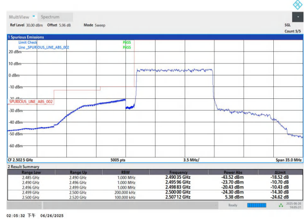
NTNV-n7-PC3-15-10-L-DFT-QPSK-Outer_Full-PASS
