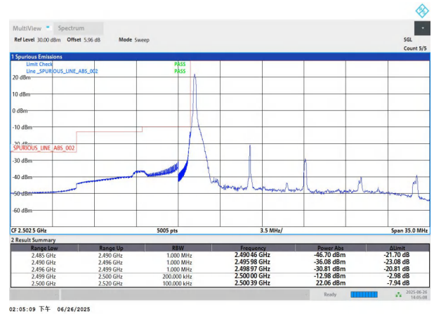
NTNV-n7-PC3-15-10-L-DFT-BPSK-Edge_1RB_Left-PASS
