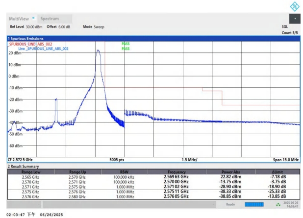
NTNV-n7-PC3-15-5-H-DFT-BPSK-Edge_1RB_Right-PASS
