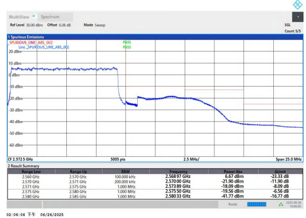
NTNV-n7-PC3-15-10-H-DFT-BPSK-Outer_Full-PASS
