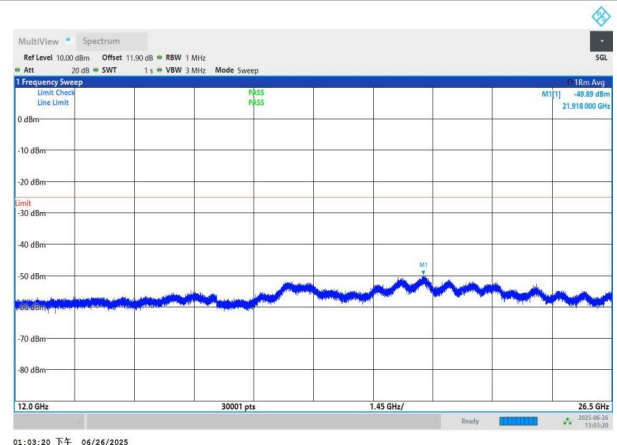
NTNV-n7-PC3-15-10-H-DFT-QPSK-Edge_1RB_Left-12000-26500 -PASS
