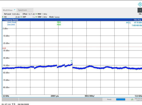
NTNV-n7-PC3-15-15-H-DFT-QPSK-Edge_1RB_Left-3000-12000- PASS
