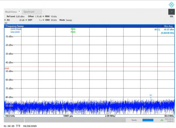
NTNV-n7-PC3-15-15-H-DFT-BPSK-Edge_1RB_Left-0.15-30-PAS S
