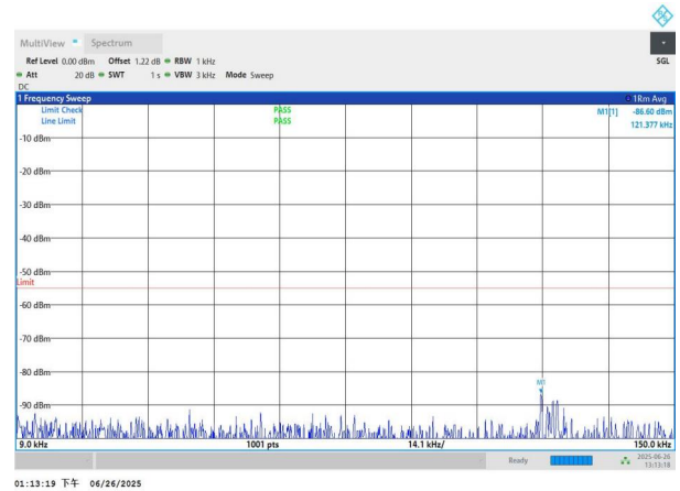
NTNV-n7-PC3-15-25-M-DFT-QPSK-Edge_1RB_Left-0.009-0.15-P ASS
