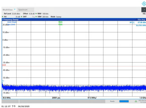
NTNV-n7-PC3-15-25-M-DFT-BPSK-Edge_1RB_Left-30-1000-PA SS
