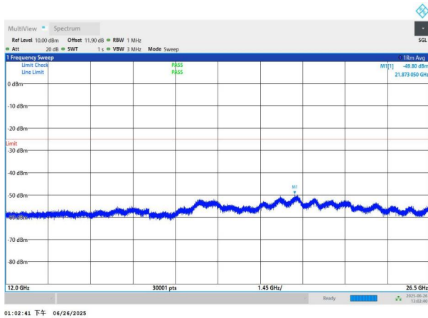
NTNV-n7-PC3-15-10-H-DFT-BPSK-Edge_1RB_Left-12000-26500 -PASS
