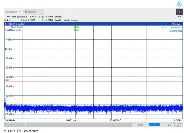
NTNV-n7-PC3-15-10-H-DFT-QPSK-Edge_1RB_Left-30-1000-PAS S
