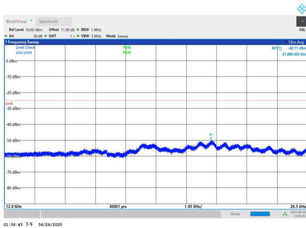
NTNV-n7-PC3-15-15-H-DFT-BPSK-Edge_1RB_Left-12000-26500 -PASS
