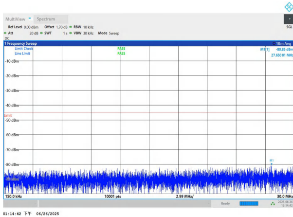
NTNV-n7-PC3-15-25-H-DFT-QPSK-Edge_1RB_Left-0.15-30-PAS S
