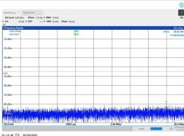
NTNV-n7-PC3-15-25-M-DFT-QPSK-Edge_1RB_Left-0.15-30-PAS S
