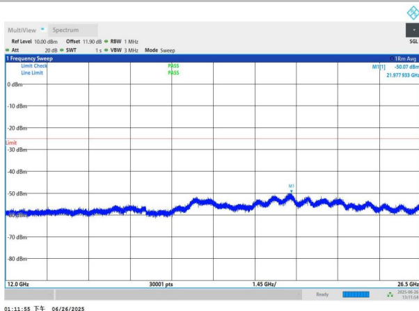
NTNV-n7-PC3-15-25-L-DFT-BPSK-Edge_1RB_Left-12000-26500
