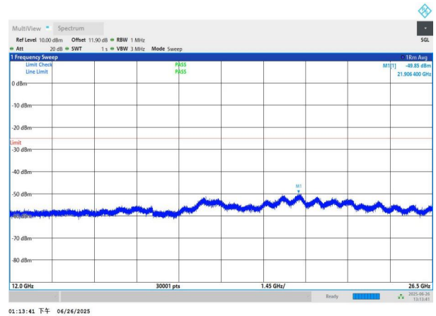
NTNV-n7-PC3-15-25-M-DFT-QPSK-Edge_1RB_Left-12000-2650 0-PASS
