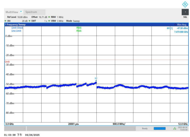
NTNV-n7-PC3-15-15-L-DFT-BPSK-Edge_1RB_Left-3000-12000-PASS
