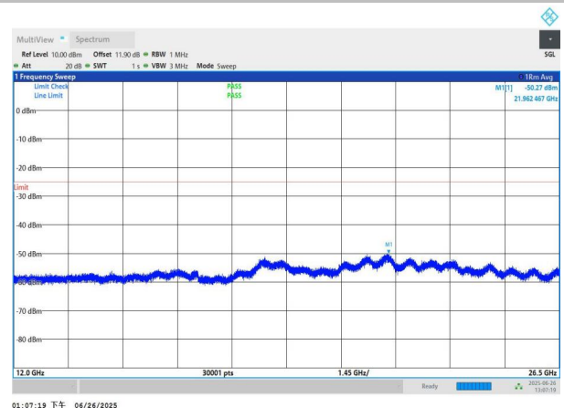
NTNV-n7-PC3-15-15-H-DFT-QPSK-Edge_1RB_Left-12000-26500 -PASS
