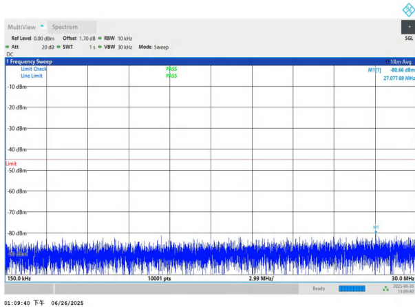
NTNV-n7-PC3-15-20-M-DFT-QPSK-Edge_1RB_Left-0.15-30-PAS S
