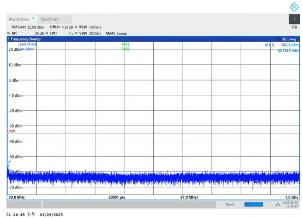
NTNV-n7-PC3-15-25-H-DFT-QPSK-Edge_1RB_Left-30-1000-PAS S
