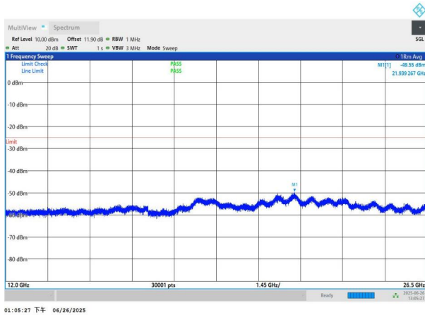
NTNV-n7-PC3-15-15-M-DFT-BPSK-Edge_1RB_Left-12000-2650 0-PASS
