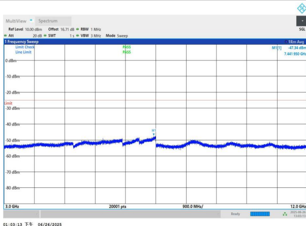
NTNV-n7-PC3-15-10-H-DFT-QPSK-Edge_1RB_Left-3000-12000- PASS
