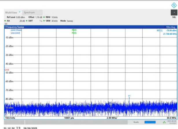
NTNV-n7-PC3-15-25-M-DFT-BPSK-Edge_1RB_Left-0.15-30-PAS
