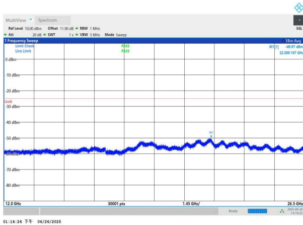
NTNV-n7-PC3-15-25-H-DFT-BPSK-Edge_1RB_Left-12000-26500 -PASS
