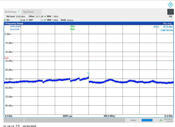
NTNV-n7-PC3-15-25-H-DFT-BPSK-Edge_1RB_Left-3000-12000- PASS
