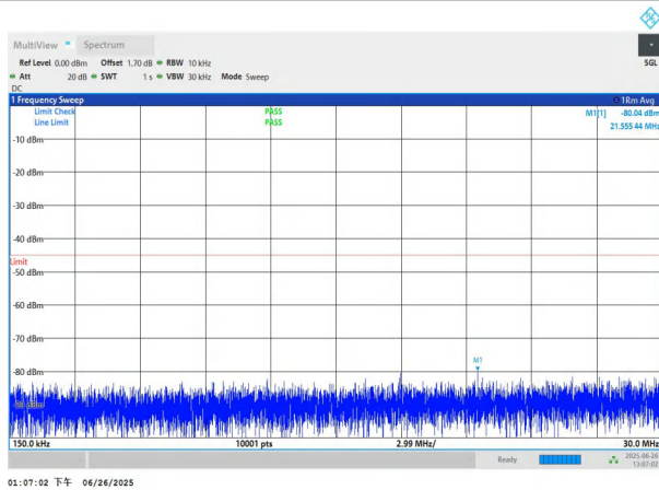
NTNV-n7-PC3-15-15-H-DFT-QPSK-Edge_1RB_Left-0.15-30-PAS S
