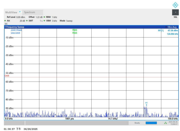
NTNV-n7-PC3-15-15-H-DFT-QPSK-Edge_1RB_Left-0.009-0.15-P ASS
