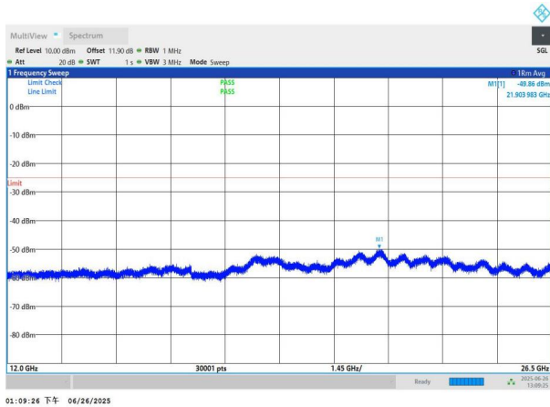
NTNV-n7-PC3-15-20-M-DFT-BPSK-Edge_1RB_Left-12000-2650 0-PASS
