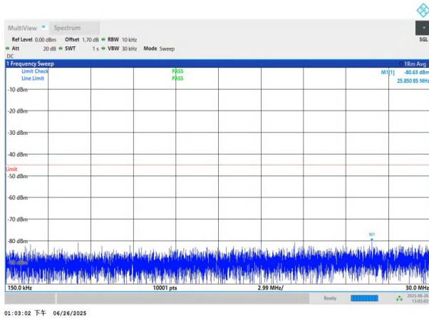
NTNV-n7-PC3-15-10-H-DFT-QPSK-Edge_1RB_Left-0.15-30-PAS S
