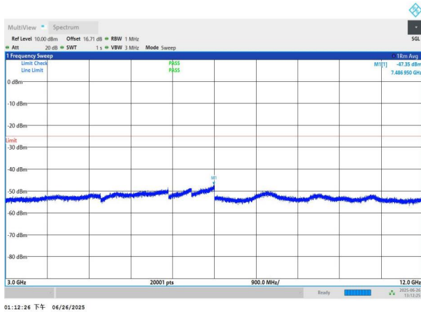
NTNV-n7-PC3-15-25-L-DFT-QPSK-Edge_1RB_Left-3000-12000-
