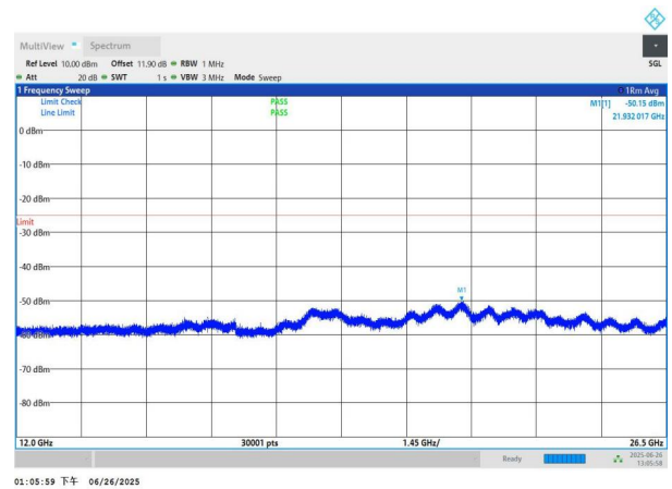
NTNV-n7-PC3-15-15-M-DFT-QPSK-Edge_1RB_Left-12000-2650 0-PASS
