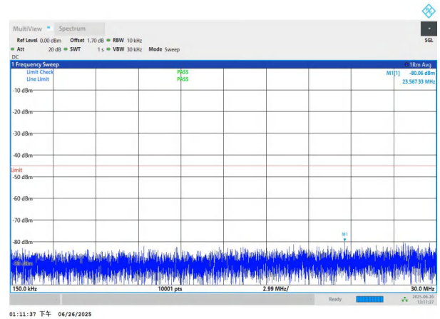
NTNV-n7-PC3-15-25-L-DFT-BPSK-Edge_1RB_Left-0.15-30-PAS
