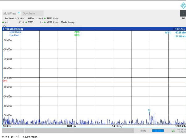
NTNV-n7-PC3-15-25-M-DFT-BPSK-Edge_1RB_Left-0.009-0.15-P
