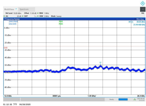
NTNV-n7-PC3-15-25-L-DFT-QPSK-Edge_1RB_Left-12000-26500
