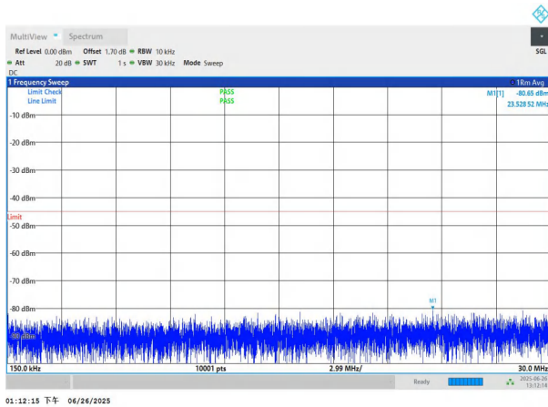
NTNV-n7-PC3-15-25-L-DFT-QPSK-Edge_1RB_Left-0.15-30-PAS
