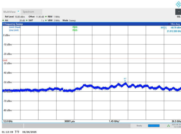
NTNV-n7-PC3-15-25-M-DFT-BPSK-Edge_1RB_Left-12000-2650 0-PASS
