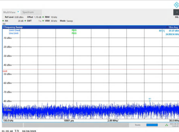
NTNV-n7-PC3-15-15-M-DFT-QPSK-Edge_1RB_Left-0.15-30-PAS S
