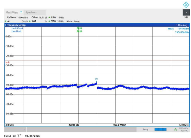
NTNV-n7-PC3-15-25-M-DFT-BPSK-Edge_1RB_Left-3000-12000- PASS
