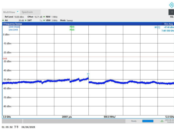
NTNV-n7-PC3-15-15-M-DFT-QPSK-Edge_1RB_Left-3000-12000- PASS
