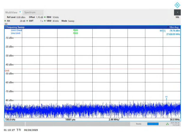
NTNV-n7-PC3-15-30-L-DFT-BPSK-Edge_1RB_Left-0.15-30-PAS
