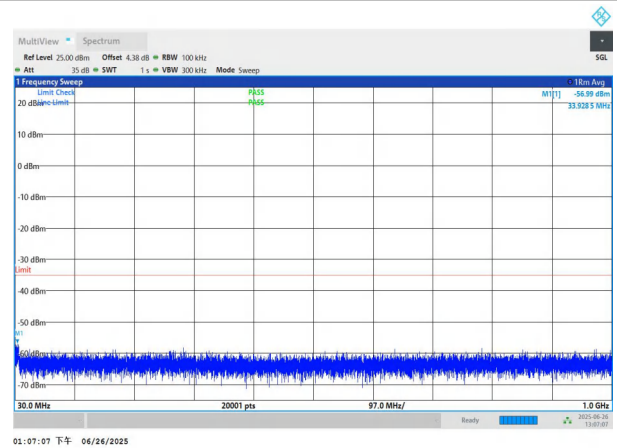
NTNV-n7-PC3-15-15-H-DFT-QPSK-Edge_1RB_Left-30-1000-PAS S
