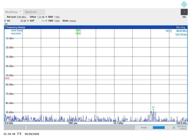
NTNV-n7-PC3-15-20-M-DFT-QPSK-Edge_1RB_Left-0.009-0.15-P ASS
