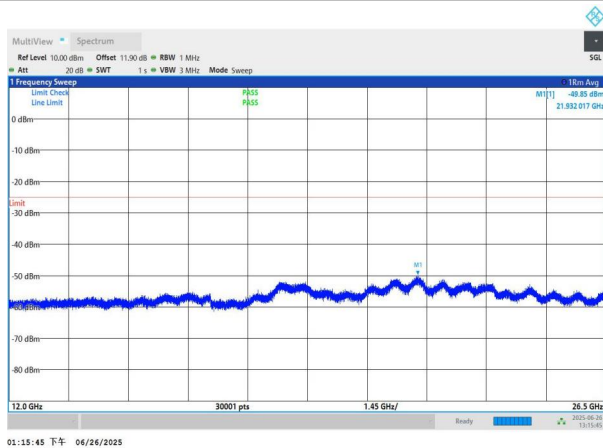
NTNV-n7-PC3-15-30-L-DFT-BPSK-Edge_1RB_Left-12000-26500
