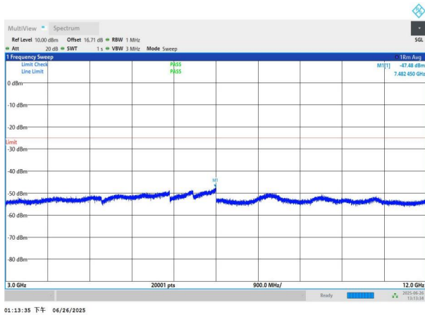
NTNV-n7-PC3-15-25-M-DFT-QPSK-Edge_1RB_Left-3000-12000- PASS
