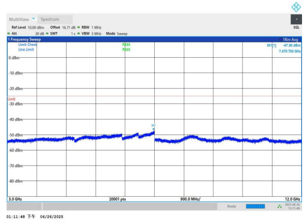
NTNV-n7-PC3-15-25-L-DFT-BPSK-Edge_1RB_Left-3000-12000-
