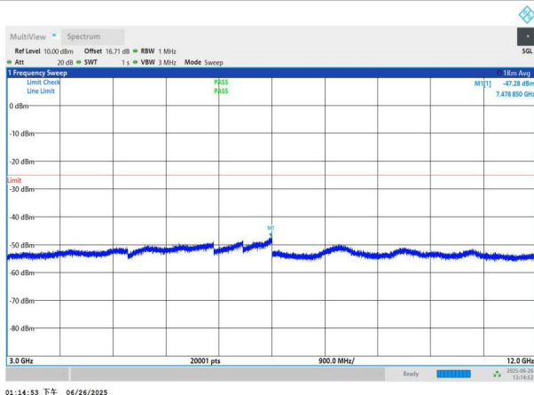
NTNV-n7-PC3-15-25-H-DFT-QPSK-Edge_1RB_Left-3000-12000- PASS
