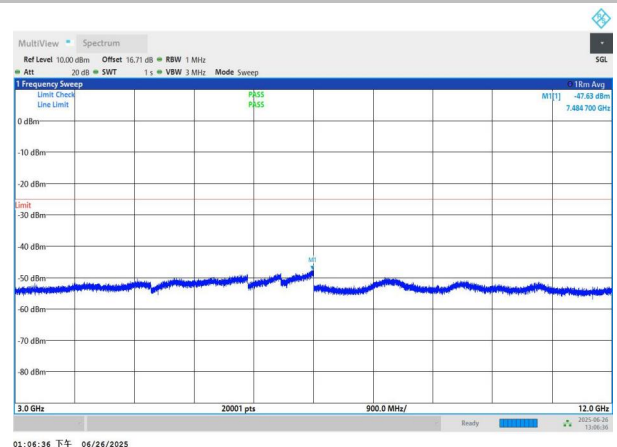
NTNV-n7-PC3-15-15-H-DFT-BPSK-Edge_1RB_Left-3000-12000- PASS
