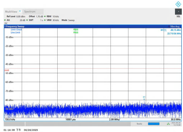
NTNV-n7-PC3-15-25-H-DFT-BPSK-Edge_1RB_Left-0.15-30-PAS S
