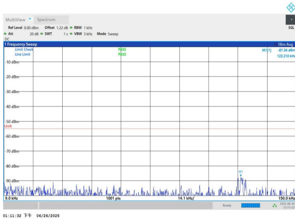
NTNV-n7-PC3-15-25-L-DFT-BPSK-Edge_1RB_Left-0.009-0.15-P
