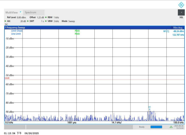
NTNV-n7-PC3-15-30-L-DFT-QPSK-Edge_1RB_Left-0.009-0.15-P
