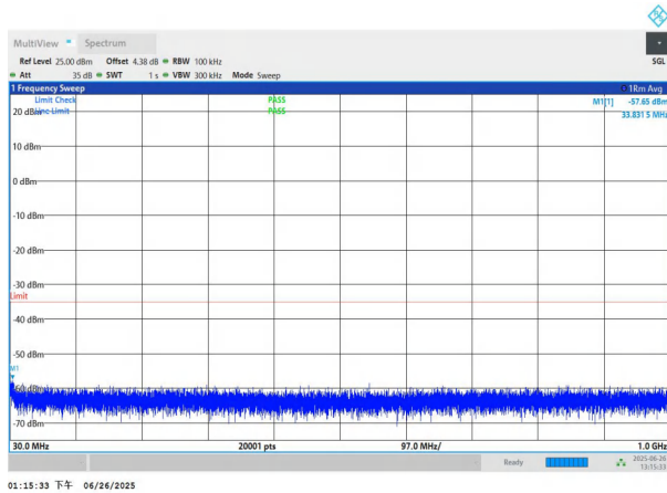
NTNV-n7-PC3-15-30-L-DFT-BPSK-Edge_1RB_Left-30-1000-PAS
