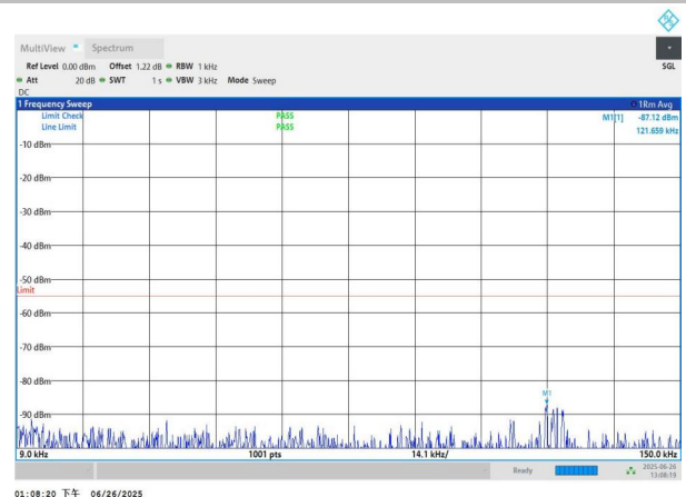
NTNV-n7-PC3-15-20-L-DFT-QPSK-Edge_1RB_Left-0.009-0.15-P
