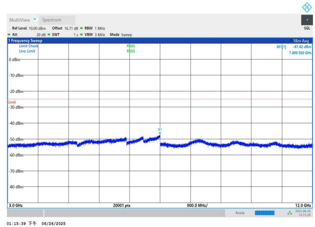
NTNV-n7-PC3-15-30-L-DFT-BPSK-Edge_1RB_Left-3000-12000-PASS
