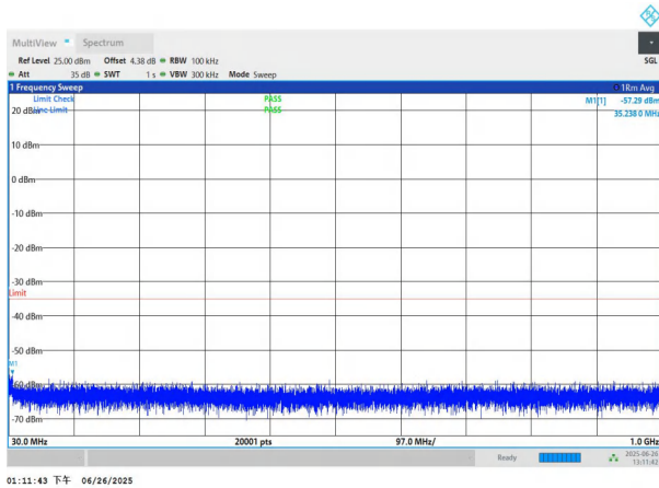
NTNV-n7-PC3-15-25-L-DFT-BPSK-Edge_1RB_Left-30-1000-PAS
