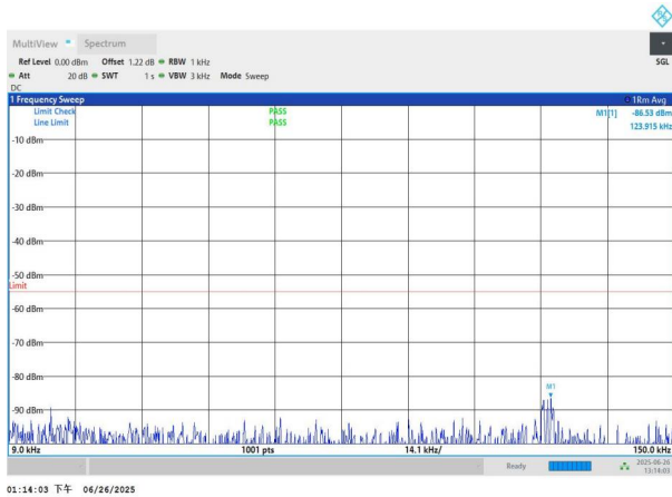
NTNV-n7-PC3-15-25-H-DFT-BPSK-Edge_1RB_Left-0.009-0.15-P ASS
