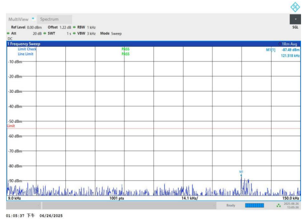
NTNV-n7-PC3-15-15-M-DFT-QPSK-Edge_1RB_Left-0.009-0.15-P ASS
