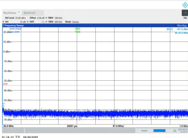
NTNV-n7-PC3-15-25-H-DFT-BPSK-Edge_1RB_Left-30-1000-PAS S
