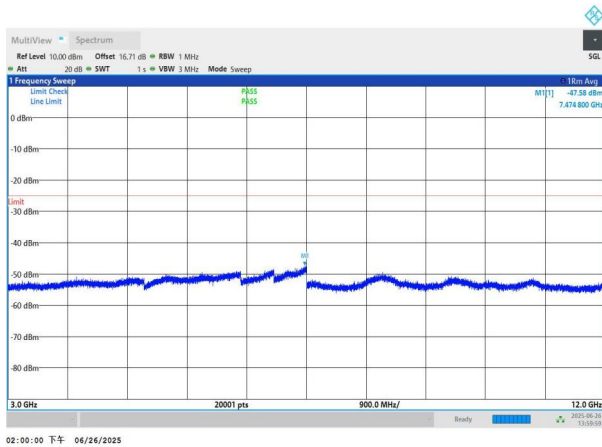
NTNV-n7-PC3-15-40-M-DFT-QPSK-Edge_1RB_Left-3000-12000- PASS
