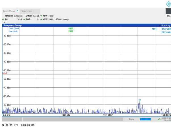
NTNV-n7-PC3-15-40-H-DFT-BPSK-Edge_1RB_Left-0.009-0.15-P ASS
