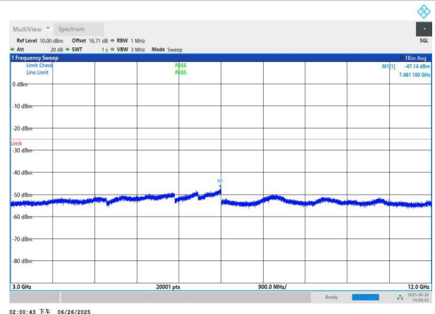
NTNV-n7-PC3-15-40-H-DFT-BPSK-Edge_1RB_Left-3000-12000- PASS
