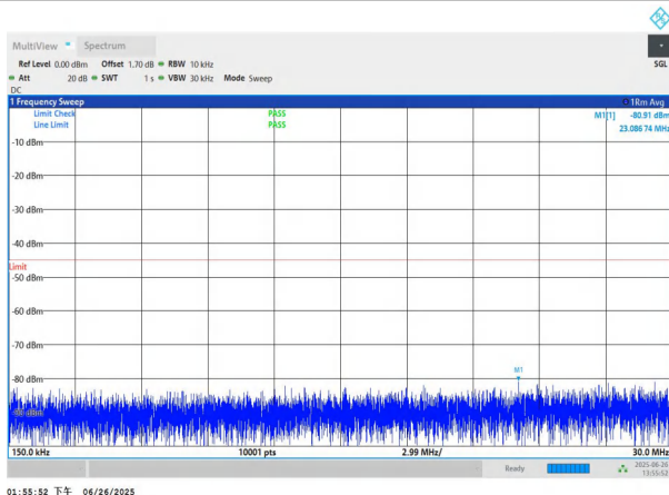
NTNV-n7-PC3-15-30-M-DFT-QPSK-Edge_1RB_Left-0.15-30-PAS S
