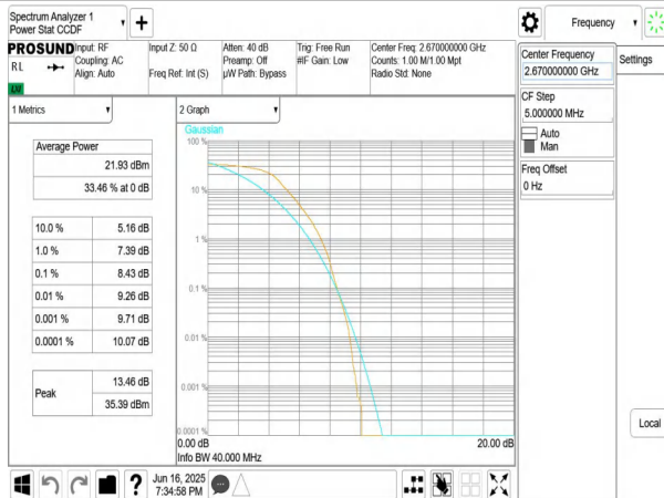
NTNV-n41-PC3-30-40-H-DFT-BPSK-Outer_Full-PASS
