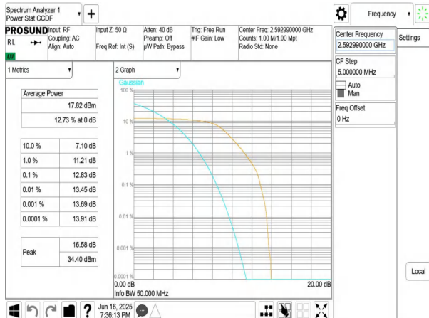
NTNV-n41-PC3-30-50-M-DFT-BPSK-Outter_Full-PASS
