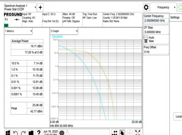
NTNV-n41-PC3-30-20-M-DFT-QPSK-Outter_Full-PASS
