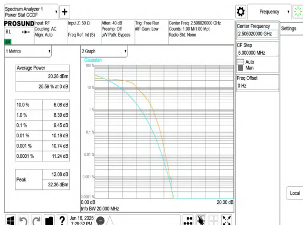
NTNV-n41-PC3-30-20-L-DFT-BPSK-Outter_Full-PASS
