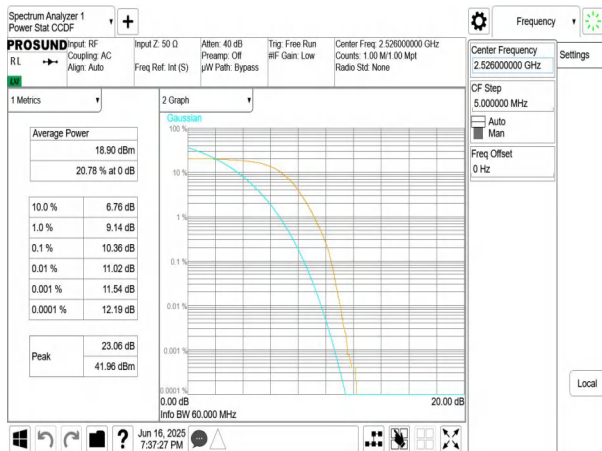
NTNV-n41-PC3-30-60-L-DFT-BPSK-Outer_Full-PASS
