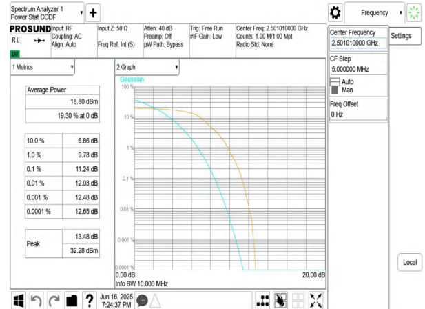
NTNV-n41-PC3-30-10-L-DFT-QPSK-Outer_Full-PASS
