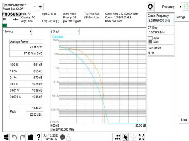
NTNV-n41-PC3-30-50-L-DFT-BPSK-Outter_Full-PASS
