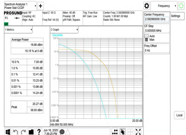
NTNV-n41-PC3-30-50-M-DFT-QPSK-Outter_Full-PASS
