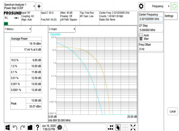
NTNV-n41-PC3-30-50-L-DFT-QPSK-Outter_Full-PASS
