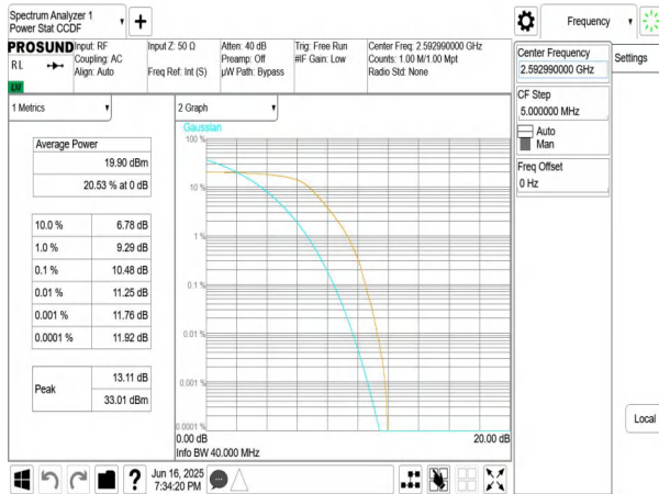
NTNV-n41-PC3-30-40-M-DFT-BPSK-Outer_Full-PASS
