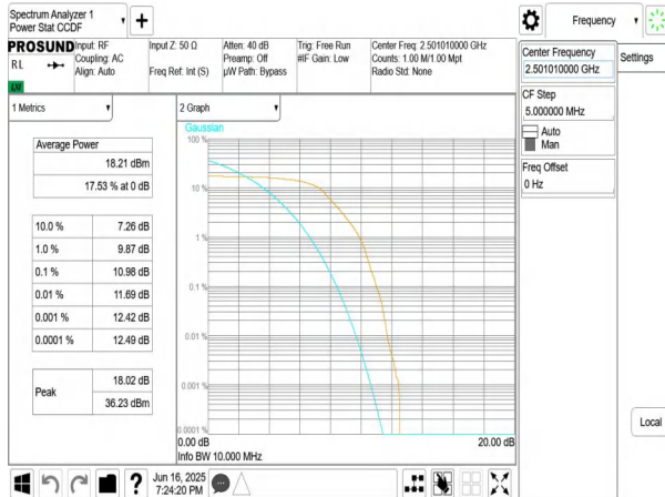
NTNV-n41-PC3-30-10-L-DFT-BPSK-Outer_Full-PASS
