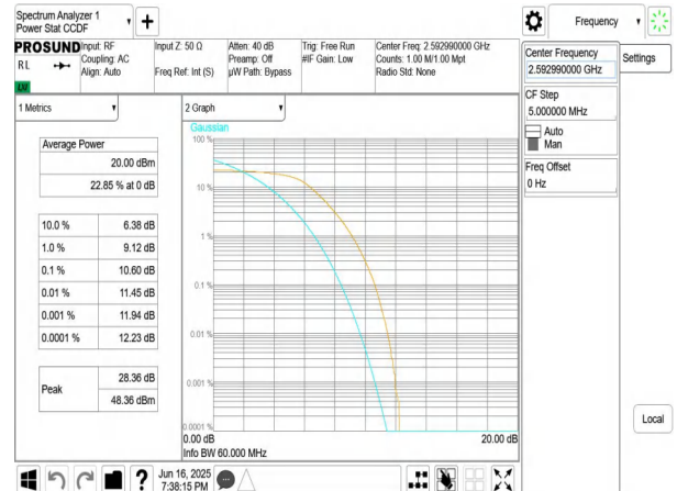
NTNV-n41-PC3-30-60-M-DFT-QPSK-Outer_Full-PASS
