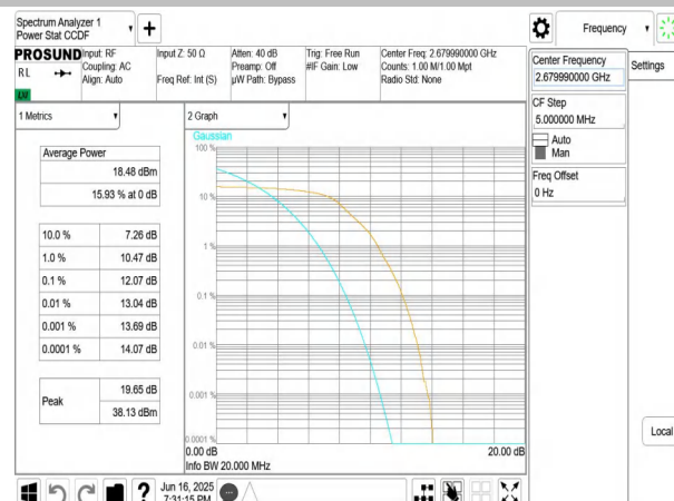
NTNV-n41-PC3-30-20-H-DFT-QPSK-Outter_Full-PASS
