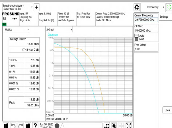
NTNV-n41-PC3-30-20-H-DFT-BPSK-Outter_Full-PASS
