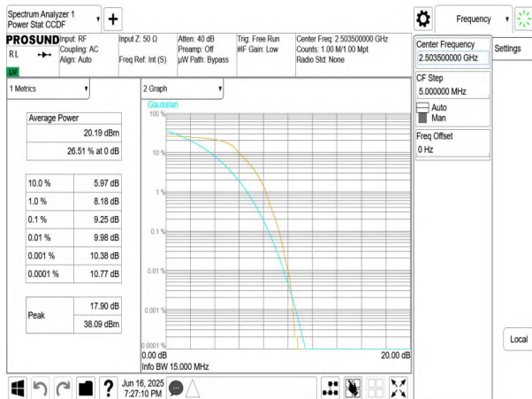
NTNV-n41-PC3-30-15-L-DFT-BPSK-Outer_Full-PASS
