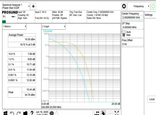
NTNV-n41-PC3-30-20-M-DFT-BPSK-Outter_Full-PASS
