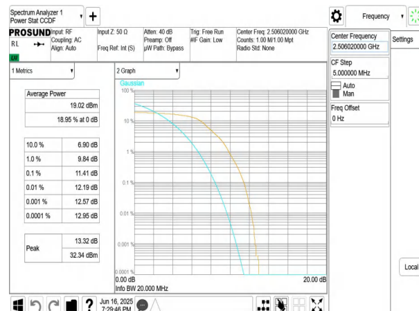
NTNV-n41-PC3-30-20-L-DFT-QPSK-Outter_Full-PASS
