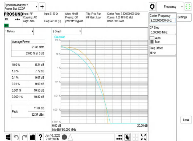
NTNV-n41-PC3-30-60-L-DFT-QPSK-Outer_Full-PASS
