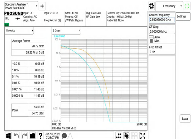
NTNV-n41-PC3-30-15-M-DFT-QPSK-Outer_Full-PASS
