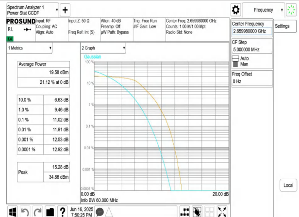
NTNV-n41-PC3-30-60-H-DFT-QPSK-Outer_Full-PASS
