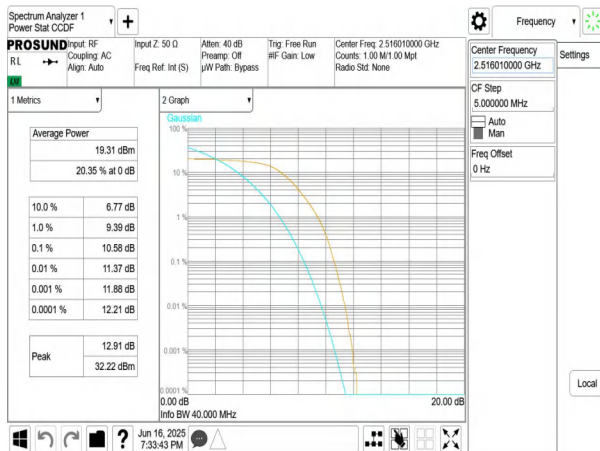
NTNV-n41-PC3-30-40-L-DFT-BPSK-Outer_Full-PASS
