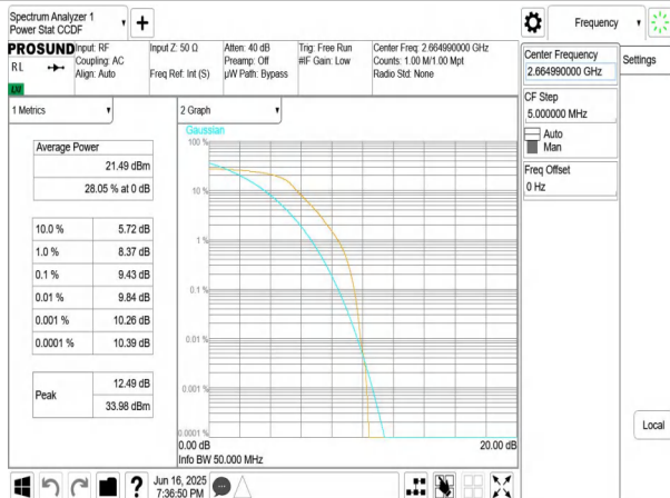
NTNV-n41-PC3-30-50-H-DFT-BPSK-Outter_Full-PASS
