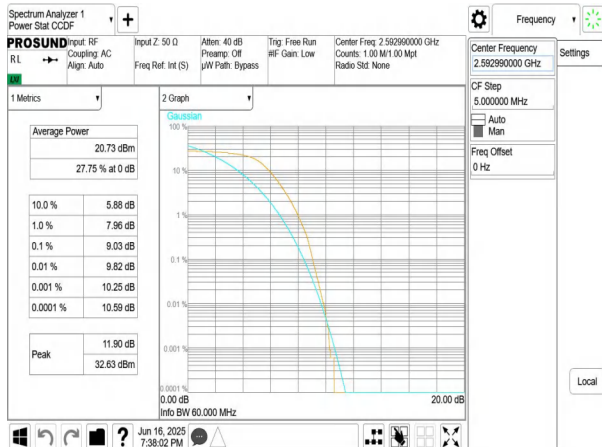
NTNV-n41-PC3-30-60-M-DFT-BPSK-Outer_Full-PASS
