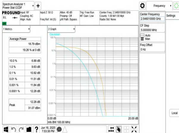
NTNV-n41-PC3-30-100-L-DFT-BPSK-Outer_Full-PASS
