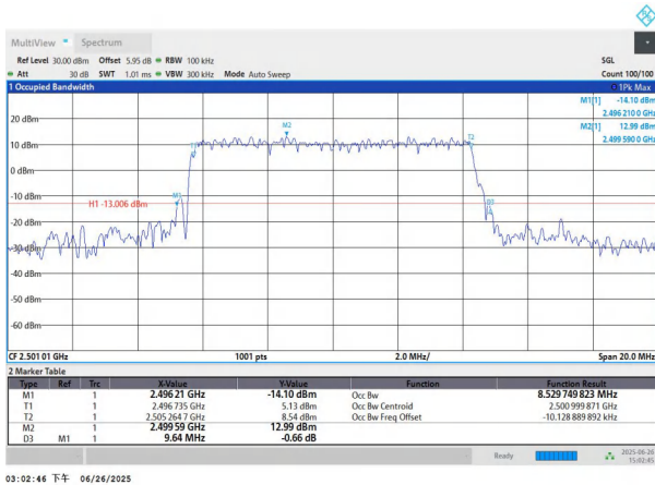
NTNV-n41-PC3-30-10-L-DFT-256QAM-Outet-Full-Ant1-PASS
