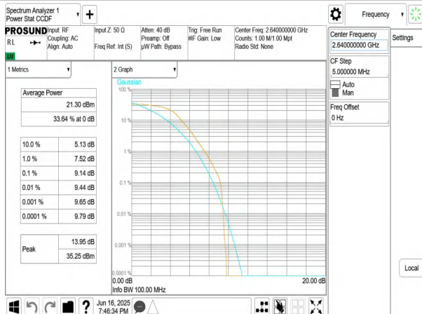
NTNV-n41-PC3-30-100-H-DFT-BPSK-Outer_Full-PASS
