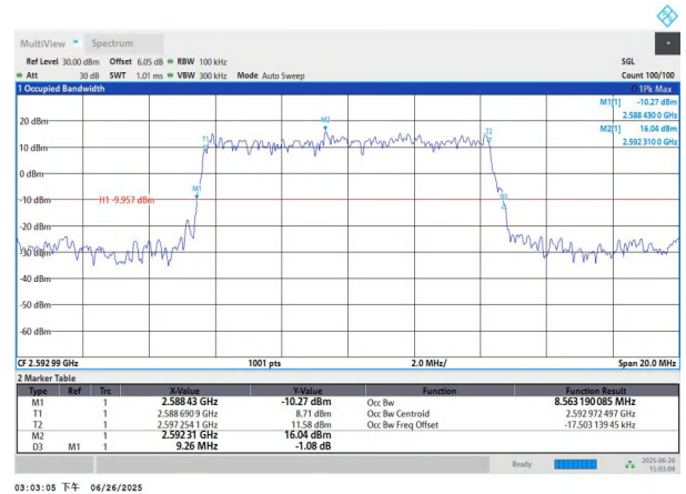
NTNV-n41-PC3-30-10-M-DFT-BPSK-Outet-Full-Ant1-PASS
