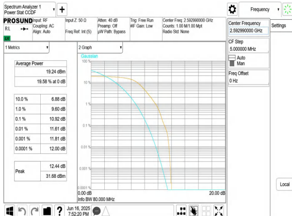
NTNV-n41-PC3-30-80-M-DFT-BPSK-Outer_Full-PASS
