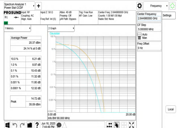
NTNV-n41-PC3-30-90-H-DFT-QPSK-Outter_Full-PASS
