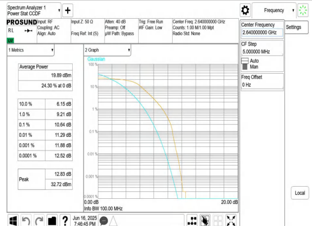
NTNV-n41-PC3-30-100-H-DFT-QPSK-Outer_Full-PASS
