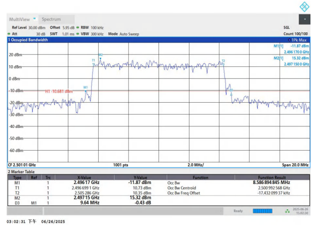
NTNV-n41-PC3-30-10-L-DFT-64QAM-Outet-Full-Ant1-PASS
