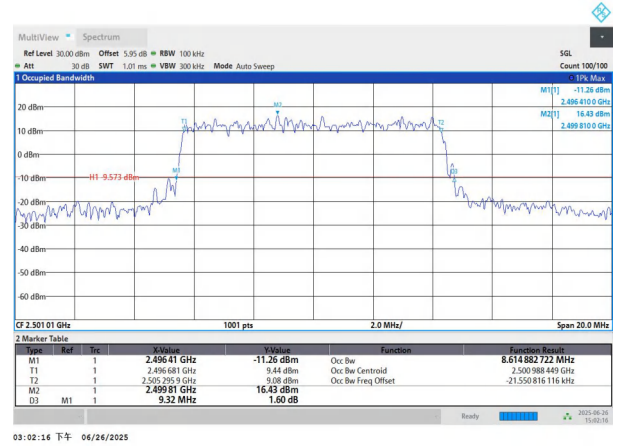
NTNV-n41-PC3-30-10-L-DFT-QPSK-Outet-Full-Ant1-PASS
