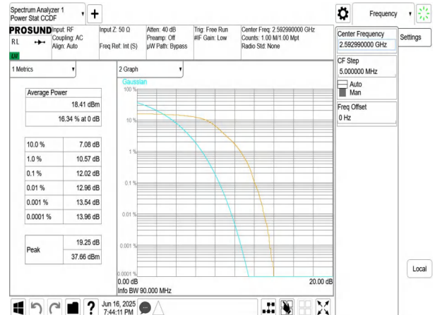
NTNV-n41-PC3-30-90-M-DFT-QPSK-Outter_Full-PASS
