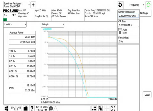
NTNV-n41-PC3-30-100-M-DFT-QPSK-Outer_Full-PASS
