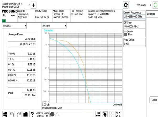
NTNV-n41-PC3-30-90-M-DFT-BPSK-Outter_Full-PASS
