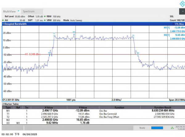
NTNV-n41-PC3-30-10-L-DFT-BPSK-Outet-Full-Ant1-PASS
