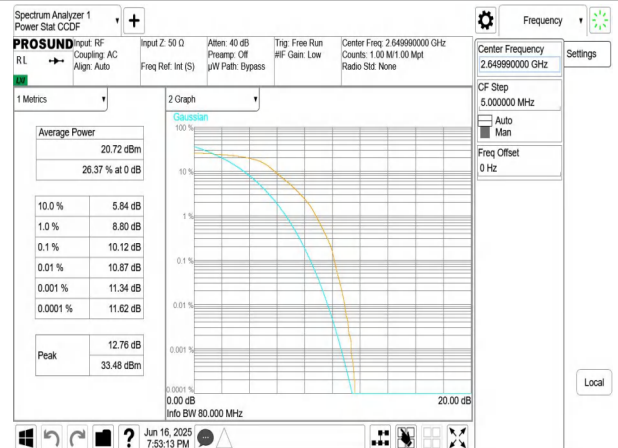
NTNV-n41-PC3-30-80-H-DFT-QPSK-Outer_Full-PASS
