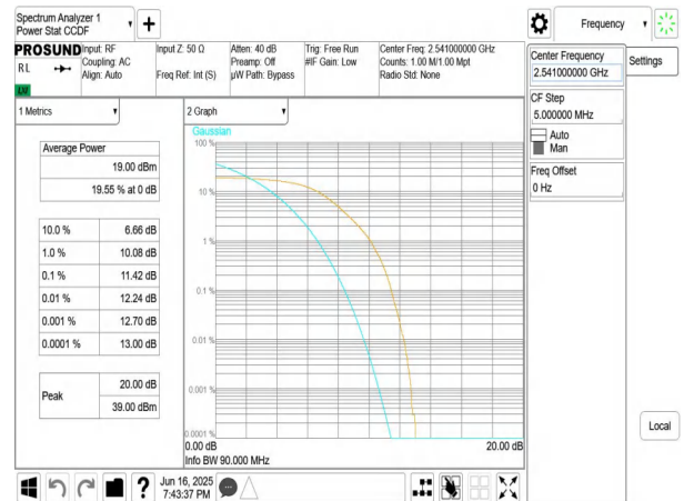
NTNV-n41-PC3-30-90-L-DFT-QPSK-Outter_Full-PASS
