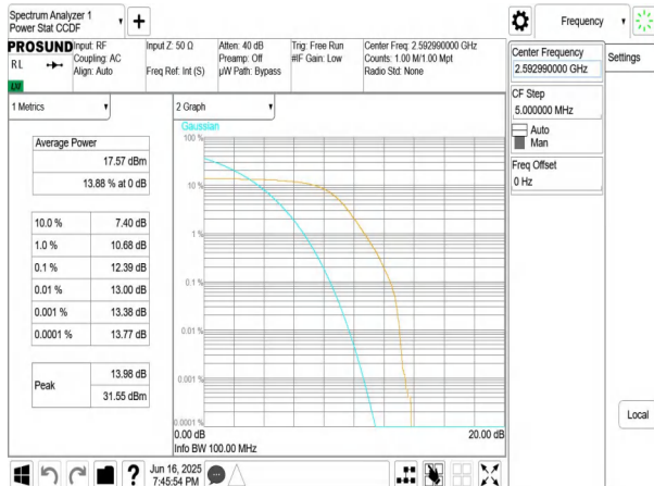
NTNV-n41-PC3-30-100-M-DFT-BPSK-Outer_Full-PASS
