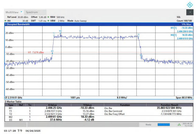
NTNV-n41-PC3-30-40-L-DFT-QPSK-Outet_Full-Ant1-PASS
