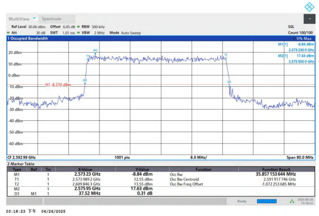
NTNV-n41-PC3-30-40-M-DFT-BPSK-Outet_Full-Ant1-PASS
