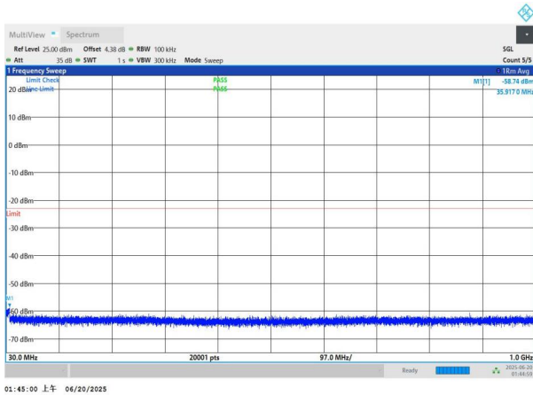
NTNV-n66-PC3-15-20-L-DFT-BPSK-Edge_1RB_Left-30-1000-PA SS
