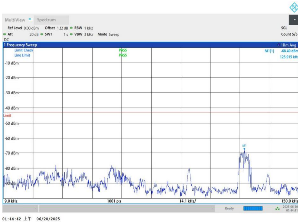
NTNV-n66-PC3-15-20-L-DFT-BPSK-Edge_1RB_Left-0.009-0.15- PASS
