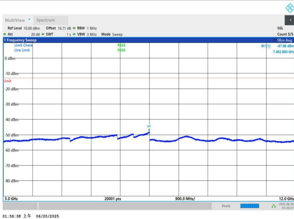
NTNV-n66-PC3-15-10-H-DFT-QPSK-Edge_1RB_Left-3000-1200 0-PASS
