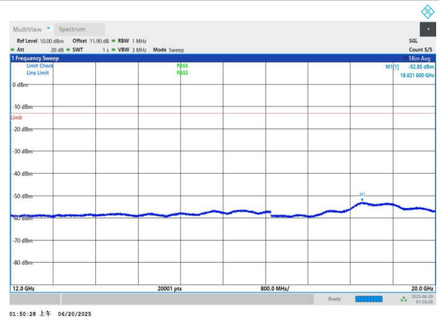
NTNV-n66-PC3-15-20-H-DFT-BPSK-Edge_1RB_Left-12000-2000 0-PASS
