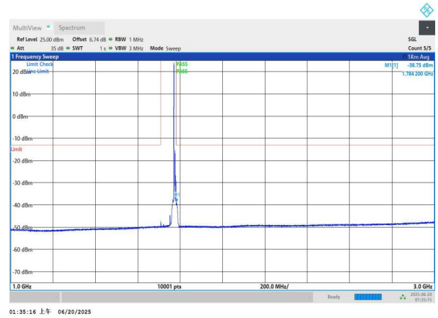
NTNV-n66-PC3-15-10-H-DFT-BPSK-Edge_1RB_Left-1000-3000-P ASS
