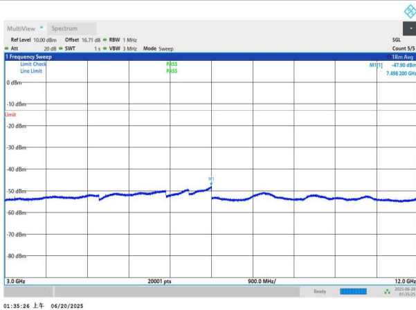
NTNV-n66-PC3-15-10-H-DFT-BPSK-Edge_1RB_Left-3000-1200 0-PASS
