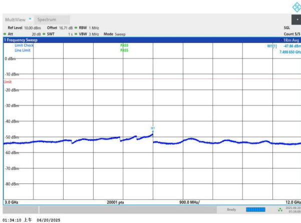
NTNV-n66-PC3-15-10-M-DFT-QPSK-Edge_1RB_Left-3000-1200 0-PASS
