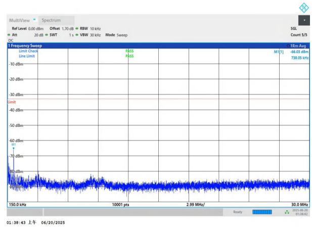
NTNV-n66-PC3-15-15-L-DFT-QPSK-Edge_1RB_Left-0.15-30-PAS S
