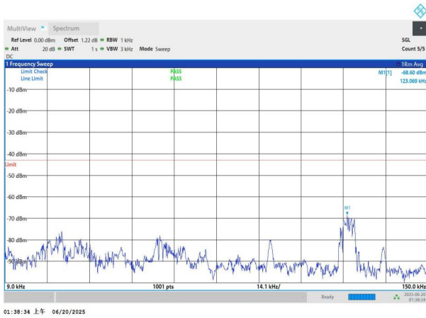
NTNV-n66-PC3-15-15-L-DFT-QPSK-Edge_1RB_Left-0.009-0.15- PASS
