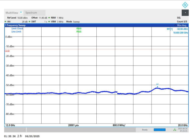
NTNV-n66-PC3-15-10-H-DFT-BPSK-Edge_1RB_Left-12000-2000 0-PASS
