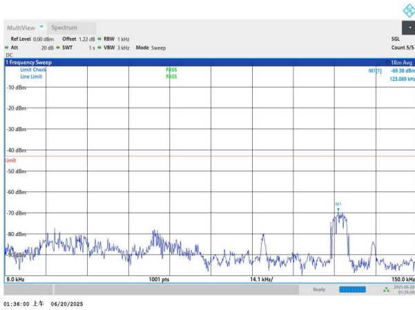
NTNV-n66-PC3-15-10-H-DFT-QPSK-Edge_1RB_Left-0.009-0.15- PASS
