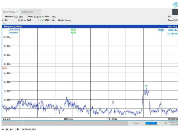
NTNV-n66-PC3-15-20-H-DFT-BPSK-Edge_1RB_Left-0.009-0.15- PASS
