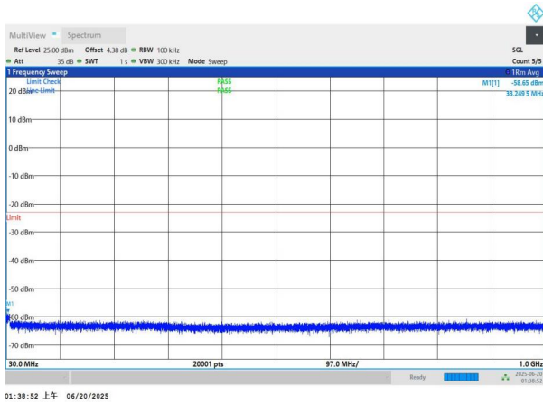
NTNV-n66-PC3-15-15-L-DFT-QPSK-Edge_1RB_Left-30-1000-PA SS
