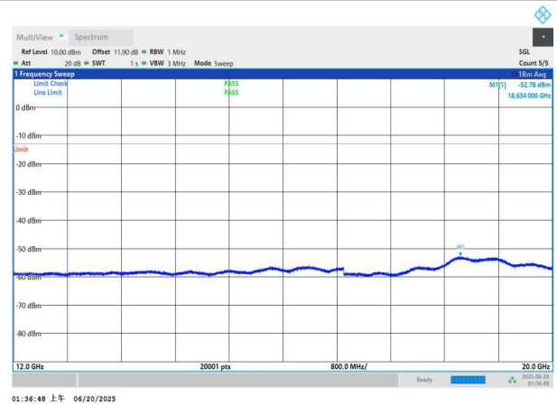
NTNV-n66-PC3-15-10-H-DFT-QPSK-Edge_1RB_Left-12000-2000 0-PASS
