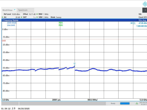
NTNV-n66-PC3-15-15-L-DFT-QPSK-Edge_1RB_Left-3000-1200 0-PASS
