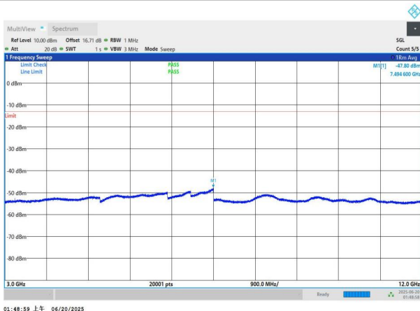
NTNV-n66-PC3-15-20-M-DFT-QPSK-Edge_1RB_Left-3000-1200 0-PASS
