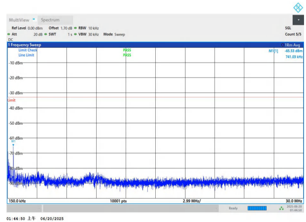
NTNV-n66-PC3-15-20-L-DFT-BPSK-Edge_1RB_Left-0.15-30-PAS S
