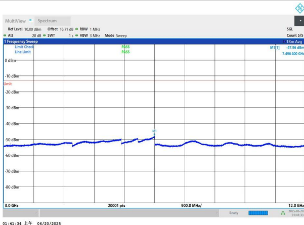
NTNV-n66-PC3-15-15-M-DFT-QPSK-Edge_1RB_Left-3000-1200 0-PASS
