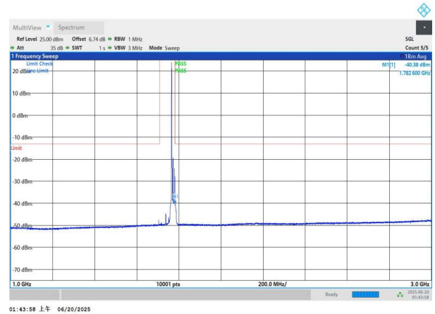
NTNV-n66-PC3-15-15-H-DFT-QPSK-Edge_1RB_Left-1000-3000- PASS
