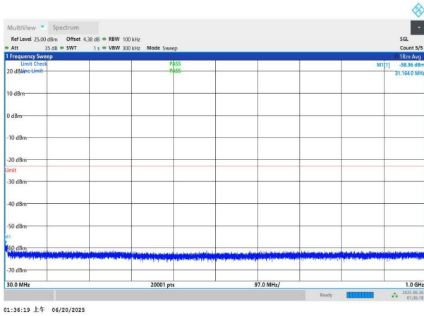
NTNV-n66-PC3-15-10-H-DFT-QPSK-Edge_1RB_Left-30-1000-P ASS
