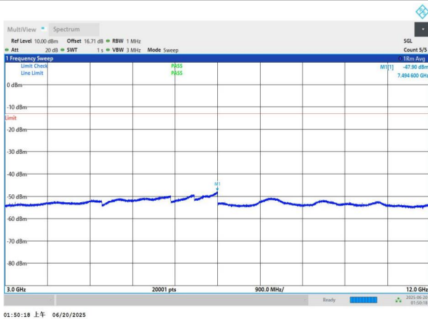
NTNV-n66-PC3-15-20-H-DFT-BPSK-Edge_1RB_Left-3000-1200 0-PASS
