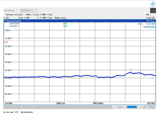
NTNV-n66-PC3-15-15-M-DFT-QPSK-Edge_1RB_Left-12000-2000 0-PASS
