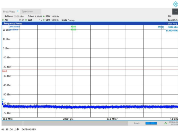
NTNV-n66-PC3-15-10-H-DFT-BPSK-Edge_1RB_Left-30-1000-P ASS
