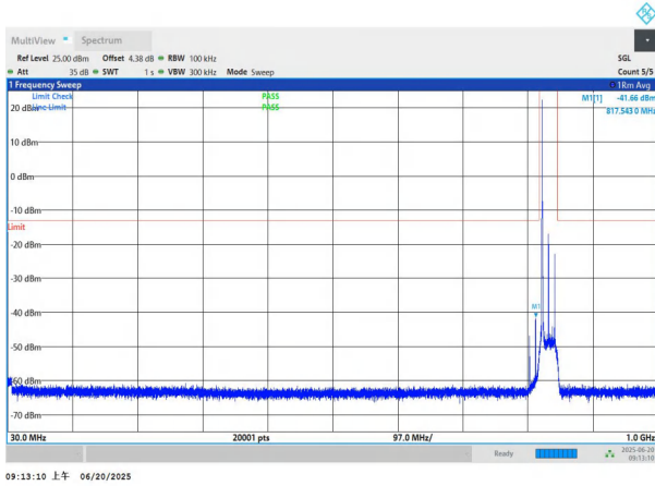
NTNV-n26(824-849)-PC3-15-20-M-DFT-BPSK-Edge_1RB_Left-3 0-1000-PASS
