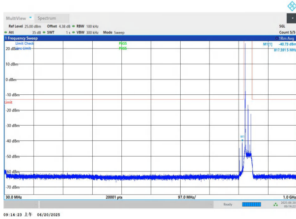
NTNV-n26(824-849)-PC3-15-20-M-DFT-QPSK-Edge_1RB_Left-3 0-1000-PASS
