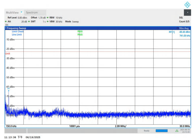
NTNV-n26(824-849)-PC3-15-10-L-DFT-BPSK-Edge_1RB_Left-0.1 5-30-PASS
