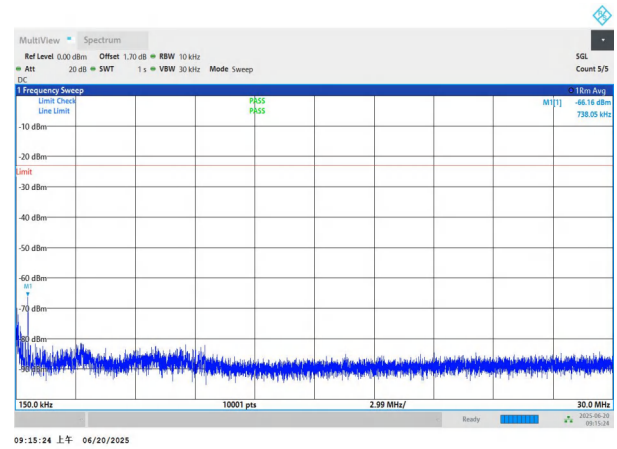
NTNV-n26(824-849)-PC3-15-20-H-DFT-BPSK-Edge_1RB_Left-0. 15-30-PASS
