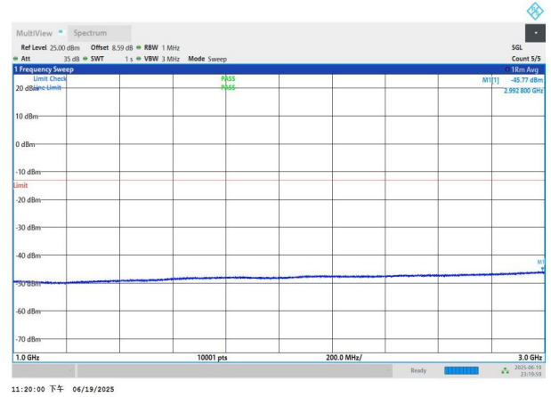
NTNV-n26(824-849)-PC3-15-10-H-DFT-BPSK-Edge_1RB_Left-1000-3000-PASS
