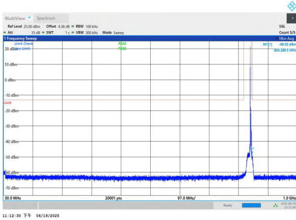
NTNV-n26(824-849)-PC3-15-5-H-DFT-QPSK-Edge_1RB_Left-30 -1000-PASS
