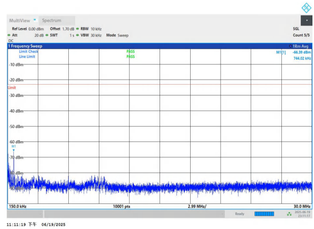
NTNV-n26(824-849)-PC3-15-5-H-DFT-BPSK-Edge_1RB_Left-0.1 5-30-PASS
