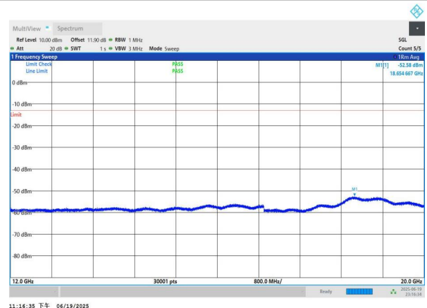
NTNV-n26(824-849)-PC3-15-10-M-DFT-BPSK-Edge_1RB_Left-12 000-20000-PASS
