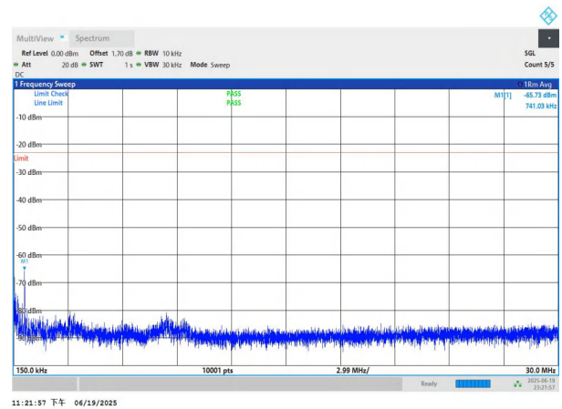
NTNV-n26(824-849)-PC3-15-15-L-DFT-BPSK-Edge_1RB_Left-0.1 5-30-PASS
