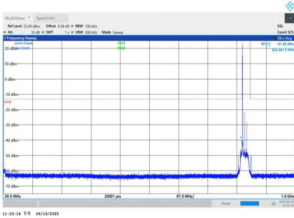
NTNV-n26(824-849)-PC3-15-15-L-DFT-QPSK-Edge_1RB_Left-3 0-1000-PASS
