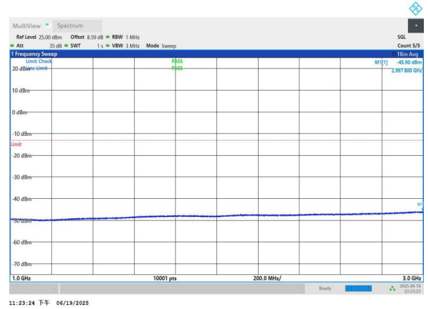
NTNV-n26(824-849)-PC3-15-15-L-DFT-QPSK-Edge_1RB_Left-10 00-3000-PASS
