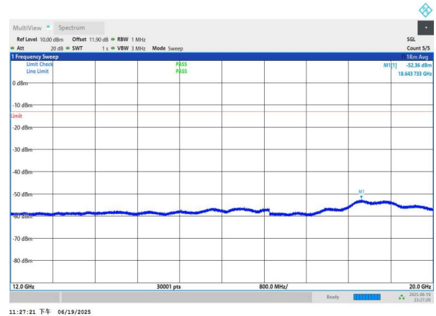
NTNV-n26(824-849)-PC3-15-15-H-DFT-BPSK-Edge_1RB_Left-12000-20000-PASS
