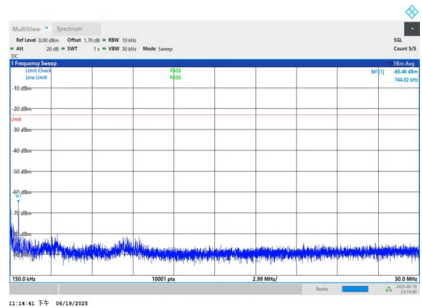
NTNV-n26(824-849)-PC3-15-10-L-DFT-QPSK-Edge_1RB_Left-0.1 5-30-PASS
