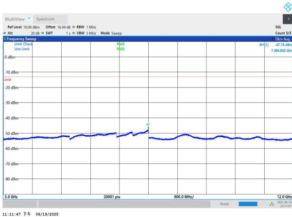
NTNV-n26(824-849)-PC3-15-5-H-DFT-BPSK-Edge_1RB_Left-30 00-12000-PASS
