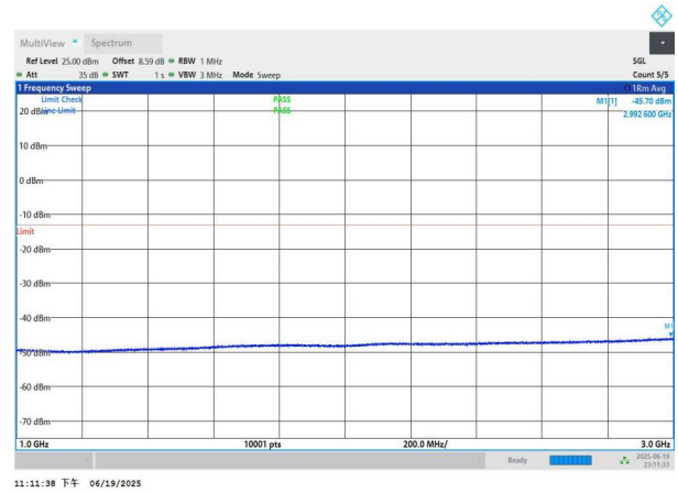
NTNV-n26(824-849)-PC3-15-5-H-DFT-BPSK-Edge_1RB_Left-100 0-3000-PASS
