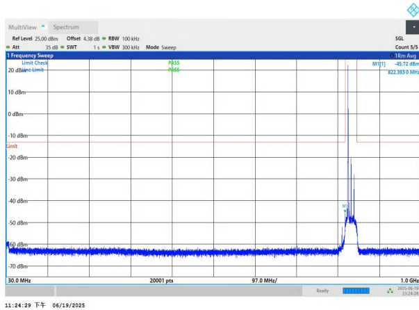
NTNV-n26(824-849)-PC3-15-15-M-DFT-BPSK-Edge_1RB_Left-3 0-1000-PASS
