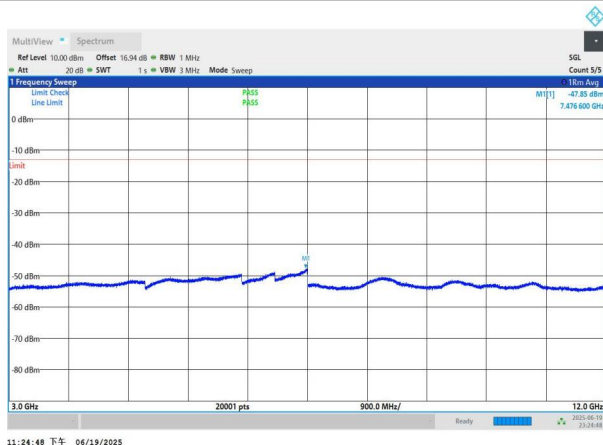
NTNV-n26(824-849)-PC3-15-15-M-DFT-BPSK-Edge_1RB_Left-3 000-12000-PASS
