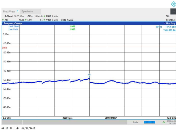
NTNV-n26(824-849)-PC3-15-20-H-DFT-BPSK-Edge_1RB_Left-3 000-12000-PASS
