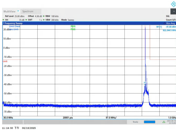
NTNV-n26(824-849)-PC3-15-10-L-DFT-QPSK-Edge_1RB_Left-3 0-1000-PASS
