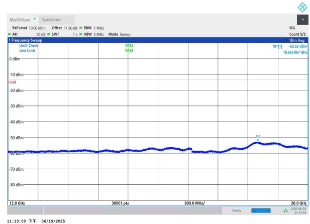
NTNV-n26(824-849)-PC3-15-5-H-DFT-QPSK-Edge_1RB_Left-120 00-20000-PASS
