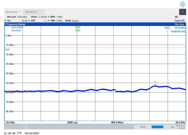
NTNV-n26(824-849)-PC3-15-15-L-DFT-QPSK-Edge_1RB_Left-12 000-20000-PASS
