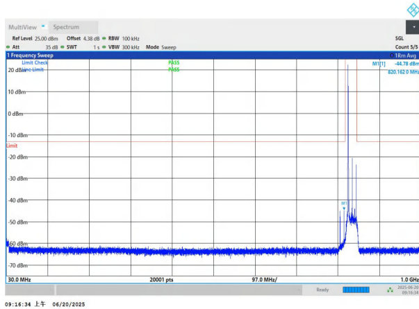
NTNV-n26(824-849)-PC3-15-20-H-DFT-QPSK-Edge_1RB_Left-3.0-1000-PASS
