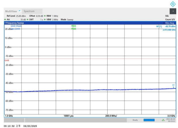
NTNV-n26(824-849)-PC3-15-20-L-DFT-BPSK-Edge_1RB_Left-10 00-3000-PASS
