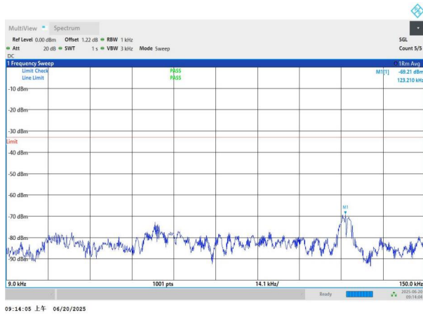
NTNV-n26(824-849)-PC3-15-20-M-DFT-QPSK-Edge_1RB_Left-0 .009-0.15-PASS
