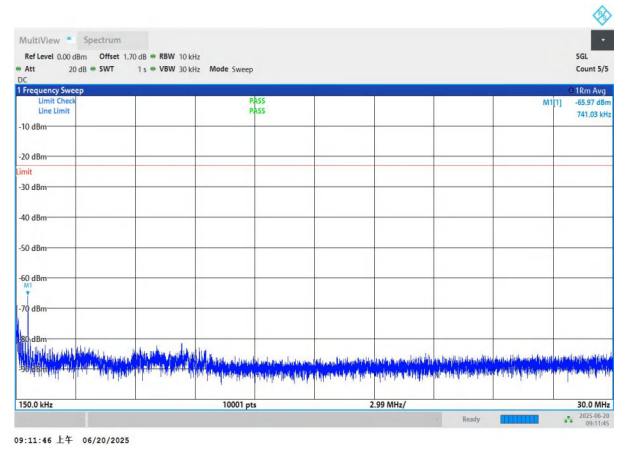
NTNV-n26(824-849)-PC3-15-20-L-DFT-QPSK-Edge_1RB_Left-0.1 5-30-PASS
