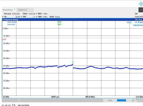
NTNV-n26(824-849)-PC3-15-10-L-DFT-QPSK-Edge_1RB_Left-3 000-12000-PASS
