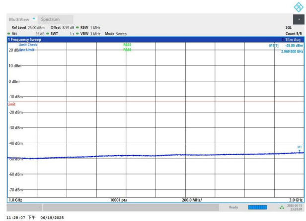
NTNV-n26(824-849)-PC3-15-15-H-DFT-QPSK-Edge_1RB_Left-10 00-3000-PASS
