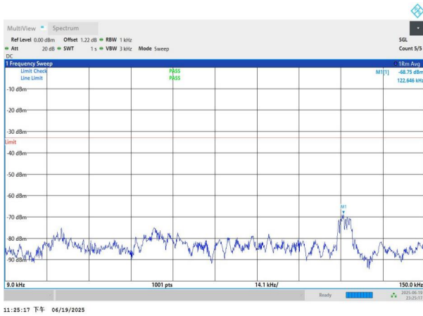
NTNV-n26(824-849)-PC3-15-15-M-DFT-QPSK-Edge_1RB_Left-0 .009-0.15-PASS
