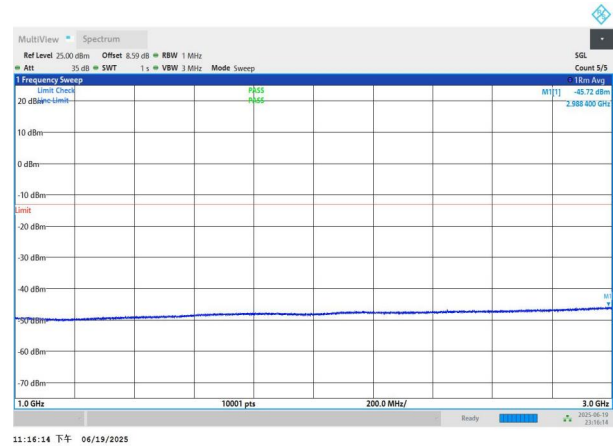
NTNV-n26(824-849)-PC3-15-10-M-DFT-BPSK-Edge_1RB_Left-10 00-3000-PASS
