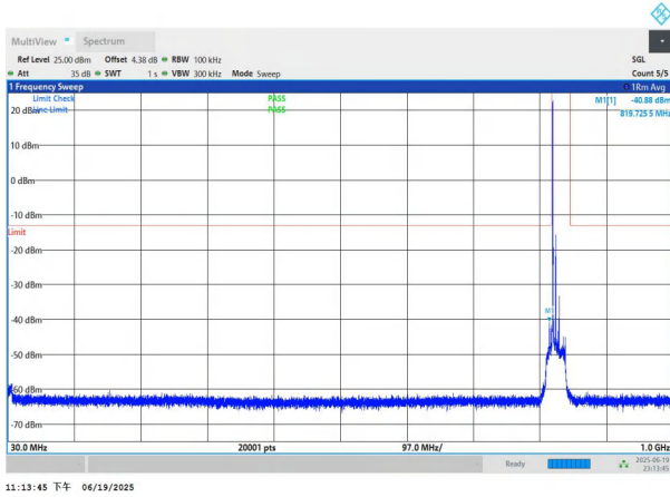
NTNV-n26(824-849)-PC3-15-10-L-DFT-BPSK-Edge_1RB_Left-3 0-1000-PASS
