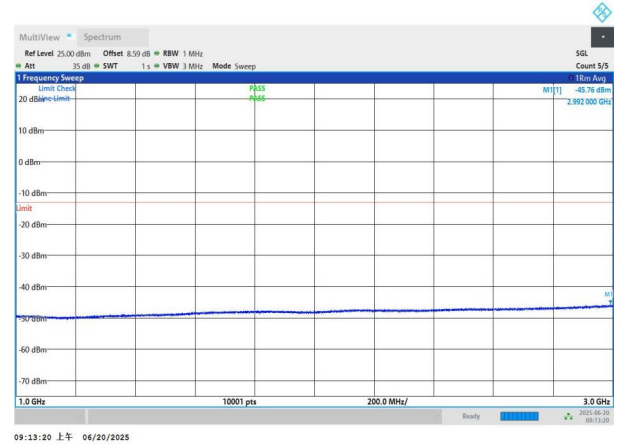
NTNV-n26(824-849)-PC3-15-20-M-DFT-BPSK-Edge_1RB_Left-10 00-3000-PASS
