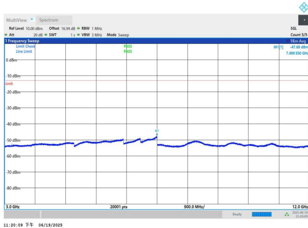
NTNV-n26(824-849)-PC3-15-10-H-DFT-BPSK-Edge_1RB_Left-3000-12000-PASS
