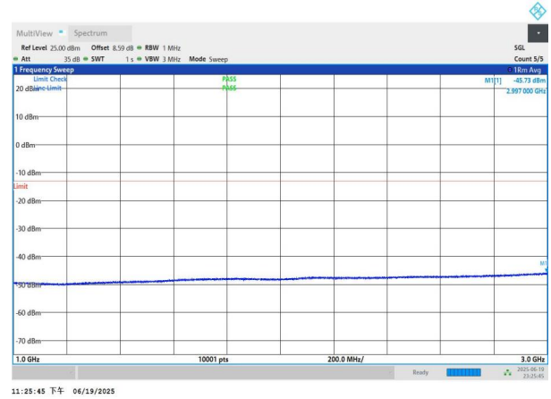
NTNV-n26(824-849)-PC3-15-15-M-DFT-QPSK-Edge_1RB_Left-10 00-3000-PASS
