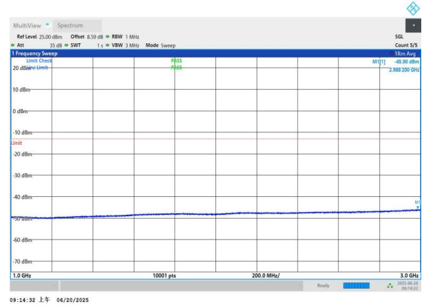
NTNV-n26(824-849)-PC3-15-20-M-DFT-QPSK-Edge_1RB_Left-10 00-3000-PASS
