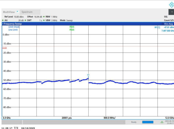
NTNV-n26(824-849)-PC3-15-15-H-DFT-QPSK-Edge_1RB_Left-3 000-12000-PASS
