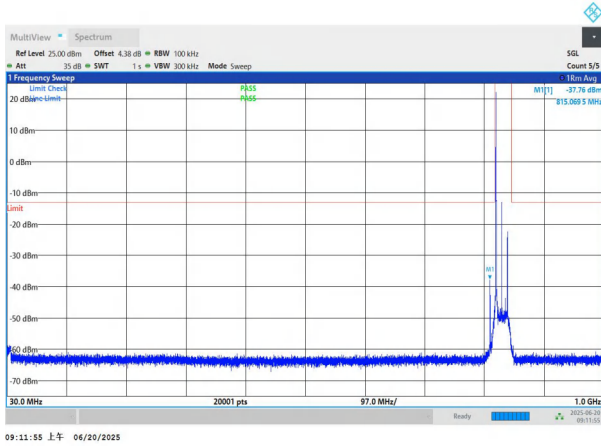
NTNV-n26(824-849)-PC3-15-20-L-DFT-QPSK-Edge_1RB_Left-3 0-1000-PASS
