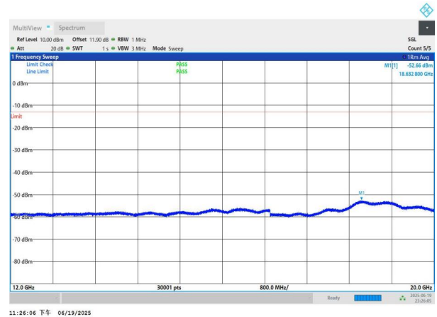
NTNV-n26(824-849)-PC3-15-15-M-DFT-QPSK-Edge_1RB_Left-12 000-20000-PASS
