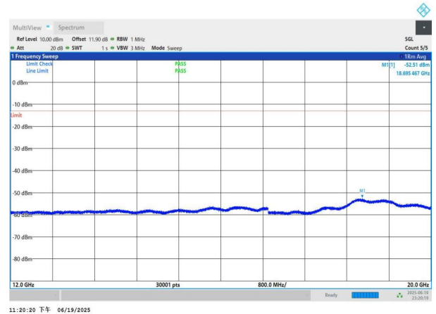
NTNV-n26(824-849)-PC3-15-10-H-DFT-BPSK-Edge_1RB_Left-12000-20000-PASS
