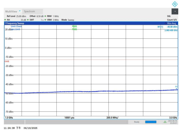
NTNV-n26(824-849)-PC3-15-15-M-DFT-BPSK-Edge_1RB_Left-10 00-3000-PASS
