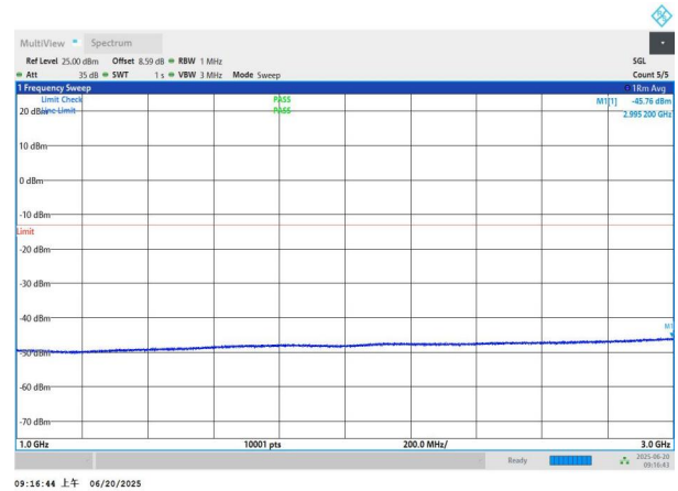
NTNV-n26(824-849)-PC3-15-20-H-DFT-QPSK-Edge_1RB_Left-10.00-3000-PASS
