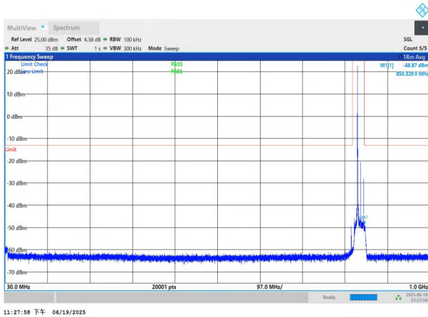
NTNV-n26(824-849)-PC3-15-15-H-DFT-QPSK-Edge_1RB_Left-3 0-1000-PASS
