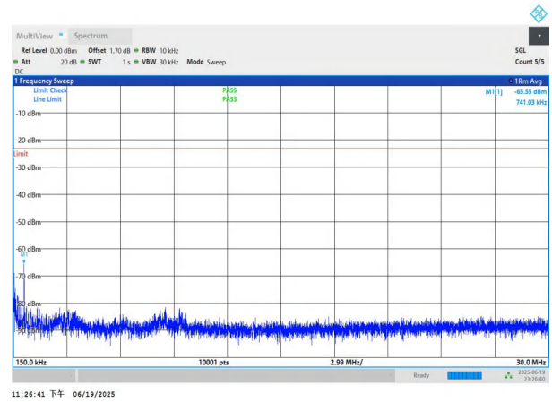
NTNV-n26(824-849)-PC3-15-15-H-DFT-BPSK-Edge_1RB_Left-0.15-30-PASS
