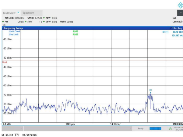
NTNV-n26(824-849)-PC3-15-15-L-DFT-BPSK-Edge_1RB_Left-0. 009-0.15-PASS
