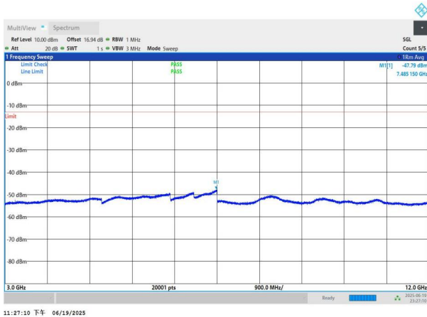
NTNV-n26(824-849)-PC3-15-15-H-DFT-BPSK-Edge_1RB_Left-3000-12000-PASS
