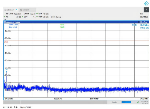
NTNV-n26(824-849)-PC3-15-20-H-DFT-QPSK-Edge_1RB_Left-0.15-30-PASS
