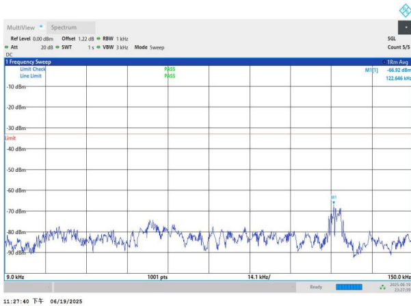
NTNV-n26(824-849)-PC3-15-15-H-DFT-QPSK-Edge_1RB_Left-0 .009-0.15-PASS
