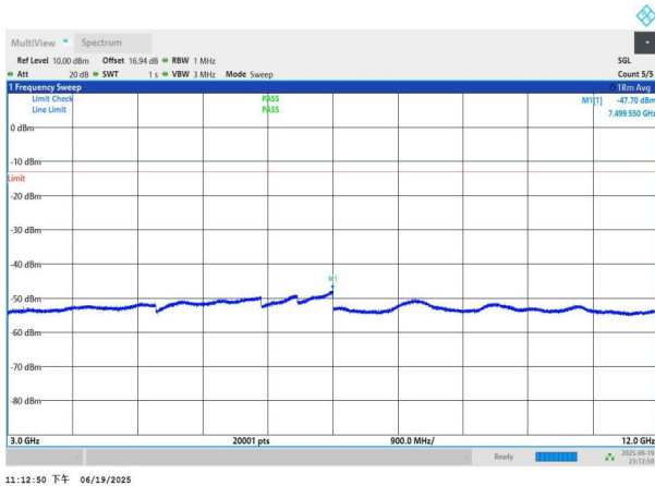
NTNV-n26(824-849)-PC3-15-5-H-DFT-QPSK-Edge_1RB_Left-30 00-12000-PASS
