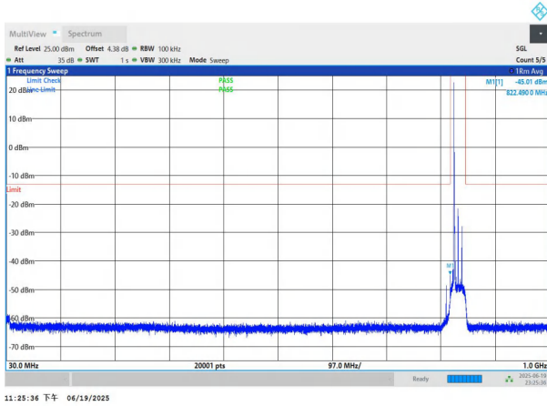
NTNV-n26(824-849)-PC3-15-15-M-DFT-QPSK-Edge_1RB_Left-3 0-1000-PASS
