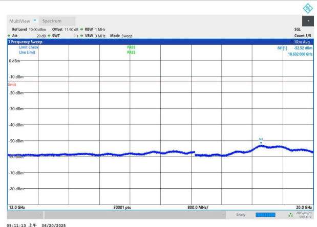
NTNV-n26(824-849)-PC3-15-20-L-DFT-BPSK-Edge_1RB_Left-12 000-20000-PASS
