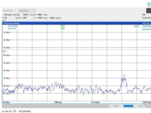
NTNV-n26(824-849)-PC3-15-15-M-DFT-BPSK-Edge_1RB_Left-0 .009-0.15-PASS
