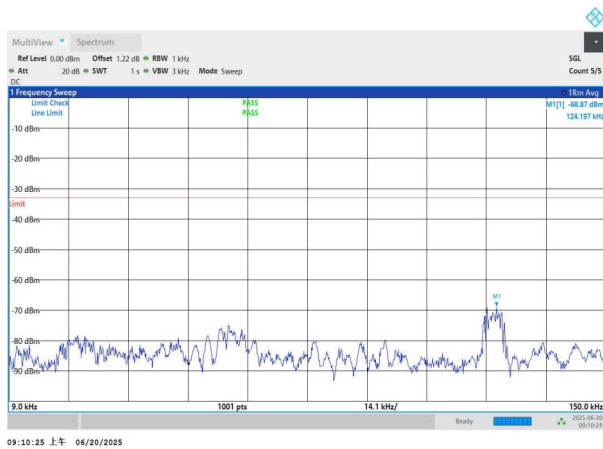
NTNV-n26(824-849)-PC3-15-20-L-DFT-BPSK-Edge_1RB_Left-0. 009-0.15-PASS
