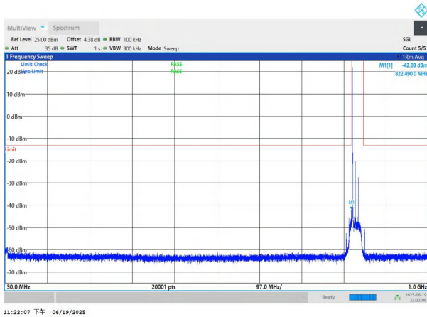
NTNV-n26(824-849)-PC3-15-15-L-DFT-BPSK-Edge_1RB_Left-3 0-1000-PASS
