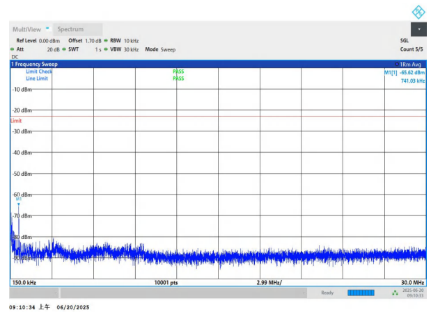
NTNV-n26(824-849)-PC3-15-20-L-DFT-BPSK-Edge_1RB_Left-0.1 5-30-PASS
