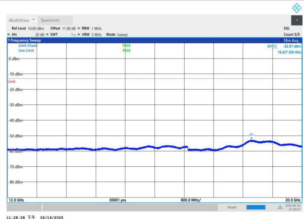
NTNV-n26(824-849)-PC3-15-15-H-DFT-QPSK-Edge_1RB_Left-12 000-20000-PASS
