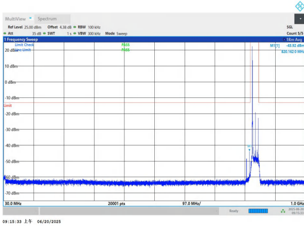
NTNV-n26(824-849)-PC3-15-20-H-DFT-BPSK-Edge_1RB_Left-3 0-1000-PASS
