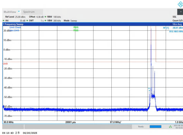
NTNV-n26(824-849)-PC3-15-20-L-DFT-BPSK-Edge_1RB_Left-3 0-1000-PASS
