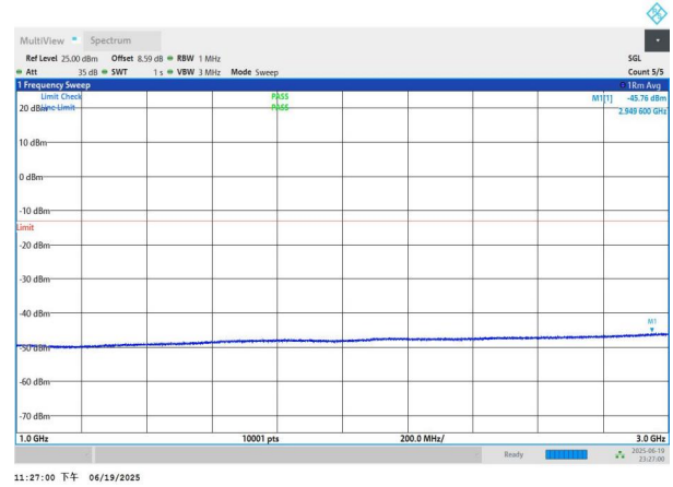
NTNV-n26(824-849)-PC3-15-15-H-DFT-BPSK-Edge_1RB_Left-1000-3000-PASS
