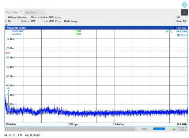
NTNV-n26(824-849)-PC3-15-20-M-DFT-BPSK-Edge_1RB_Left-0. 15-30-PASS
