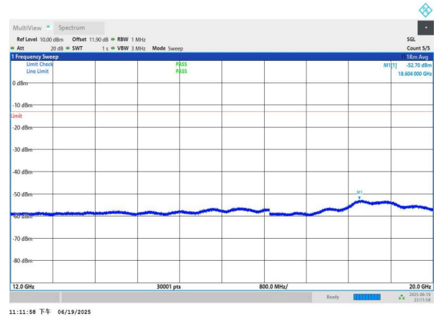
NTNV-n26(824-849)-PC3-15-5-H-DFT-BPSK-Edge_1RB_Left-120 00-20000-PASS
