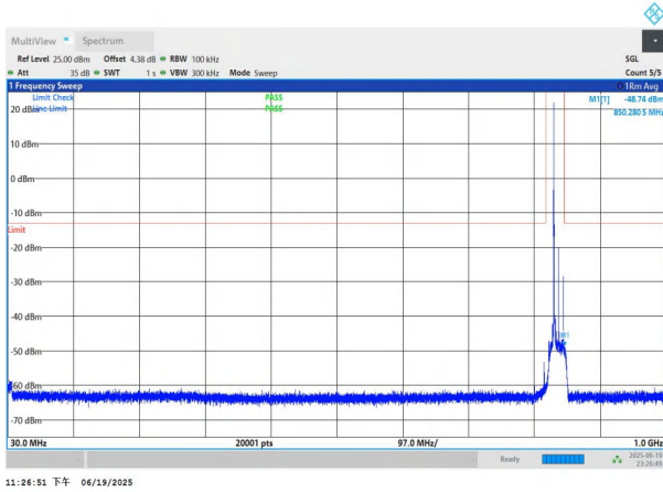
NTNV-n26(824-849)-PC3-15-15-H-DFT-BPSK-Edge_1RB_Left-30-1000-PASS
