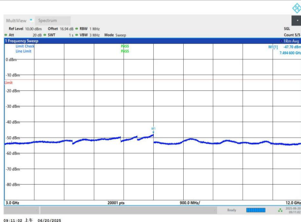
NTNV-n26(824-849)-PC3-15-20-L-DFT-BPSK-Edge_1RB_Left-3 000-12000-PASS
