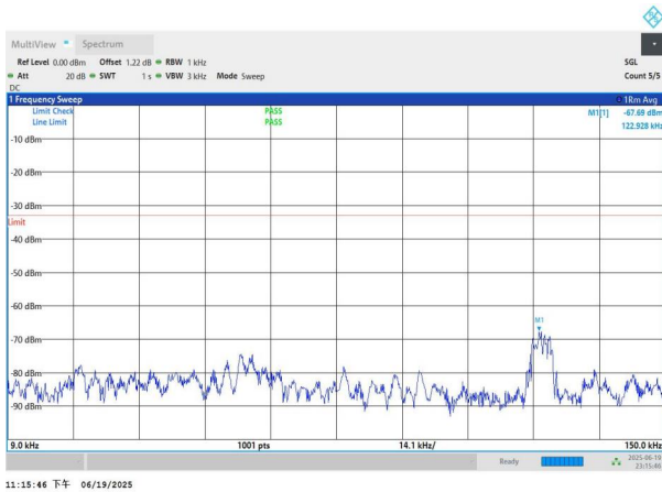
NTNV-n26(824-849)-PC3-15-10-M-DFT-BPSK-Edge_1RB_Left-0 .009-0.15-PASS
