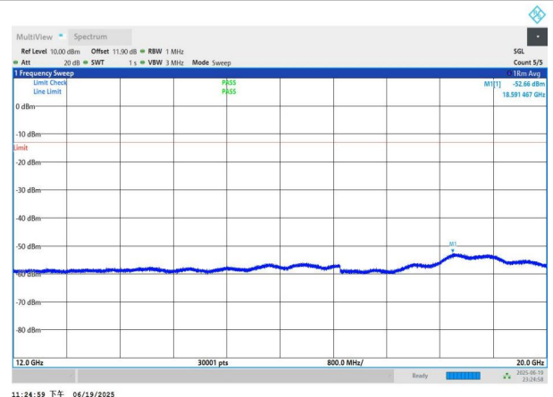
NTNV-n26(824-849)-PC3-15-15-M-DFT-BPSK-Edge_1RB_Left-12 000-20000-PASS
