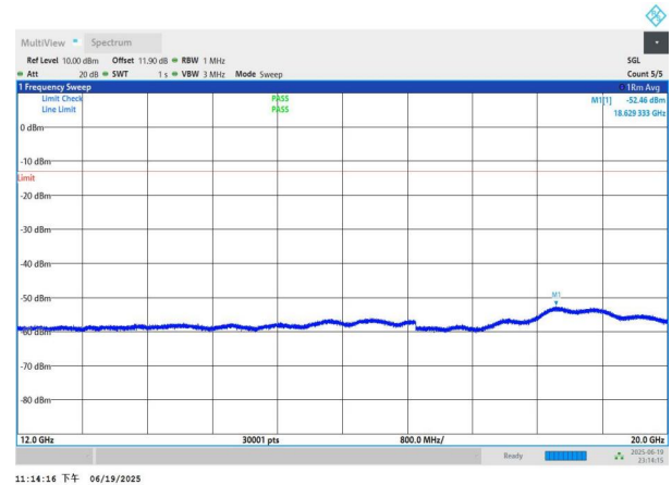
NTNV-n26(824-849)-PC3-15-10-L-DFT-BPSK-Edge_1RB_Left-12 000-20000-PASS
