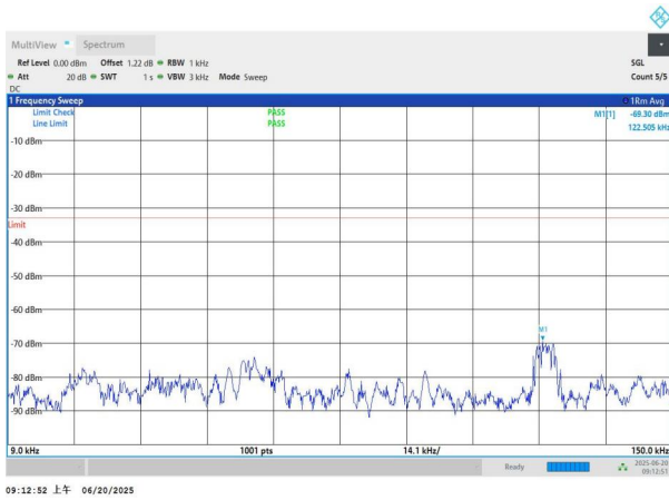
NTNV-n26(824-849)-PC3-15-20-M-DFT-BPSK-Edge_1RB_Left-0 .009-0.15-PASS
