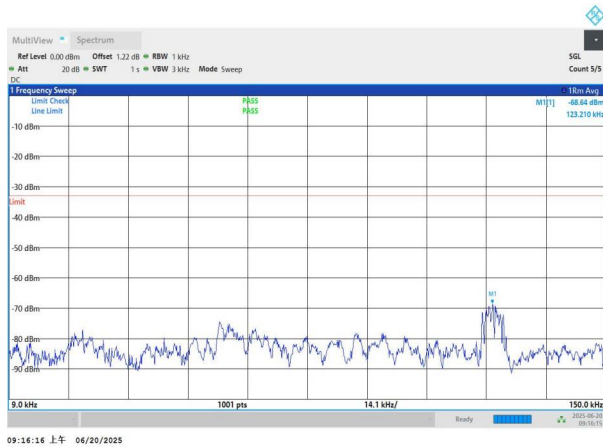
NTNV-n26(824-849)-PC3-15-20-H-DFT-QPSK-Edge_1RB_Left-0.009-0.15-PASS
