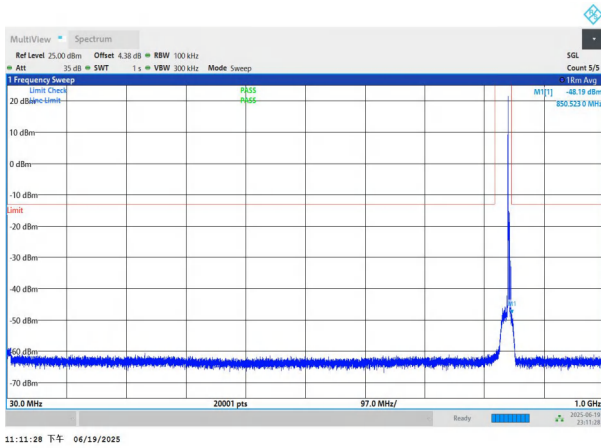
NTNV-n26(824-849)-PC3-15-5-H-DFT-BPSK-Edge_1RB_Left-30- 1000-PASS
