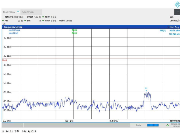
NTNV-n26(824-849)-PC3-15-15-H-DFT-BPSK-Edge_1RB_Left-0.009-0.15-PASS
