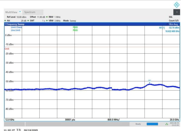
NTNV-n26(824-849)-PC3-15-15-L-DFT-BPSK-Edge_1RB_Left-12 000-20000-PASS
