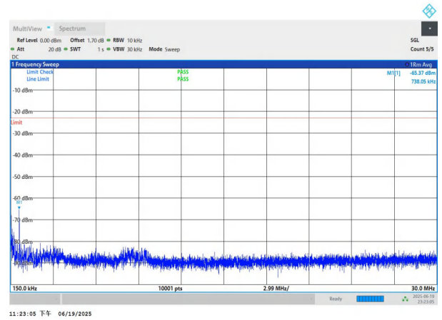
NTNV-n26(824-849)-PC3-15-15-L-DFT-QPSK-Edge_1RB_Left-0.1 5-30-PASS
