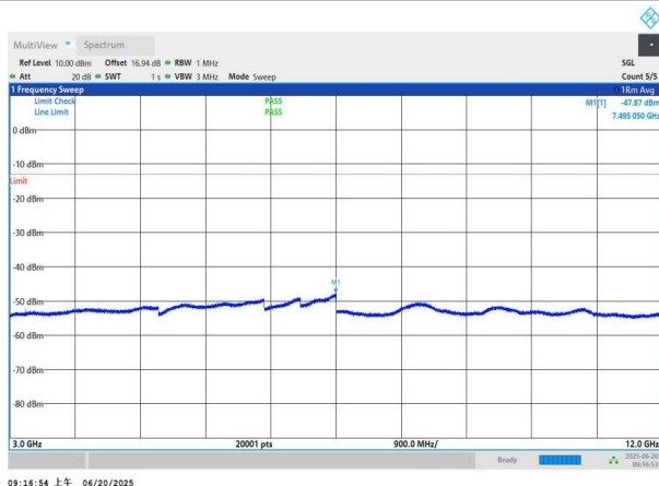
NTNV-n26(824-849)-PC3-15-20-H-DFT-QPSK-Edge_1RB_Left-3.000-12000-PASS
