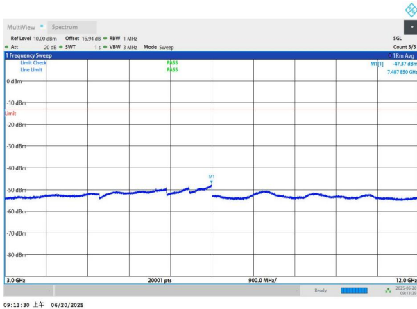
NTNV-n26(824-849)-PC3-15-20-M-DFT-BPSK-Edge_1RB_Left-3 000-12000-PASS
