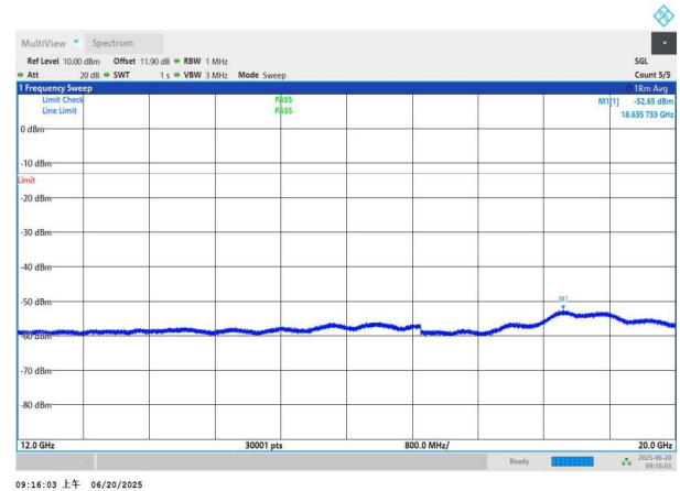
NTNV-n26(824-849)-PC3-15-20-H-DFT-BPSK-Edge_1RB_Left-12 000-20000-PASS
