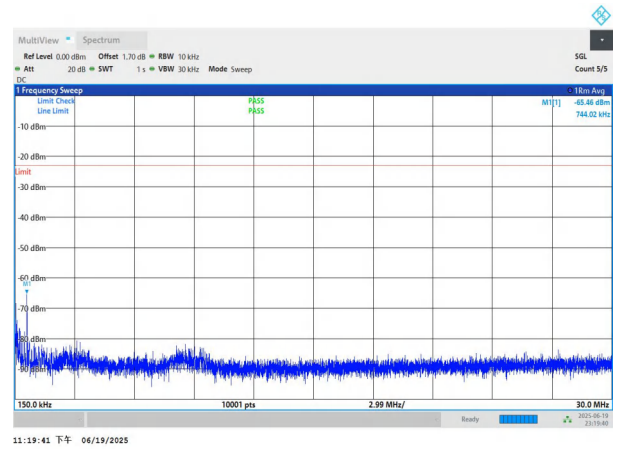
NTNV-n26(824-849)-PC3-15-10-H-DFT-BPSK-Edge_1RB_Left-0.15-30-PASS
