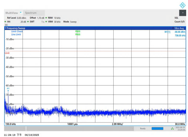
NTNV-n26(824-849)-PC3-15-15-M-DFT-BPSK-Edge_1RB_Left-0. 15-30-PASS
