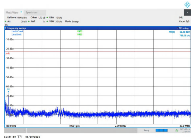
NTNV-n26(824-849)-PC3-15-15-H-DFT-QPSK-Edge_1RB_Left-0. 15-30-PASS
