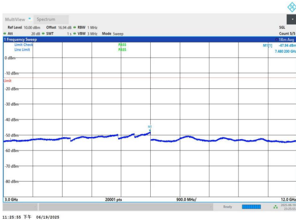
NTNV-n26(824-849)-PC3-15-15-M-DFT-QPSK-Edge_1RB_Left-3 000-12000-PASS
