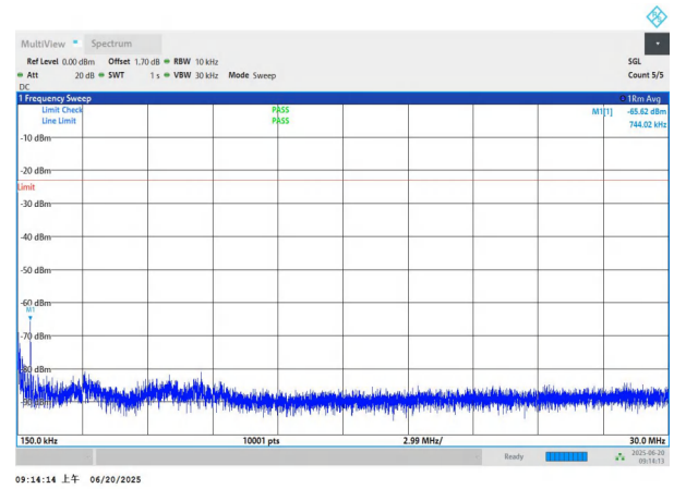
NTNV-n26(824-849)-PC3-15-20-M-DFT-QPSK-Edge_1RB_Left-0. 15-30-PASS
