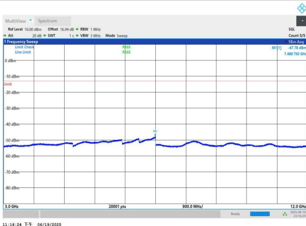
NTNV-n26(824-849)-PC3-15-10-M-DFT-BPSK-Edge_1RB_Left-3 000-12000-PASS
