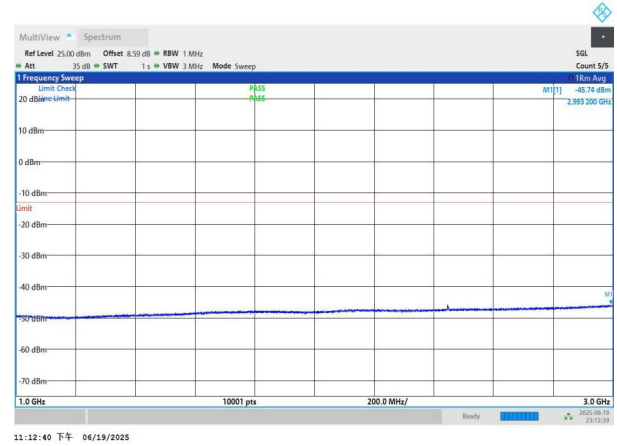
NTNV-n26(824-849)-PC3-15-5-H-DFT-QPSK-Edge_1RB_Left-100 0-3000-PASS
