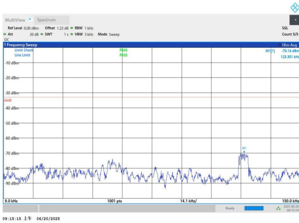
NTNV-n26(824-849)-PC3-15-20-H-DFT-BPSK-Edge_1RB_Left-0. 009-0.15-PASS
