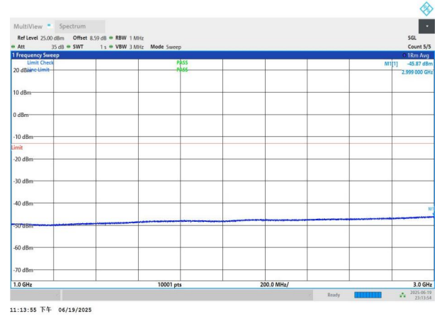
NTNV-n26(824-849)-PC3-15-10-L-DFT-BPSK-Edge_1RB_Left-10 00-3000-PASS
