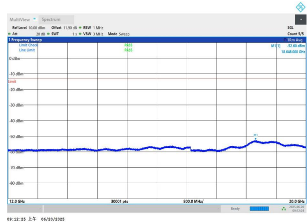
NTNV-n26(824-849)-PC3-15-20-L-DFT-QPSK-Edge_1RB_Left-12 000-20000-PASS
