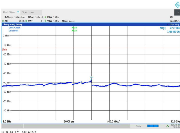
NTNV-n26(824-849)-PC3-15-15-L-DFT-BPSK-Edge_1RB_Left-3 000-12000-PASS
