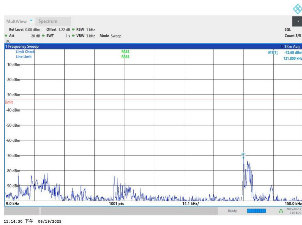
NTNV-n26(824-849)-PC3-15-10-L-DFT-QPSK-Edge_1RB_Left-0. 009-0.15-PASS
