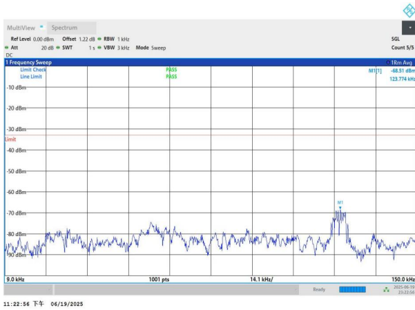
NTNV-n26(824-849)-PC3-15-15-L-DFT-QPSK-Edge_1RB_Left-0. 009-0.15-PASS
