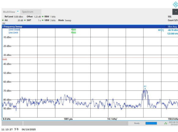
NTNV-n26(824-849)-PC3-15-10-L-DFT-BPSK-Edge_1RB_Left-0. 009-0.15-PASS
