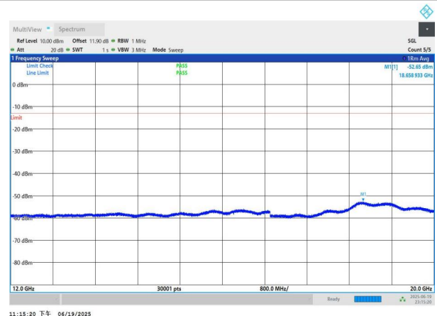
NTNV-n26(824-849)-PC3-15-10-L-DFT-QPSK-Edge_1RB_Left-12 000-20000-PASS
