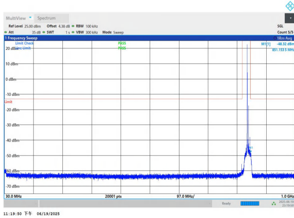
NTNV-n26(824-849)-PC3-15-10-H-DFT-BPSK-Edge_1RB_Left-30-1000-PASS
