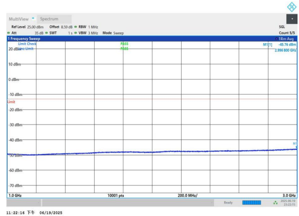
NTNV-n26(824-849)-PC3-15-15-L-DFT-BPSK-Edge_1RB_Left-10 00-3000-PASS
