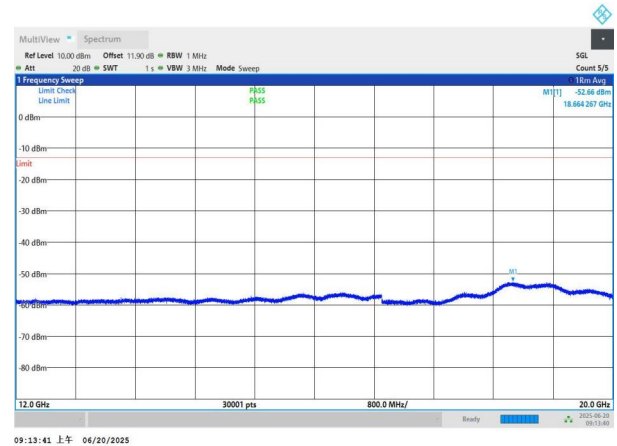
NTNV-n26(824-849)-PC3-15-20-M-DFT-BPSK-Edge_1RB_Left-12 000-20000-PASS
