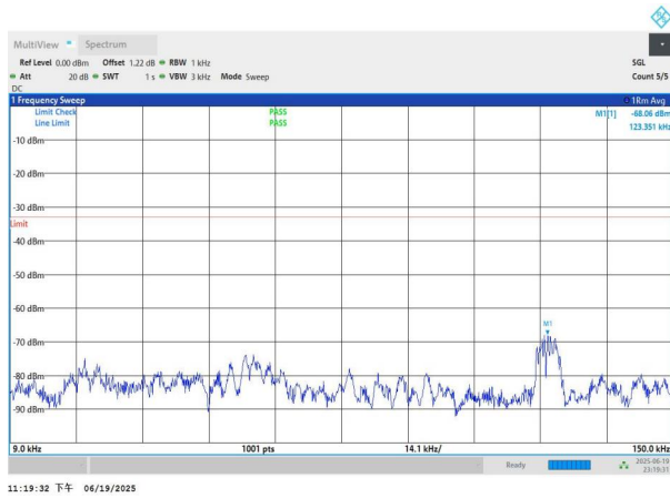
NTNV-n26(824-849)-PC3-15-10-H-DFT-BPSK-Edge_1RB_Left-0.009-0.15-PASS
