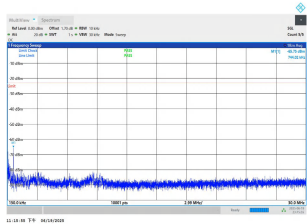
NTNV-n26(824-849)-PC3-15-10-M-DFT-BPSK-Edge_1RB_Left-0. 15-30-PASS
