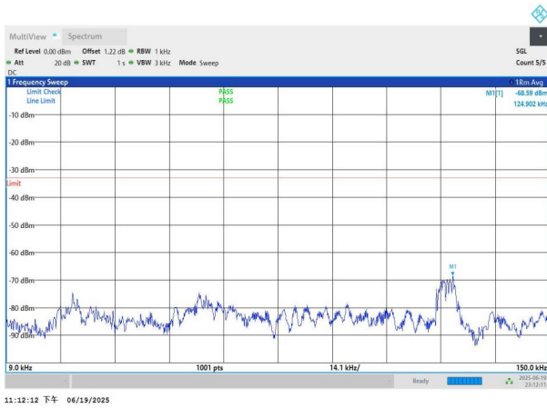
NTNV-n26(824-849)-PC3-15-5-H-DFT-QPSK-Edge_1RB_Left-0. 009-0.15-PASS
