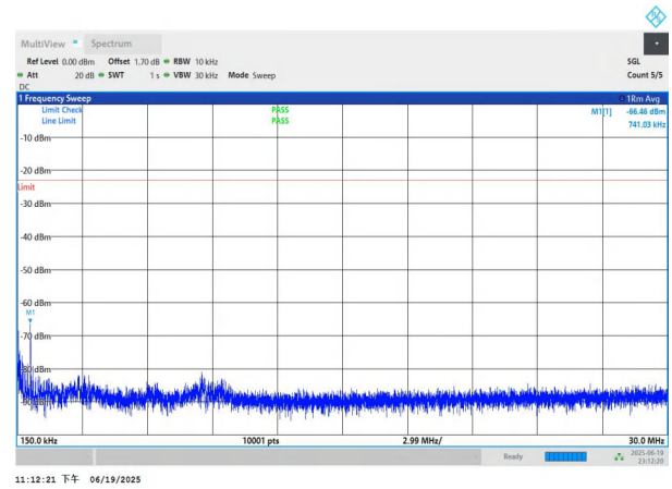
NTNV-n26(824-849)-PC3-15-5-H-DFT-QPSK-Edge_1RB_Left-0.1 5-30-PASS
