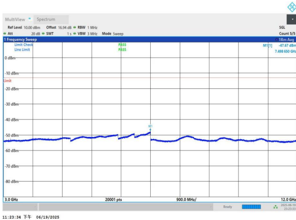
NTNV-n26(824-849)-PC3-15-15-L-DFT-QPSK-Edge_1RB_Left-3 000-12000-PASS
