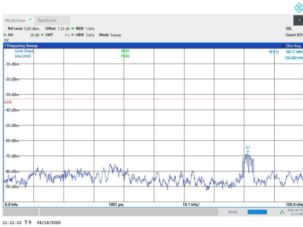
NTNV-n26(824-849)-PC3-15-5-H-DFT-BPSK-Edge_1RB_Left-0.0 09-0.15-PASS
