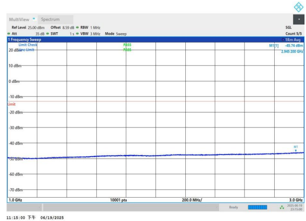
NTNV-n26(824-849)-PC3-15-10-L-DFT-QPSK-Edge_1RB_Left-10 00-3000-PASS
