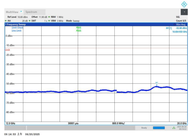
NTNV-n26(824-849)-PC3-15-20-M-DFT-QPSK-Edge_1RB_Left-12 000-20000-PASS
