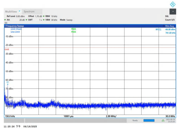
NTNV-n26(824-849)-PC3-15-15-M-DFT-QPSK-Edge_1RB_Left-0. 15-30-PASS
