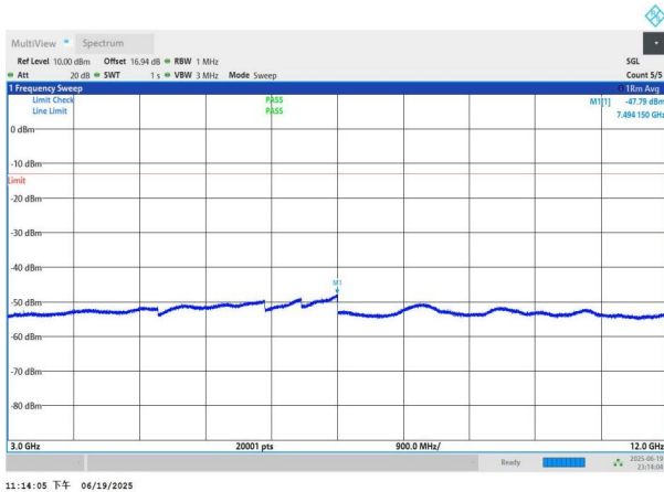
NTNV-n26(824-849)-PC3-15-10-L-DFT-BPSK-Edge_1RB_Left-3 000-12000-PASS
