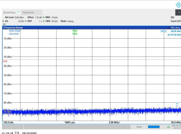
NTNV-n77(3450-3550)-PC3-30-50-M-DFT-QPSK-Edge_1RB_Left -0.15-30-PASS
