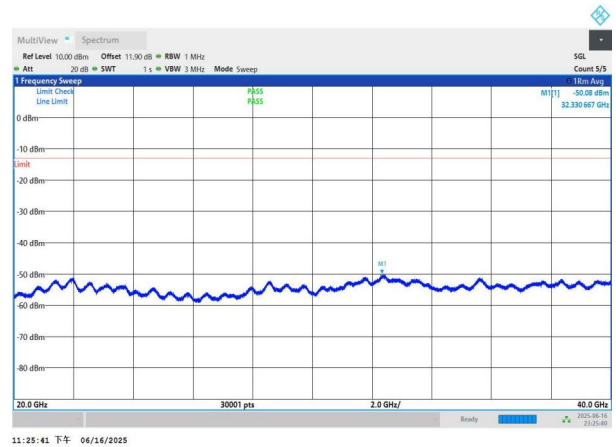
NTNV-n77(3450-3550)-PC3-30-60-L-DFT-QPSK-Edge_1RB_Left- 20000-40000-PASS
