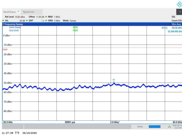
NTNV-n77(3450-3550)-PC3-30-60-M-DFT-BPSK-Edge_1RB_Left -20000-40000-PASS
