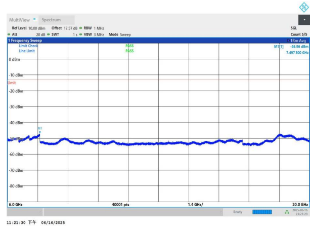
NTNV-n77(3450-3550)-PC3-30-50-H-DFT-BPSK-Edge_1RB_Left 6000-20000-PASS
