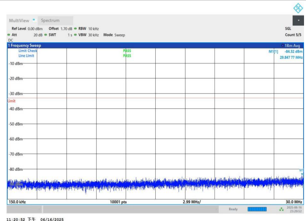
NTNV-n77(3450-3550)-PC3-30-50-H-DFT-BPSK-Edge_1RB_Left 0.15-30-PASS
