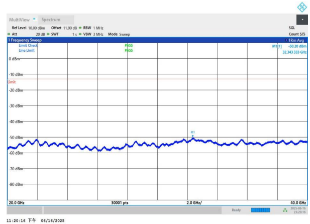
NTNV-n77(3450-3550)-PC3-30-50-M-DFT-QPSK-Edge_1RB_Left -20000-40000-PASS
