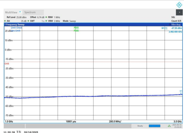
NTNV-n77(3450-3550)-PC3-30-60-M-DFT-BPSK-Edge_1RB_Left -1000-3000-PASS
