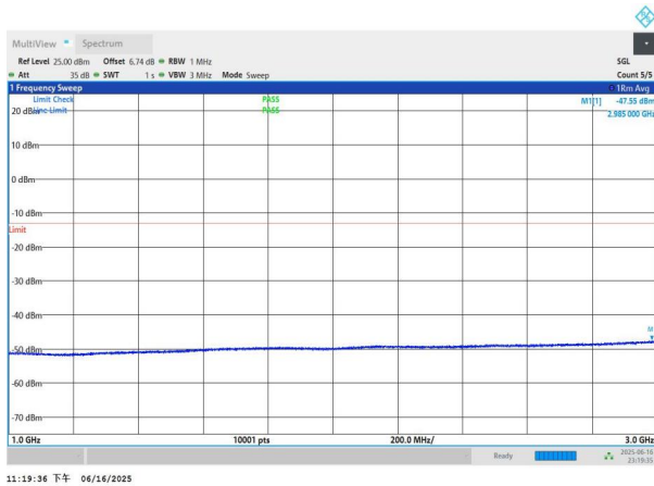
NTNV-n77(3450-3550)-PC3-30-50-M-DFT-QPSK-Edge_1RB_Left -1000-3000-PASS
