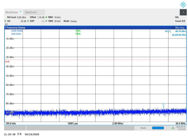
NTNV-n77(3450-3550)-PC3-30-60-L-DFT-BPSK-Edge_1RB_Left- 0.15-30-PASS
