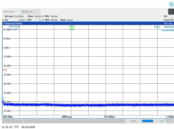
NTNV-n77(3450-3550)-PC3-30-50-H-DFT-BPSK-Edge_1RB_Left -30-1000-PASS
