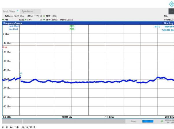
NTNV-n77(3450-3550)-PC3-30-50-H-DFT-QPSK-Edge_1RB_Left -6000-20000-PASS
