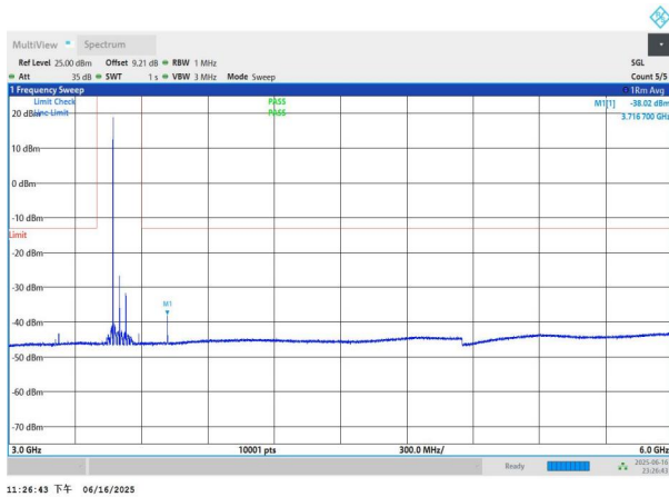
NTNV-n77(3450-3550)-PC3-30-60-M-DFT-BPSK-Edge_1RB_Left -3000-6000-PASS
