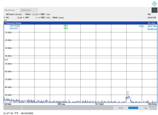
NTNV-n77(3450-3550)-PC3-30-60-M-DFT-QPSK-Edge_1RB_Left -0.009-0.15-PASS
