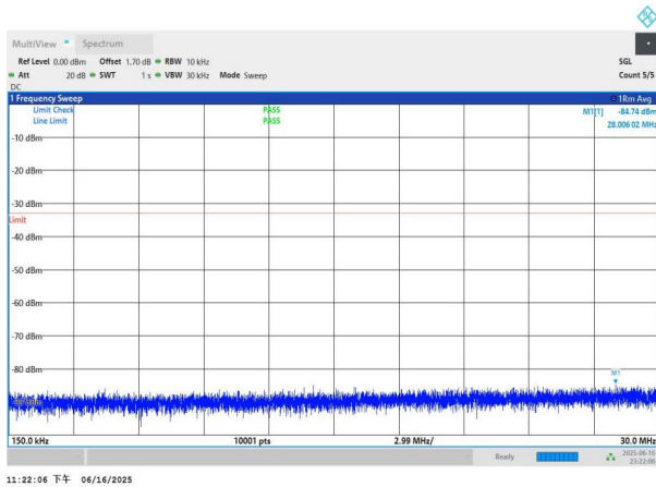
NTNV-n77(3450-3550)-PC3-30-50-H-DFT-QPSK-Edge_1RB_Left -0.15-30-PASS
