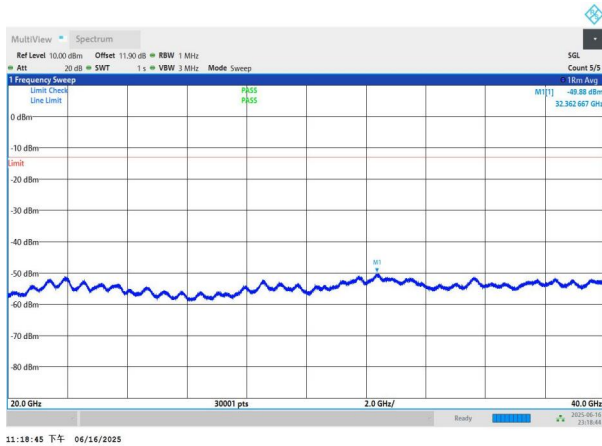
NTNV-n77(3450-3550)-PC3-30-50-M-DFT-BPSK-Edge_1RB_Left -20000-40000-PASS
