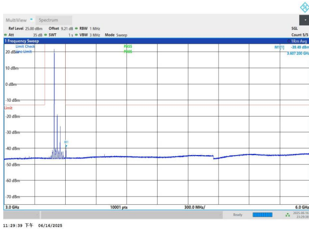
NTNV-n77(3450-3550)-PC3-30-60-H-DFT-BPSK-Edge_1RB_Left -3000-6000-PASS
