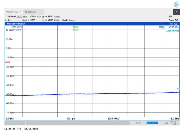
NTNV-n77(3450-3550)-PC3-30-60-H-DFT-BPSK-Edge_1RB_Left 1000-3000-PASS
