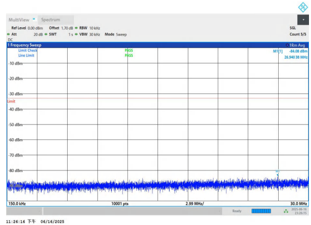
NTNV-n77(3450-3550)-PC3-30-60-M-DFT-BPSK-Edge_1RB_Left -0.15-30-PASS
