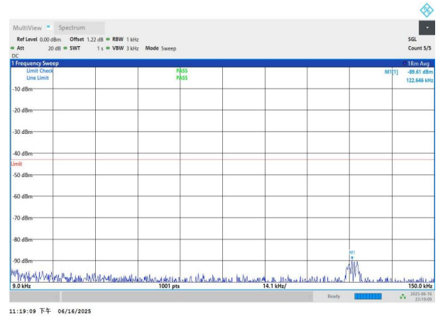
NTNV-n77(3450-3550)-PC3-30-50-M-DFT-QPSK-Edge_1RB_Left -0.009-0.15-PASS
