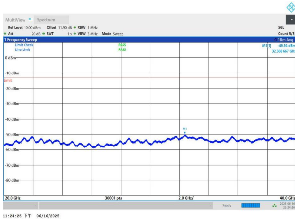
NTNV-n77(3450-3550)-PC3-30-60-L-DFT-BPSK-Edge_1RB_Left- 20000-40000-PASS
