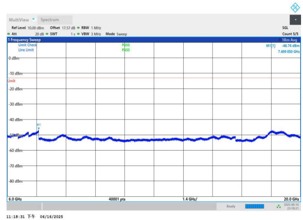
NTNV-n77(3450-3550)-PC3-30-50-M-DFT-BPSK-Edge_1RB_Left -6000-20000-PASS
