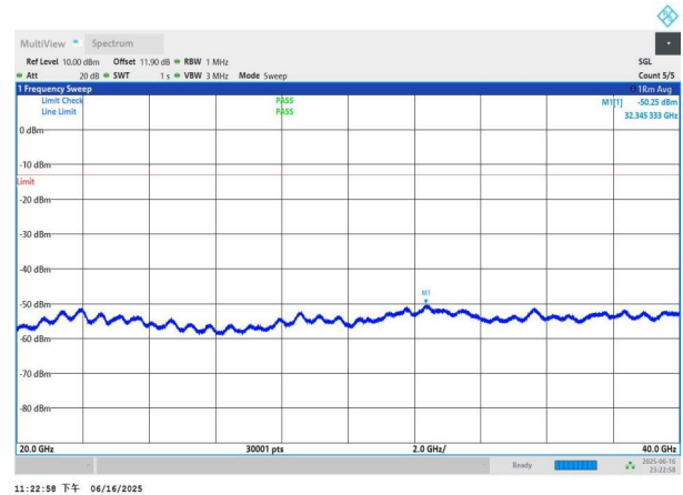
NTNV-n77(3450-3550)-PC3-30-50-H-DFT-QPSK-Edge_1RB_Left -20000-40000-PASS
