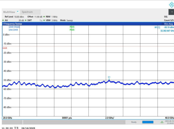
NTNV-n77(3450-3550)-PC3-30-60-H-DFT-BPSK-Edge_1RB_Left -20000-40000-PASS
