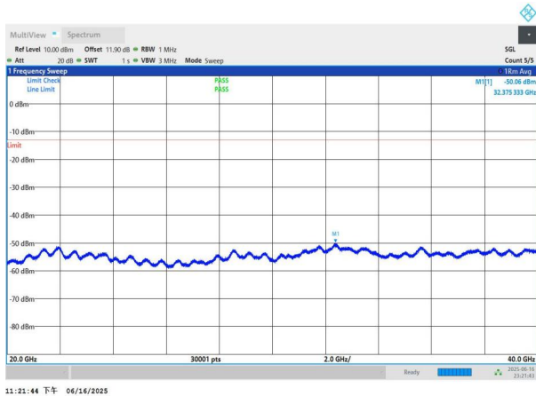
NTNV-n77(3450-3550)-PC3-30-50-H-DFT-BPSK-Edge_1RB_Left -20000-40000-PASS
