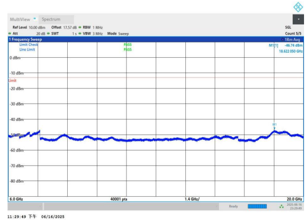
NTNV-n77(3450-3550)-PC3-30-60-H-DFT-BPSK-Edge_1RB_Left 6000-20000-PASS
