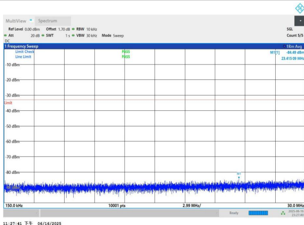
NTNV-n77(3450-3550)-PC3-30-60-M-DFT-QPSK-Edge_1RB_Left -0.15-30-PASS
