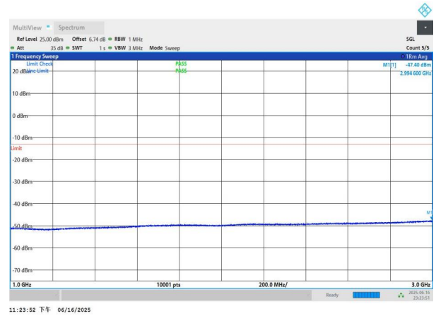
NTNV-n77(3450-3550)-PC3-30-60-L-DFT-BPSK-Edge_1RB_Left- 1000-3000-PASS
