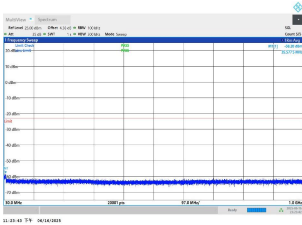
NTNV-n77(3450-3550)-PC3-30-60-L-DFT-BPSK-Edge_1RB_Left- 30-1000-PASS
