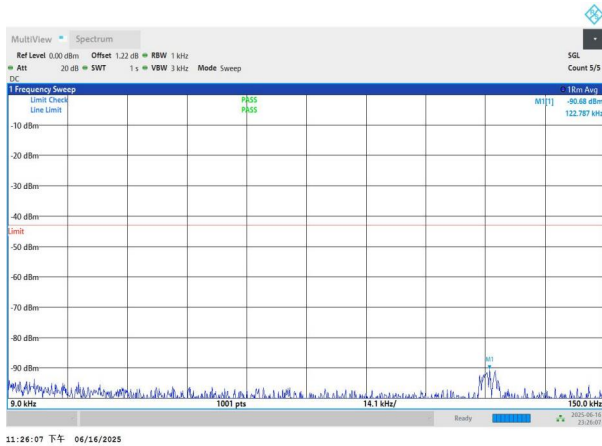
NTNV-n77(3450-3550)-PC3-30-60-M-DFT-BPSK-Edge_1RB_Left -0.009-0.15-PASS
