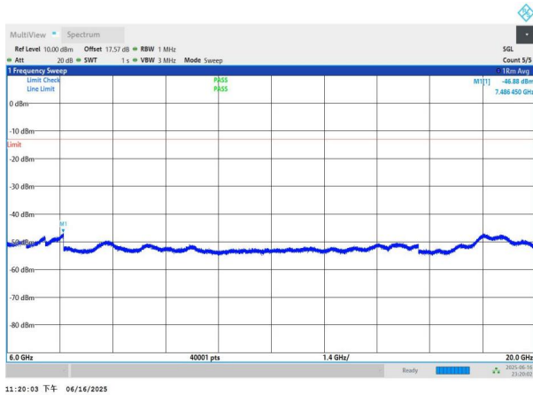
NTNV-n77(3450-3550)-PC3-30-50-M-DFT-QPSK-Edge_1RB_Left -6000-20000-PASS
