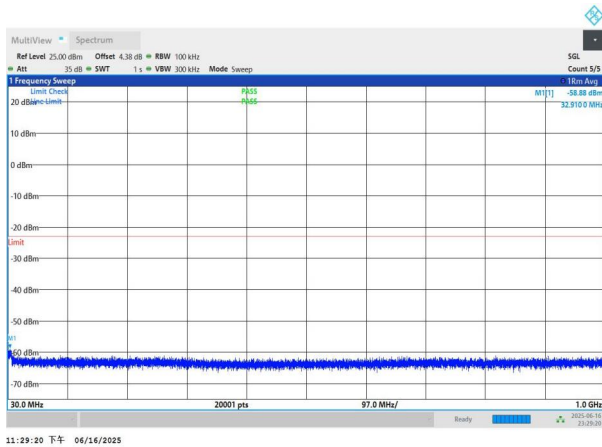
NTNV-n77(3450-3550)-PC3-30-60-H-DFT-BPSK-Edge_1RB_Left -30-1000-PASS
