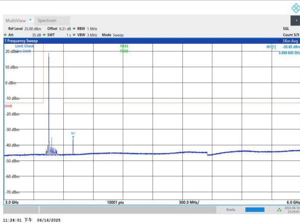
NTNV-n77(3450-3550)-PC3-30-60-L-DFT-BPSK-Edge_1RB_Left- 3000-6000-PASS
