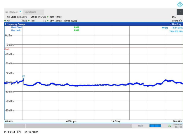
NTNV-n77(3450-3550)-PC3-30-60-M-DFT-BPSK-Edge_1RB_Left -6000-20000-PASS
