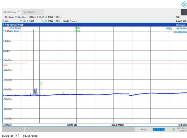
NTNV-n77(3450-3550)-PC3-30-50-H-DFT-BPSK-Edge_1RB_Left -3000-6000-PASS
