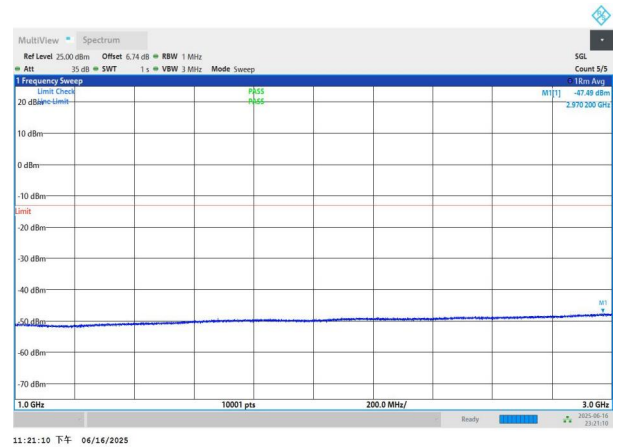
NTNV-n77(3450-3550)-PC3-30-50-H-DFT-BPSK-Edge_1RB_Left 1000-3000-PASS
