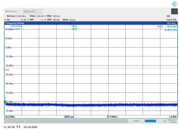
NTNV-n77(3450-3550)-PC3-30-60-L-DFT-QPSK-Edge_1RB_Left- 30-1000-PASS
