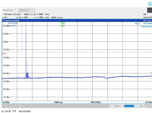
NTNV-n77(3450-3550)-PC3-30-50-M-DFT-BPSK-Edge_1RB_Left -3000-6000-PASS
