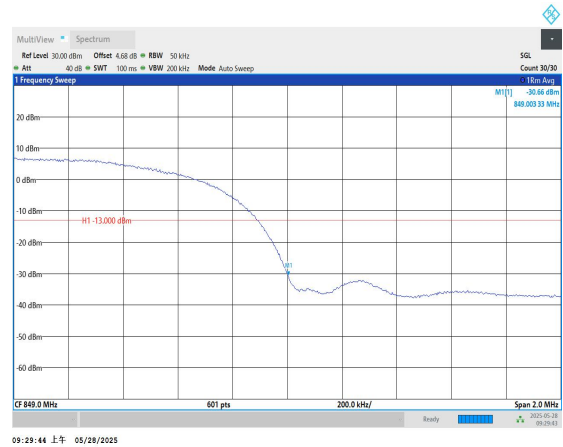
Band5-4233-PASS
