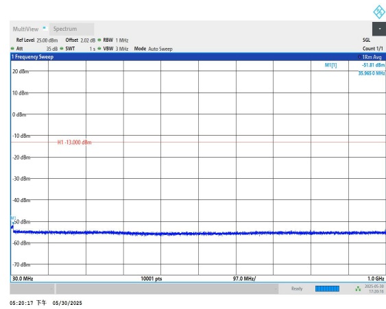
Band2-9400-30~1000MHz-PASS
