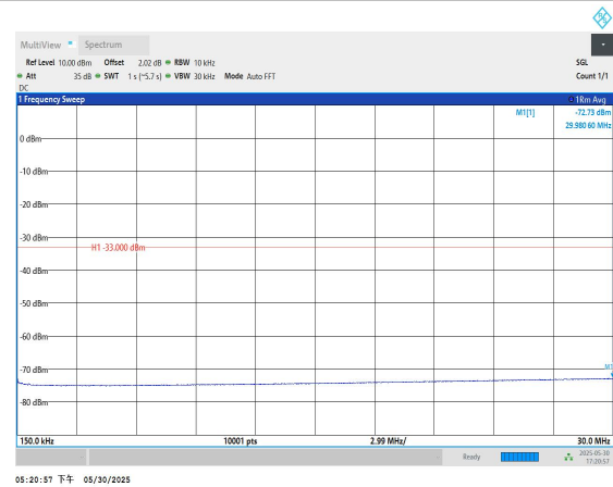
Band2-9538-0.15~30MHz-PASS
