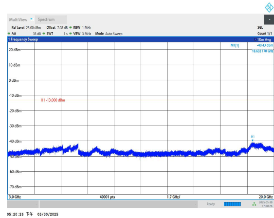
Band2-9400-3000~20000MHz-PASS
