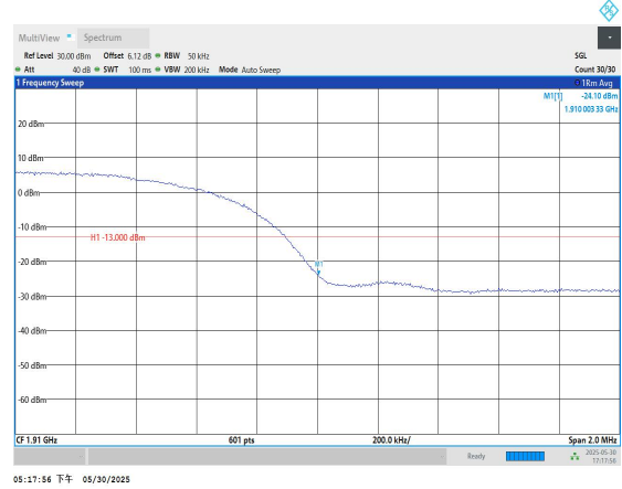
Band2-9538-PASS
