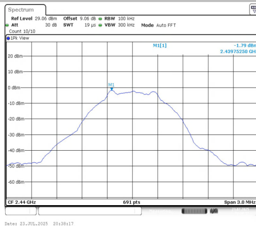
BLE_1M-Ant1-2440-0~Reference-PASS
