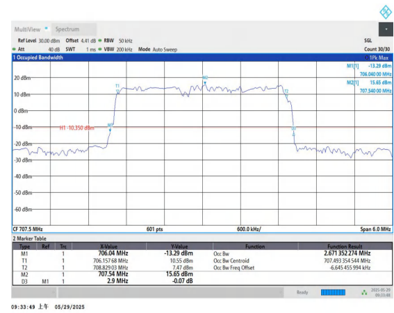
Band12-3MHz-QPSK-23095-15RB#0-PASS
