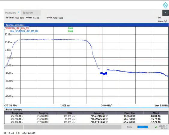
Band12-1.4MHz-QPSK-23173-6RB#0-PASS
