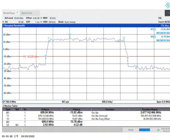
Band12-3MHz-QPSK-23025-15RB#0-PASS
