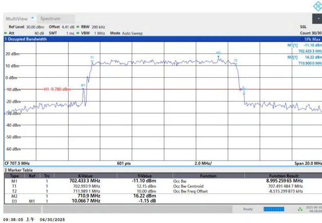
Band12-10MHz-16QAM-23095-50RB#0-PASS
