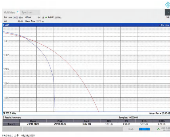
Band12-1.4MHz-16QAM-23095-1RB#0-PASS
