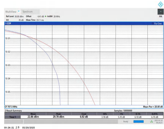
Band12-1.4MHz-16QAM-23095-6RB#0-PASS
