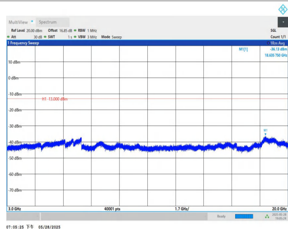
Band2-1.4MHz-QPSK-18607-1RB#0-3000~20000-PASS
