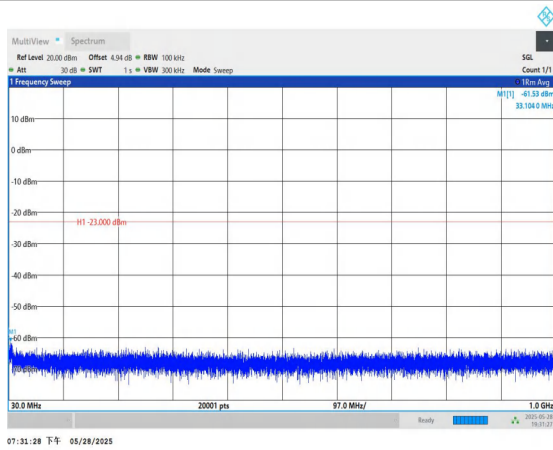
Band2-5MHz-QPSK-18625-1RB#0-30~1000-PASS
