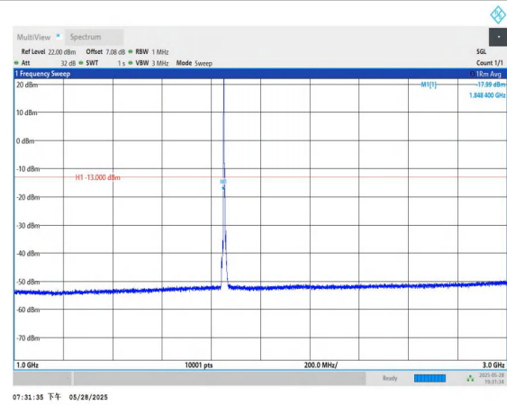
Band2-5MHz-QPSK-18625-1RB#0-1000~3000-PASS
