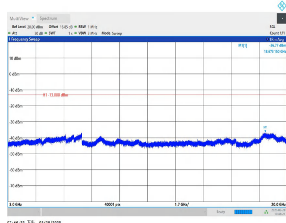
Band2-10MHz-QPSK-19150-1RB#0-3000~20000-PASS
