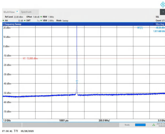
Band2-1.4MHz-QPSK-19193-1RB#0-1000~3000-PASS
