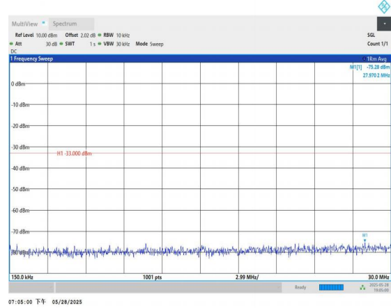
Band2-1.4MHz-QPSK-18607-1RB#0-0.15~30-PASS
