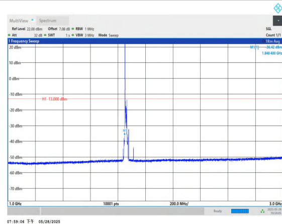
Band2-15MHz-QPSK-18675-1RB#0-1000~3000-PASS
