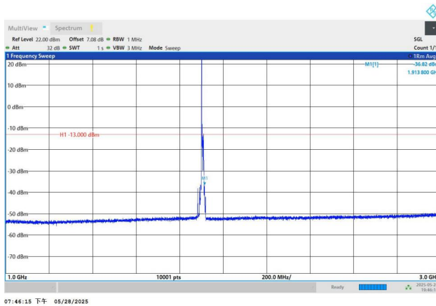
Band2-10MHz-QPSK-19150-1RB#0-1000~3000-PASS
