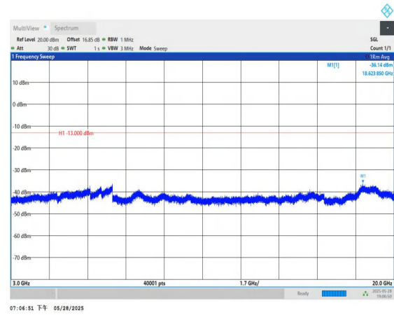
Band2-1.4MHz-QPSK-19193-1RB#0-3000~20000-PASS
