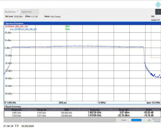
Band2-15MHz-QPSK-19125-75RB#0-PASS
