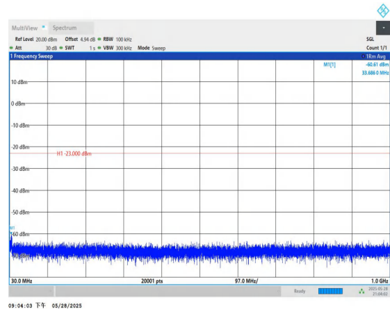
Band4-10MHz-QPSK-20350-1RB#0-30~1000-PASS
