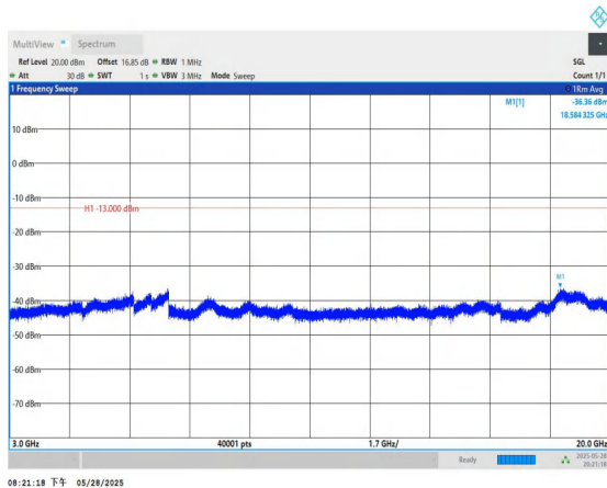
Band4-1.4MHz-QPSK-20393-1RB#0-3000~20000-PASS
