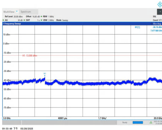
Band4-10MHz-QPSK-20175-1RB#0-3000~20000-PASS
