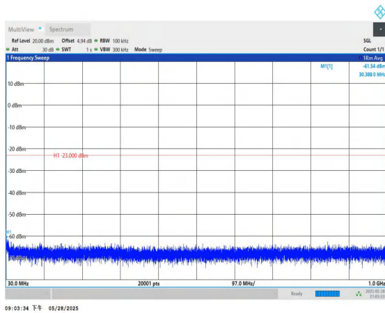
Band4-10MHz-QPSK-20175-1RB#0-30~1000-PASS
