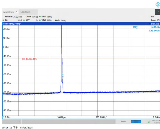
Band4-10MHz-QPSK-20350-1RB#0-1000~3000-PASS
