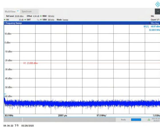
Band4-3MHz-QPSK-19965-1RB#0-30~1000-PASS
