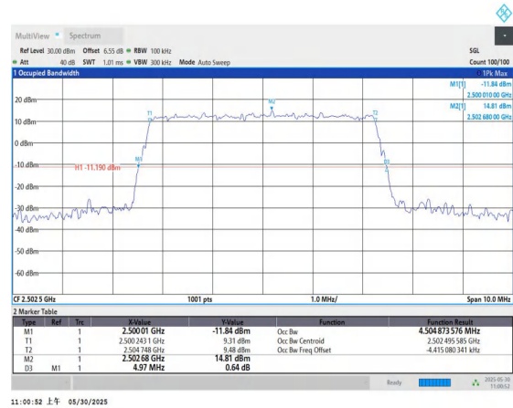
Band7-5MHz-16QAM-20775-25RB#0-PASS
