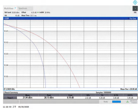
Band7-5MHz-QPSK-20775-25RB#0-PASS
