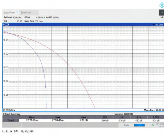
Band7-10MHz-QPSK-20800-1RB#0-PASS
