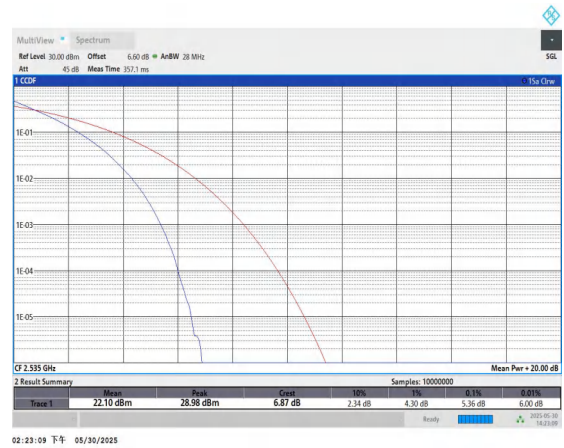
Band7-20MHz-QPSK-21100-100RB#0-PASS
