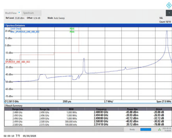
Band7-15MHz-QPSK-20825-1RB#74-PASS
