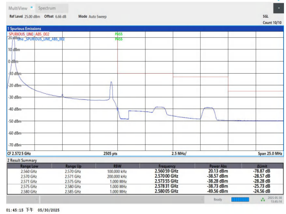
Band7-10MHz-QPSK-21400-1RB#0-PASS
