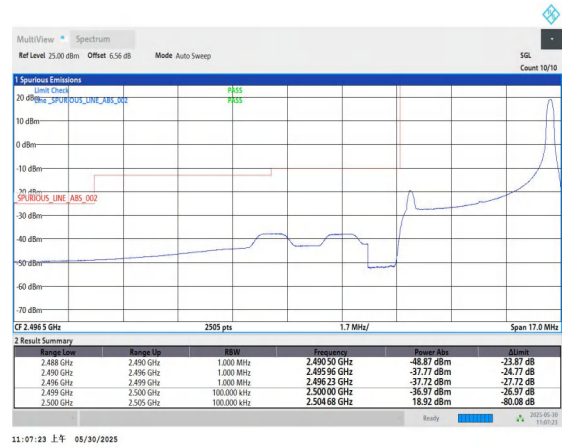
Band7-5MHz-16QAM-20775-1RB#24-PASS
