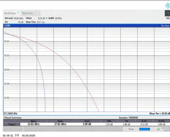
Band7-15MHz-QPSK-21375-1RB#0-PASS
