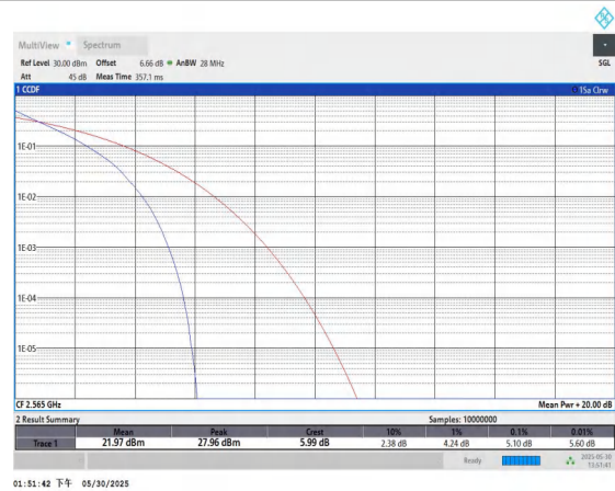
Band7-10MHz-QPSK-21400-50RB#0-PASS
