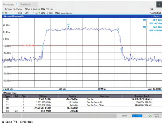
Band7-20MHz-QPSK-21350-100RB#0-PASS
