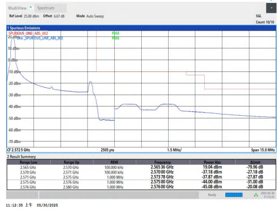
Band7-5MHz-16QAM-21425-1RB#0-PASS
