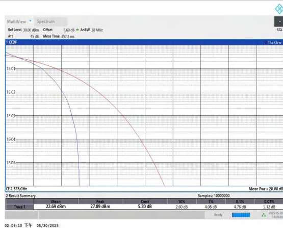
Band7-15MHz-QPSK-21100-1RB#0-PASS
