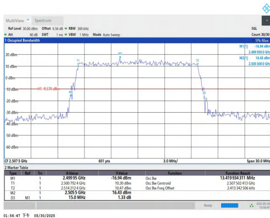
Band7-15MHz-QPSK-20825-75RB#0-PASS
