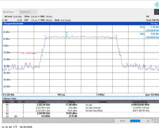
Band7-5MHz-16QAM-21100-25RB#0-PASS
