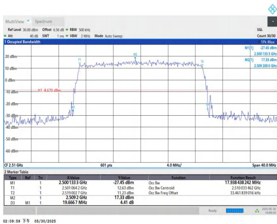
Band7-20MHz-QPSK-20850-100RB#0-PASS
