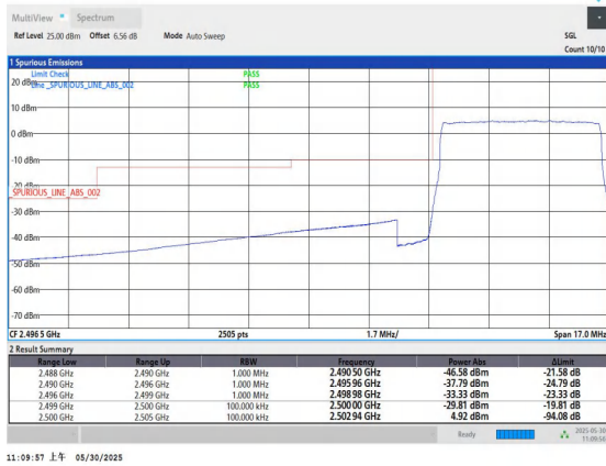
Band7-5MHz-16QAM-20775-25RB#0-PASS
