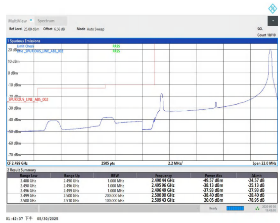
Band7-10MHz-QPSK-20800-1RB#49-PASS
