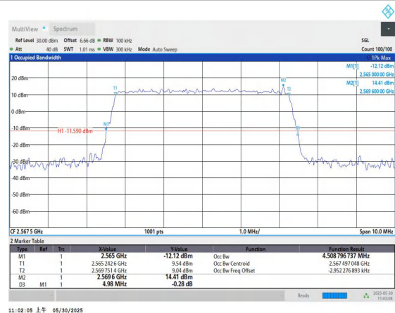
Band7-5MHz-16QAM-21425-25RB#0-PASS
