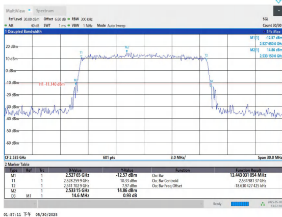
Band7-15MHz-16QAM-21100-75RB#0-PASS
