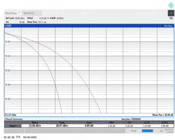
Band7-20MHz-QPSK-20850-100RB#0-PASS
