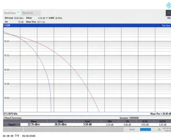
Band7-15MHz-QPSK-20825-1RB#0-PASS
