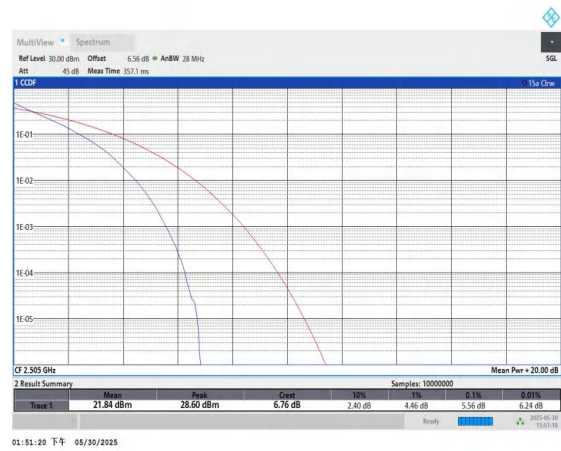
Band7-10MHz-QPSK-20800-50RB#0-PASS
