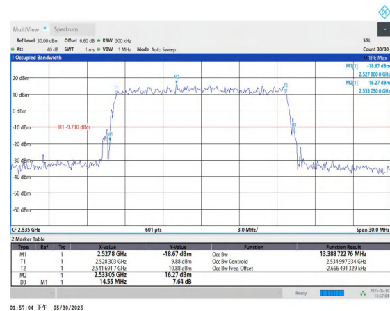
Band7-15MHz-QPSK-21100-75RB#0-PASS
