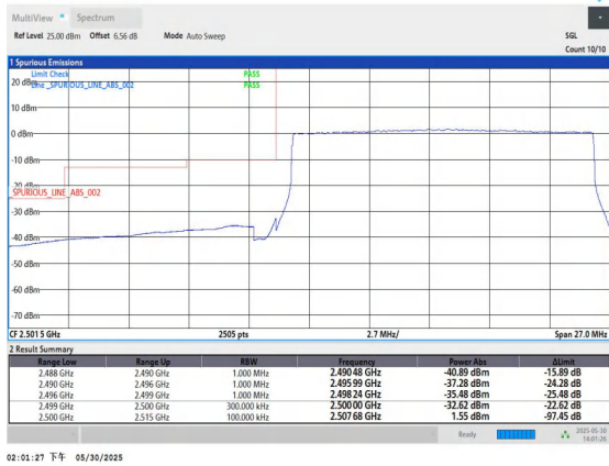
Band7-15MHz-QPSK-20825-75RB#0-PASS
