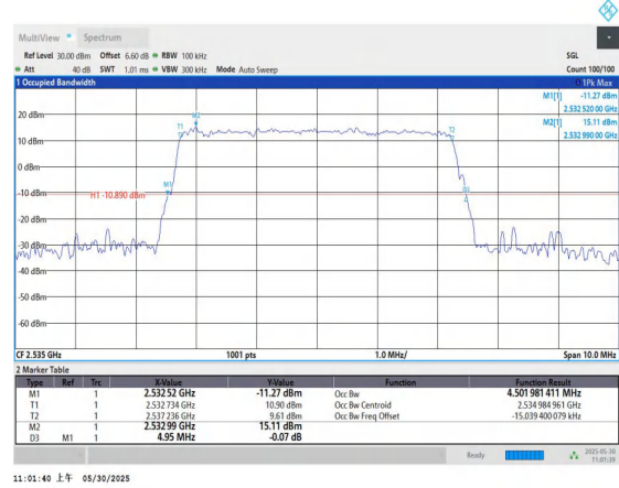
Band7-5MHz-QPSK-21100-25RB#0-PASS
