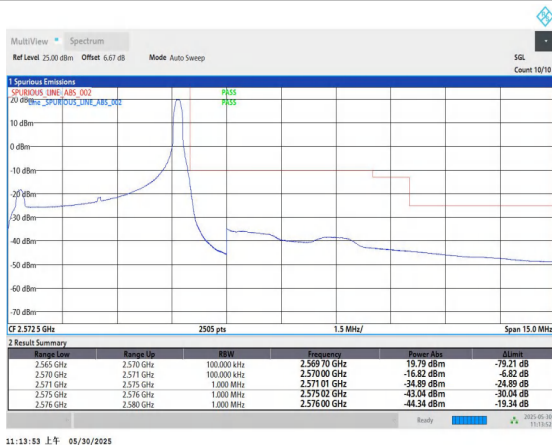
Band7-5MHz-QPSK-21425-1RB#24-PASS
