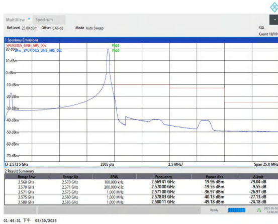
Band7-10MHz-QPSK-21400-1RB#49-PASS
