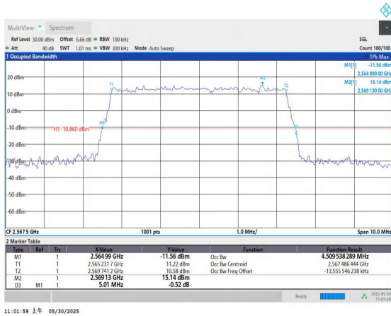
Band7-5MHz-QPSK-21425-25RB#0-PASS
