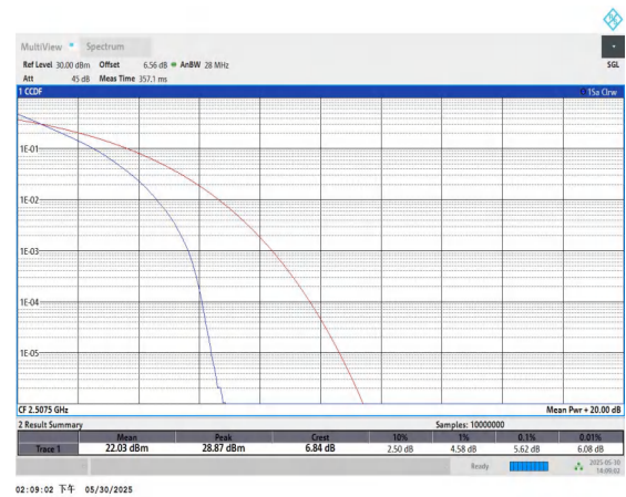
Band7-15MHz-QPSK-20825-75RB#0-PASS
