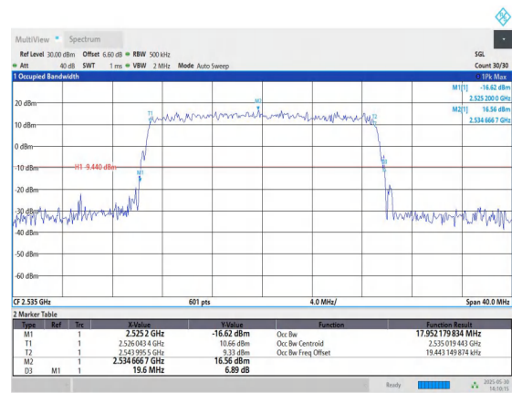
Band7-20MHz-QPSK-21100-100RB#0-PASS
