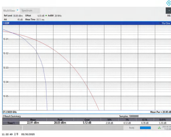
Band7-5MHz-QPSK-20775-1RB#0-PASS
