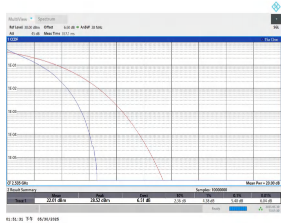
Band7-10MHz-QPSK-21100-50RB#0-PASS
