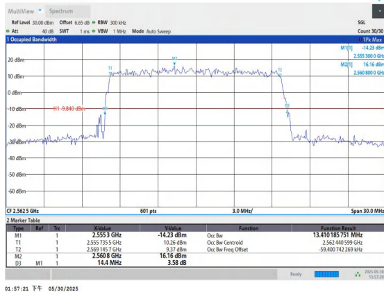
Band7-15MHz-QPSK-21375-75RB#0-PASS
