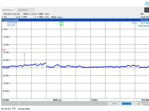
NTNV-n41-PC3-30-40-H-DFT-BPSK-Edge_1RB_Left-3000-1800 0-PASS
