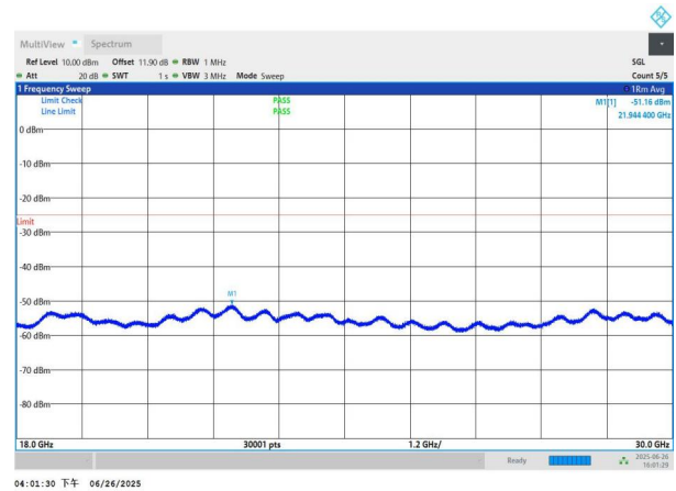
NTNV-n41-PC3-30-30-H-DFT-BPSK-Edge_1RB_Left-18000-3000 0-PASS
