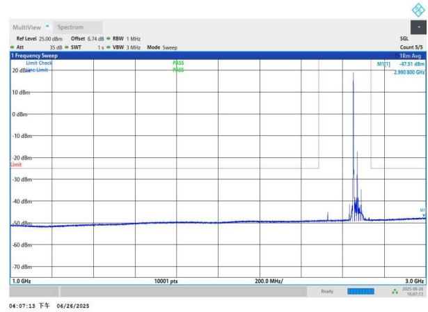
NTNV-n41-PC3-30-40-H-DFT-QPSK-Edge_1RB_Left-1000-3000-P PASS
