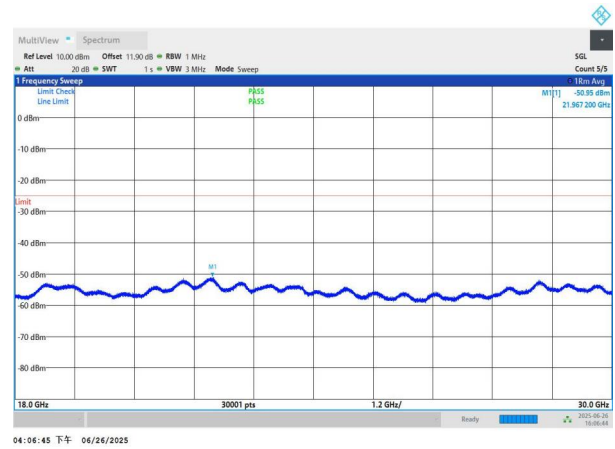
NTNV-n41-PC3-30-40-H-DFT-BPSK-Edge_1RB_Left-18000-3000 0-PASS
