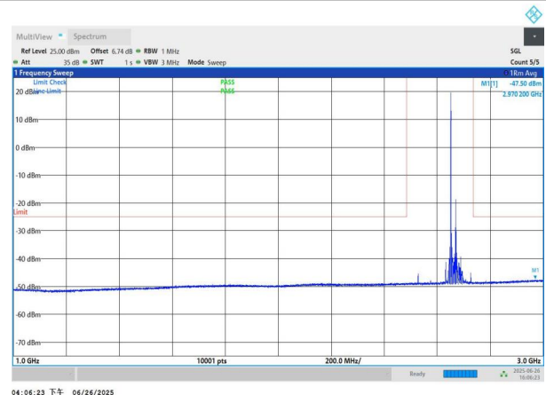
NTNV-n41-PC3-30-40-H-DFT-BPSK-Edge_1RB_Left-1000-3000-P ASS
