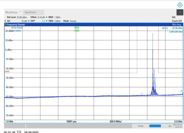
NTNV-n41-PC3-30-30-H-DFT-BPSK-Edge_1RB_Left-1000-3000-P ASS
