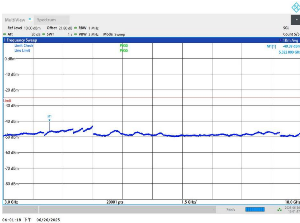
NTNV-n41-PC3-30-30-H-DFT-BPSK-Edge_1RB_Left-3000-1800 0-PASS
