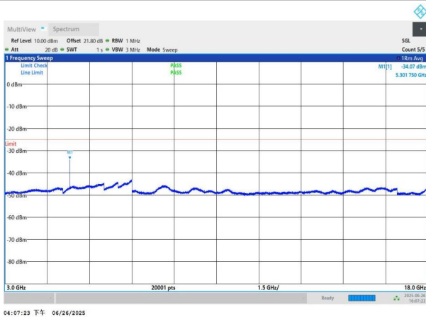
NTNV-n41-PC3-30-40-H-DFT-QPSK-Edge_1RB_Left-3000-1800 0-PASS
