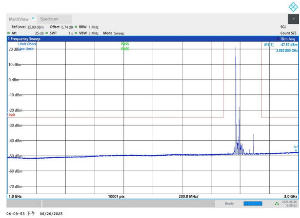
NTNV-n41-PC3-30-50-M-DFT-BPSK-Edge_1RB_Left-1000-3000-P PASS
