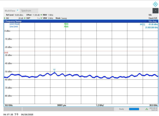
NTNV-n41-PC3-30-40-H-DFT-QPSK-Edge_1RB_Left-18000-3000 0-PASS
