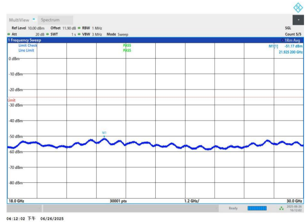
NTNV-n41-PC3-30-50-H-DFT-BPSK-Edge_1RB_Left-18000-3000 0-PASS
