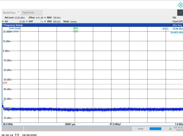
NTNV-n41-PC3-30-40-H-DFT-BPSK-Edge_1RB_Left-30-1000-P ASS
