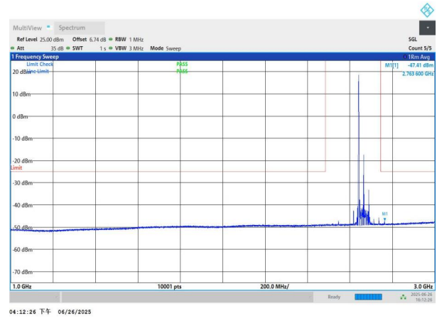
NTNV-n41-PC3-30-50-H-DFT-QPSK-Edge_1RB_Left-1000-3000-P PASS
