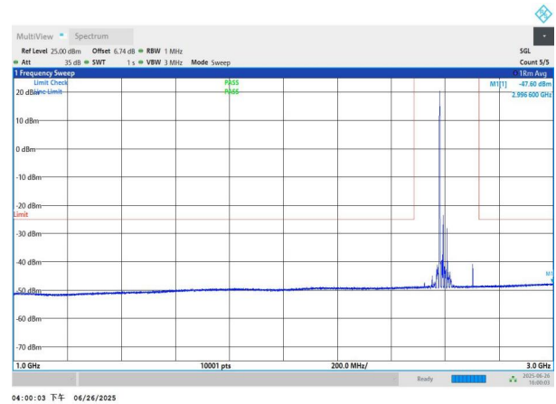
NTNV-n41-PC3-30-30-M-DFT-QPSK-Edge_1RB_Left-1000-3000- PASS
