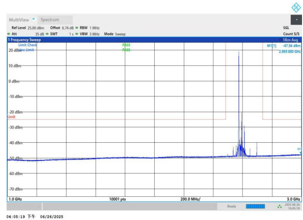
NTNV-n41-PC3-30-40-M-DFT-QPSK-Edge_1RB_Left-1000-3000- PASS
