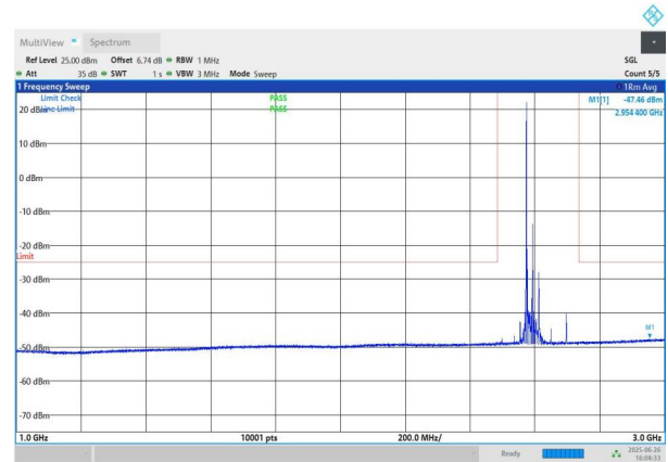
NTNV-n41-PC3-30-40-M-DFT-BPSK-Edge_1RB_Left-1000-3000-P PASS
