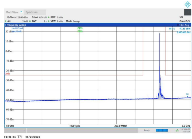
NTNV-n41-PC3-30-30-H-DFT-QPSK-Edge_1RB_Left-1000-3000-P PASS
