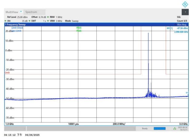
NTNV-n41-PC3-30-60-M-DFT-BPSK-Edge_1RB_Left-1000-3000-P PASS
