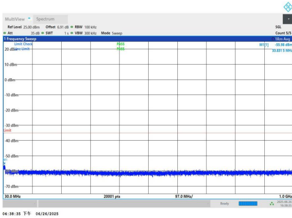
NTNV-n41-PC3-30-100-H-DFT-QPSK-Edge_1RB_Left-30-1000- PASS
