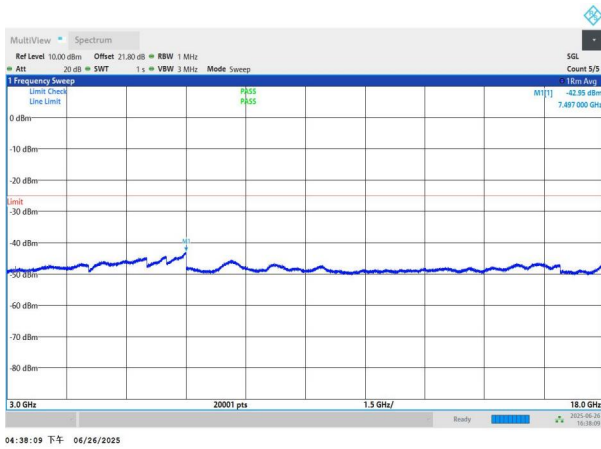
NTNV-n41-PC3-30-100-H-DFT-BPSK-Edge_1RB_Left-3000-180 00-PASS
