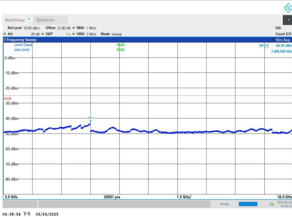
NTNV-n41-PC3-30-100-H-DFT-QPSK-Edge_1RB_Left-3000-180 00-PASS
