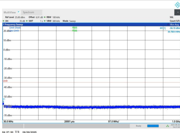
NTNV-n41-PC3-30-100-H-DFT-BPSK-Edge_1RB_Left-30-1000-PASS
