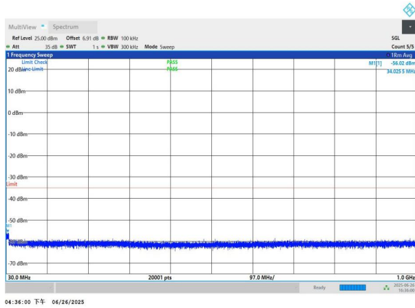
NTNV-n41-PC3-30-100-M-DFT-BPSK-Edge_1RB_Left-30-1000- PASS
