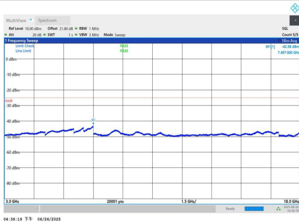
NTNV-n41-PC3-30-100-M-DFT-BPSK-Edge_1RB_Left-3000-180 00-PASS
