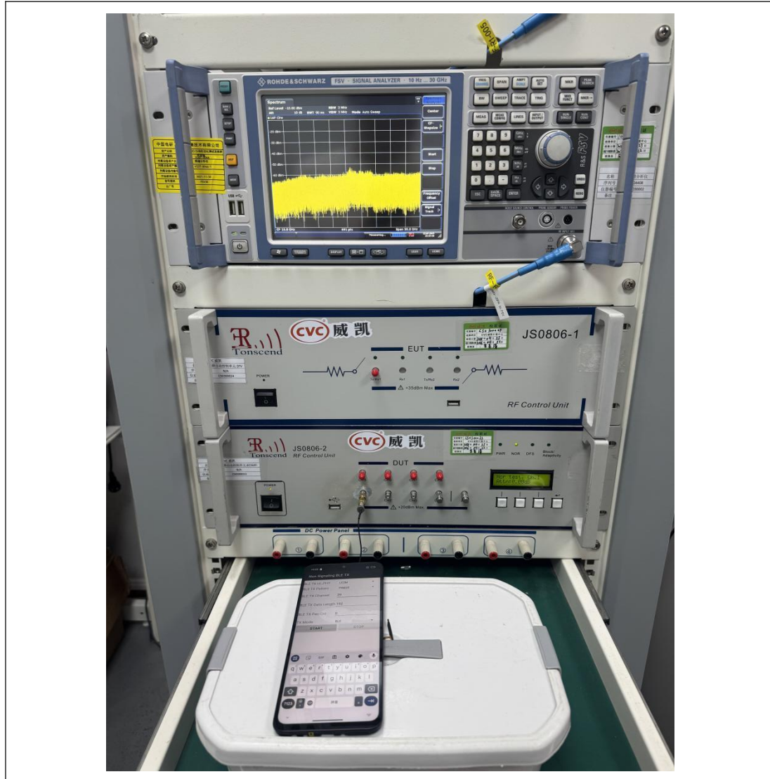
ANTENNA PORT CONDUCTED TEST
