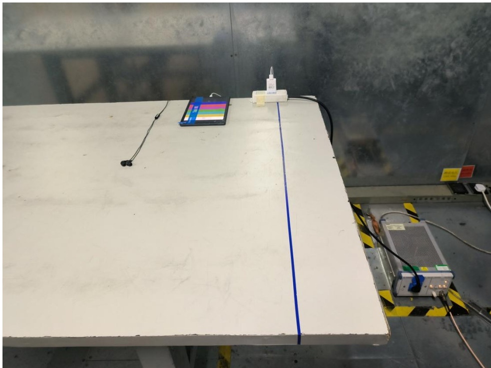
AC Conducted Measurement Photos -Adapter 2
