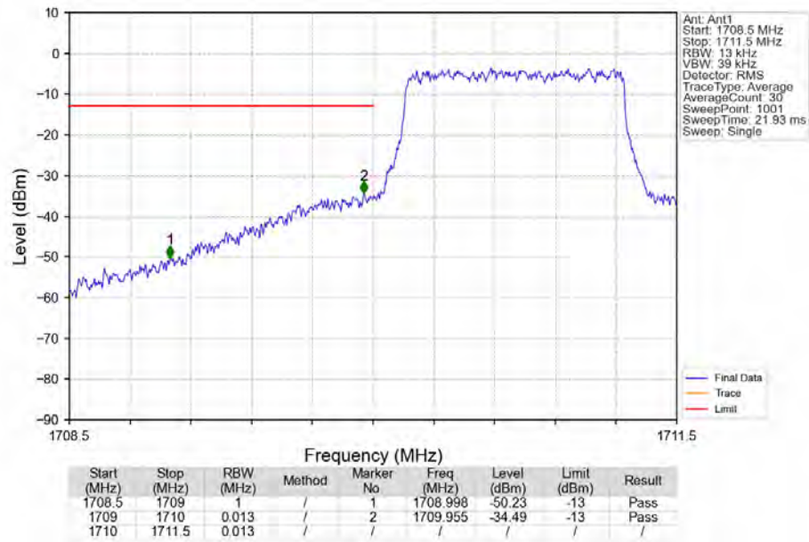
Band4_1.4MHz_16QAM_LCH_1710.7MHz_RB_6_0_NTNV
