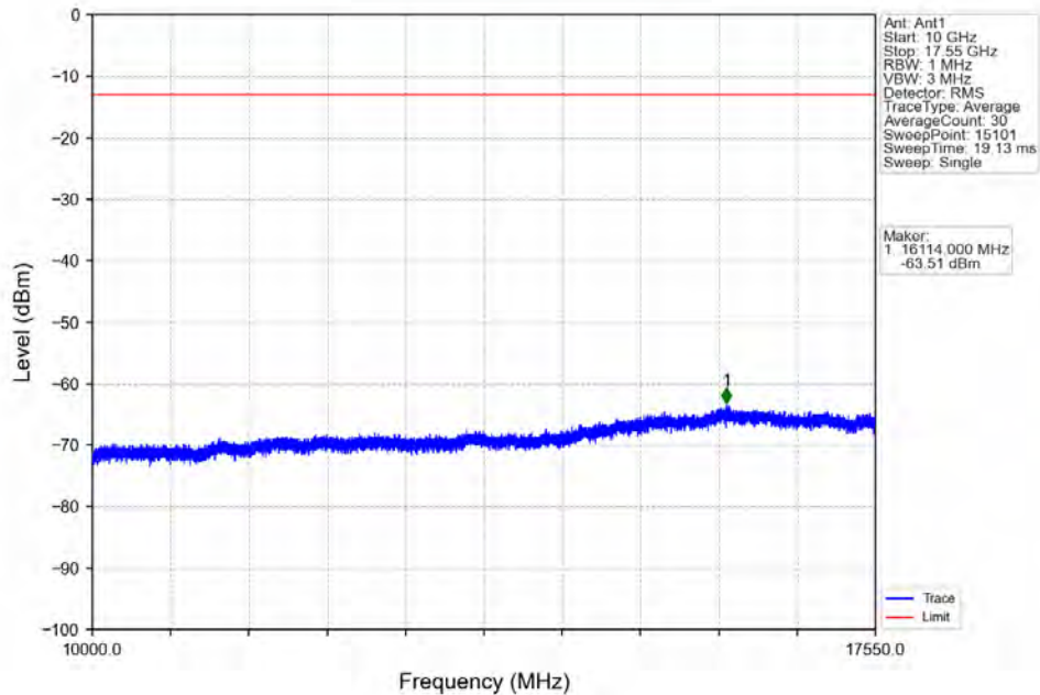
Band4_15MHz_16QAM_HCH_1747.5MHz_RB_1_0_NTNV
