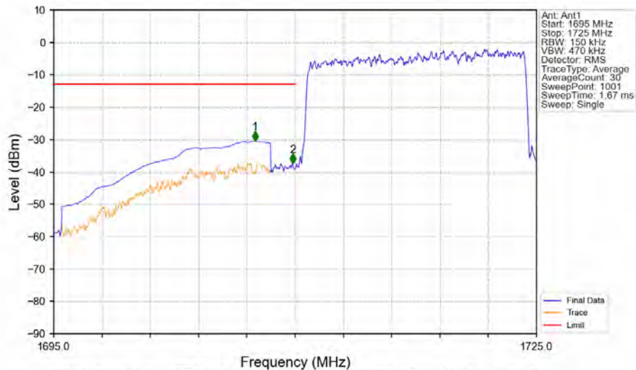
Band4_15MHz_16QAM_LCH_1717.5MHz_RB_75_0_NTNV
