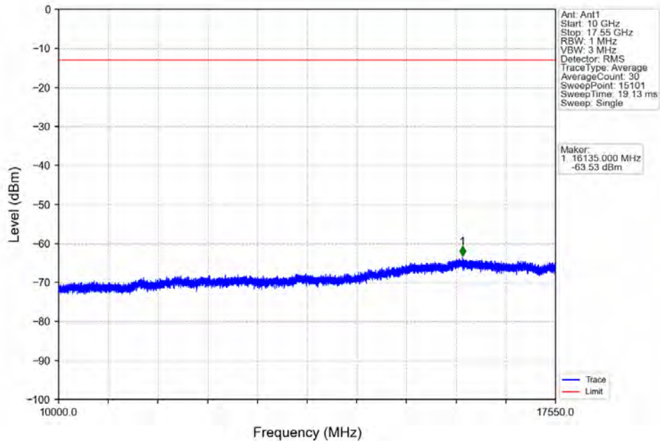
Band4_20MHz_16QAM_MCH_1732.5MHz_RB_1_0_NTNV
