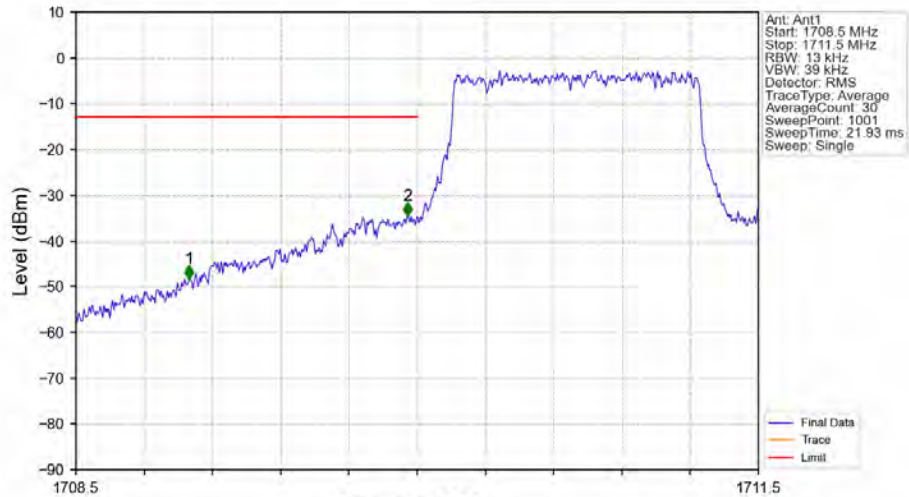
Band4_1.4MHz_QPSK_LCH_1710.7MHz_RB_6_0_NTNV
