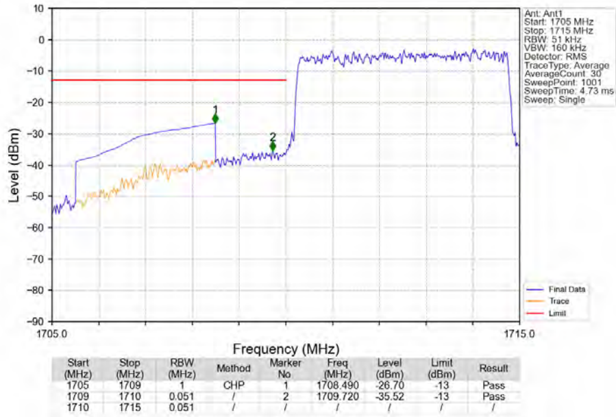
Band4_5MHz_16QAM_LCH_1712.5MHz_RB_25_0_NTNV
