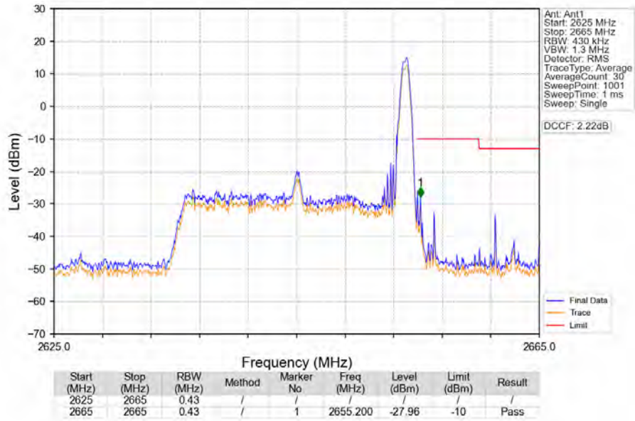
Band41_20MHz_16QAM_HCH_2645MHz_RB_1_99_NTNV
