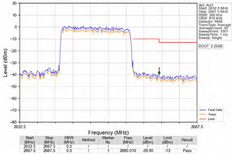
Band41_15MHz_QPSK_HCH_2647.5MHz_RB_75_0_NTNV
