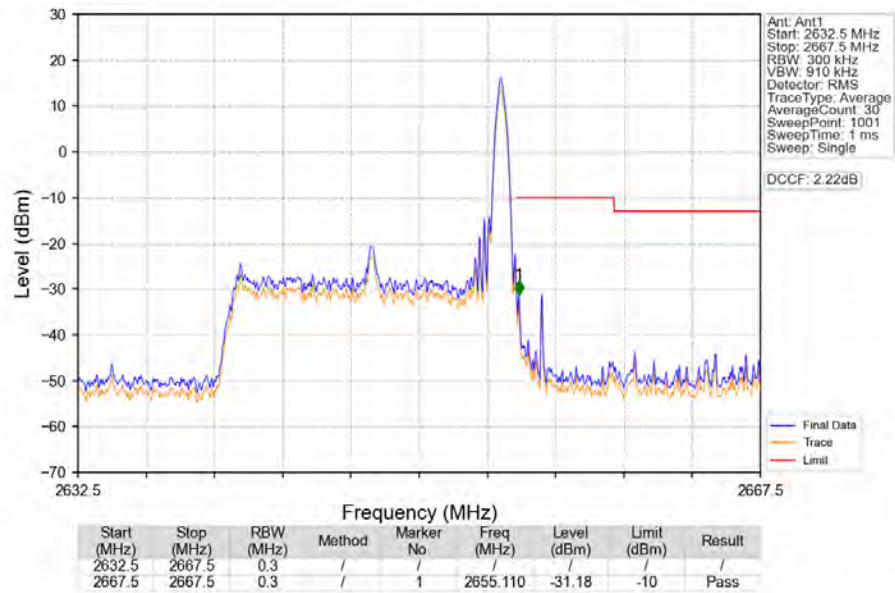
Band41_15MHz_16QAM_HCH_2647.5MHz_RB_1_74_NTNV
