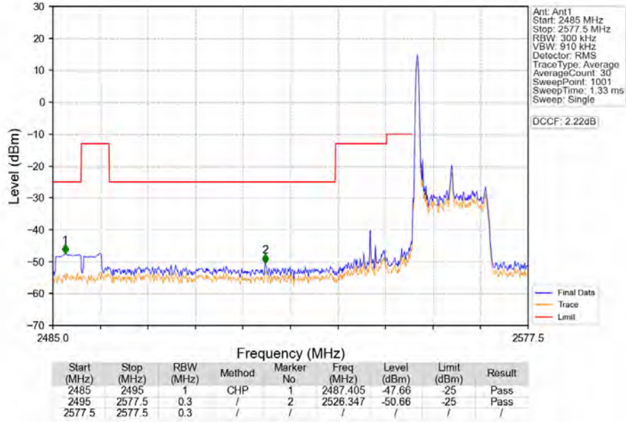
Band41_15MHz_16QAM_LCH_2562.5MHz_RB_1_0_NTNV
