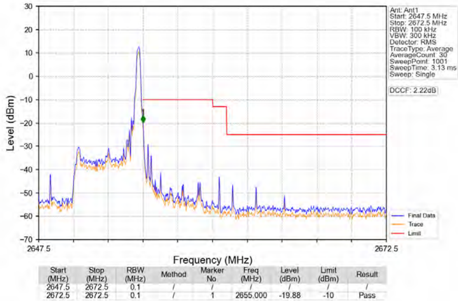
Band41_5MHz_16QAM_HCH_2652.5MHz_RB_1_24_NTNV
