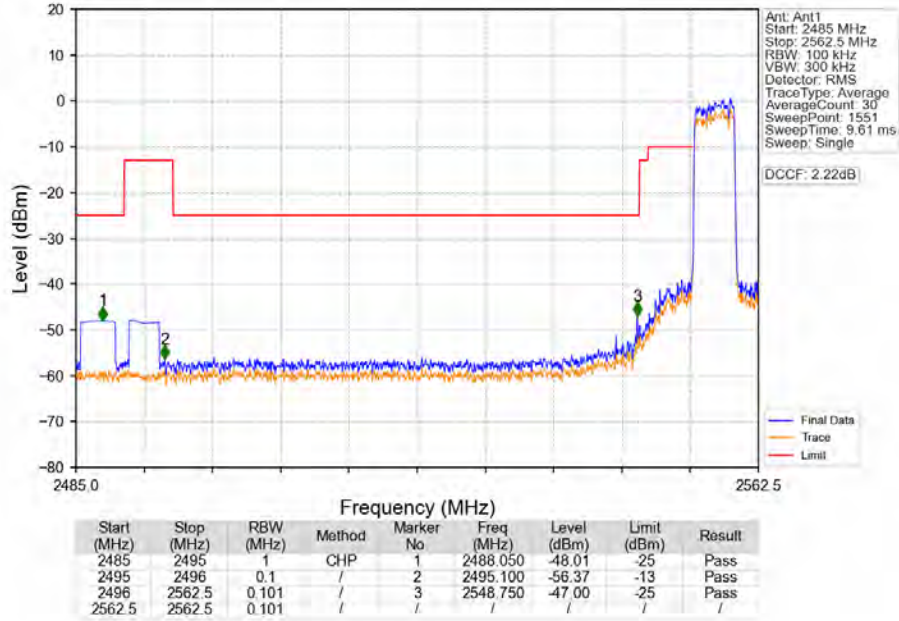
Band41_5MHz_16QAM_LCH_2557.5MHz_RB_25_0_NTNV
