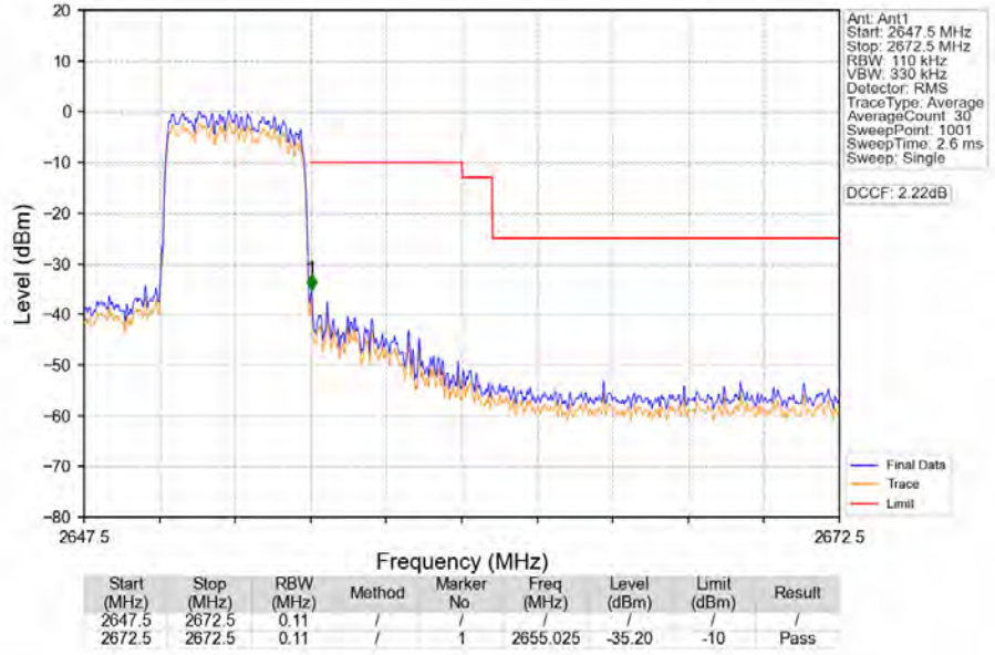
Band41_5MHz_16QAM_HCH_2652.5MHz_RB_25_0_NTNV
