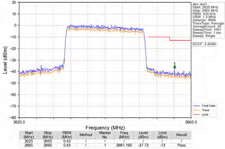
Band41_20MHz_16QAM_HCH_2645MHz_RB_100_0_NTNV
