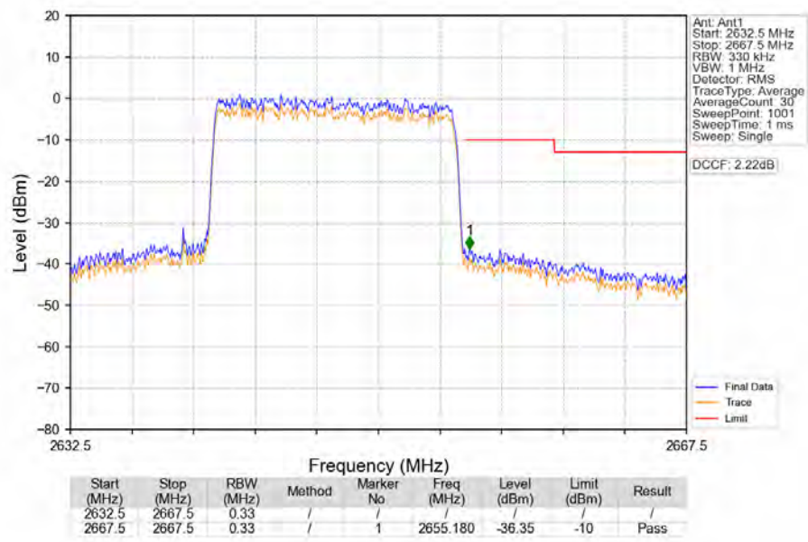
Band41_15MHz_16QAM_HCH_2647.5MHz_RB_75_0_NTNV
