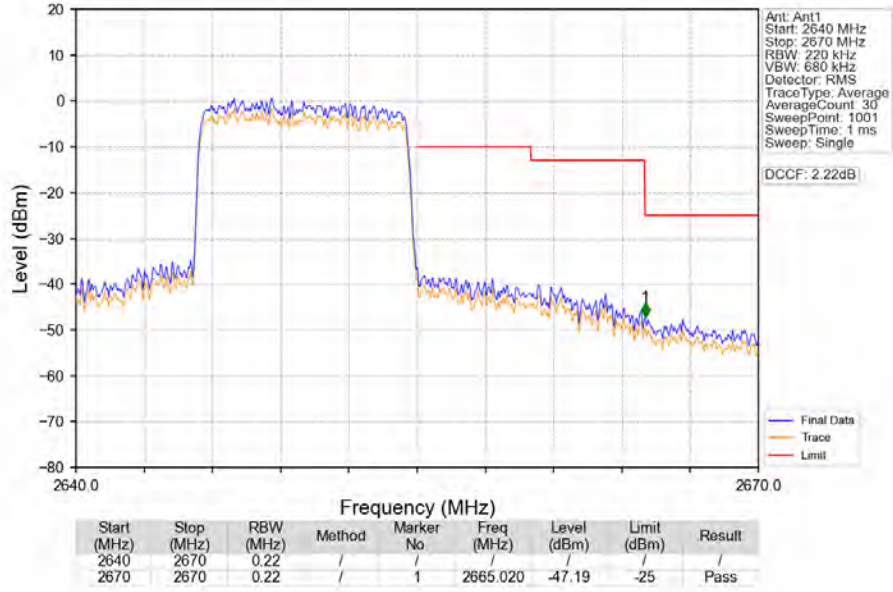
Band41_10MHz_16QAM_HCH_2650MHz_RB_50_0_NTNV
