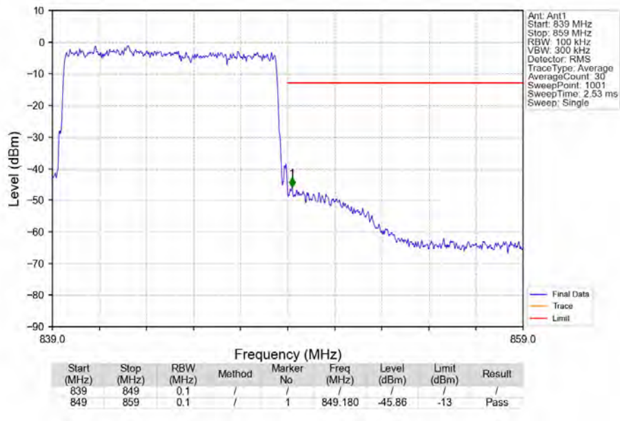
Band5_10MHz_16QAM_HCH_844MHz_RB_50_0_NTNV
