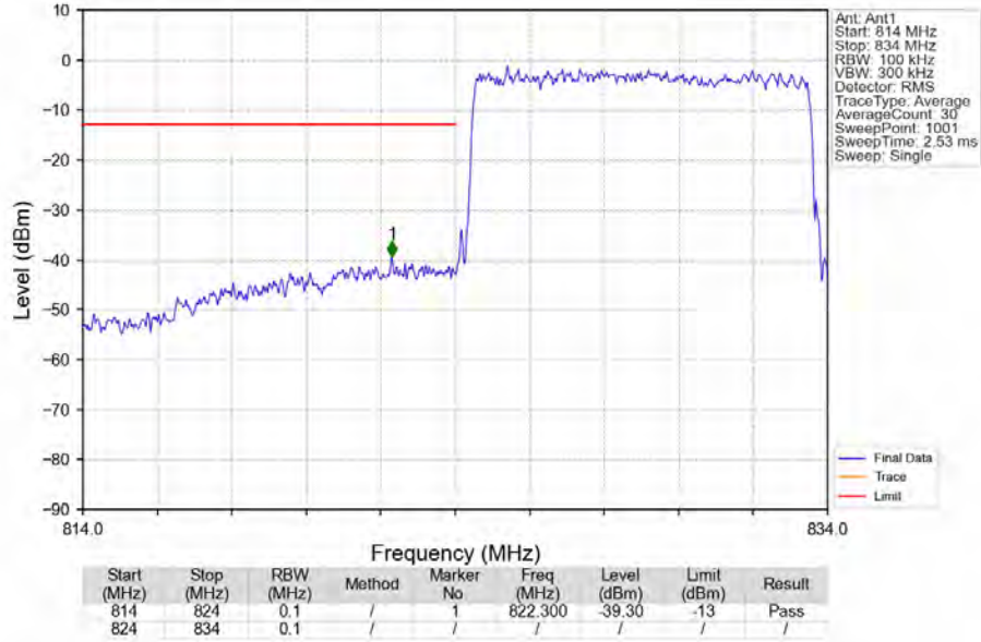
Band5_10MHz_16QAM_LCH_829MHz_RB_50_0_NTNV
