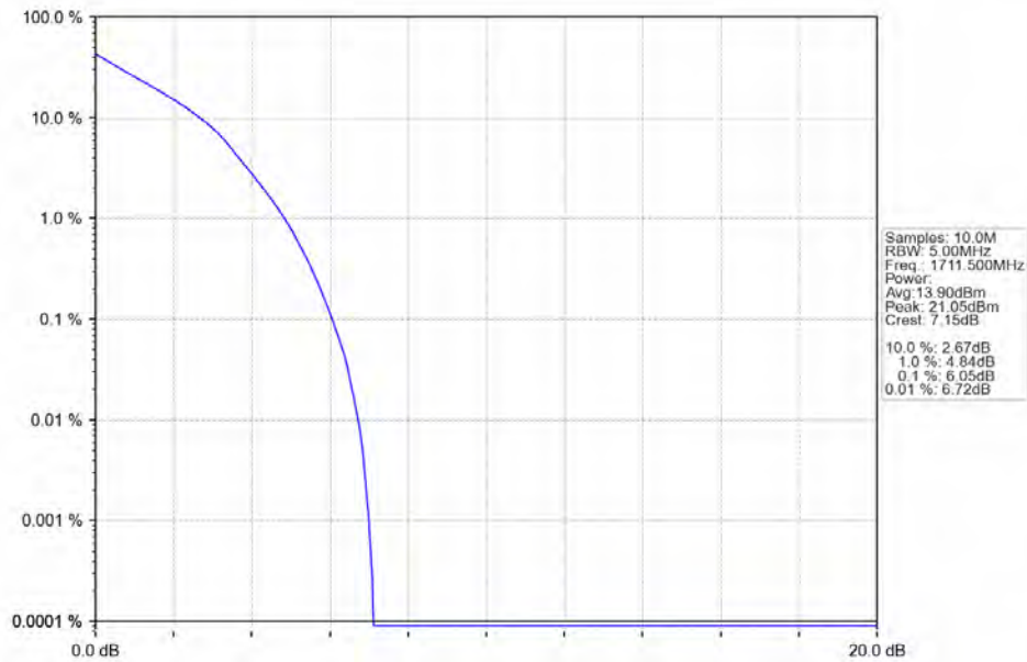
Band66 3MHz QPSK LCH 1711.5MHz RB 15 0 NTNV
