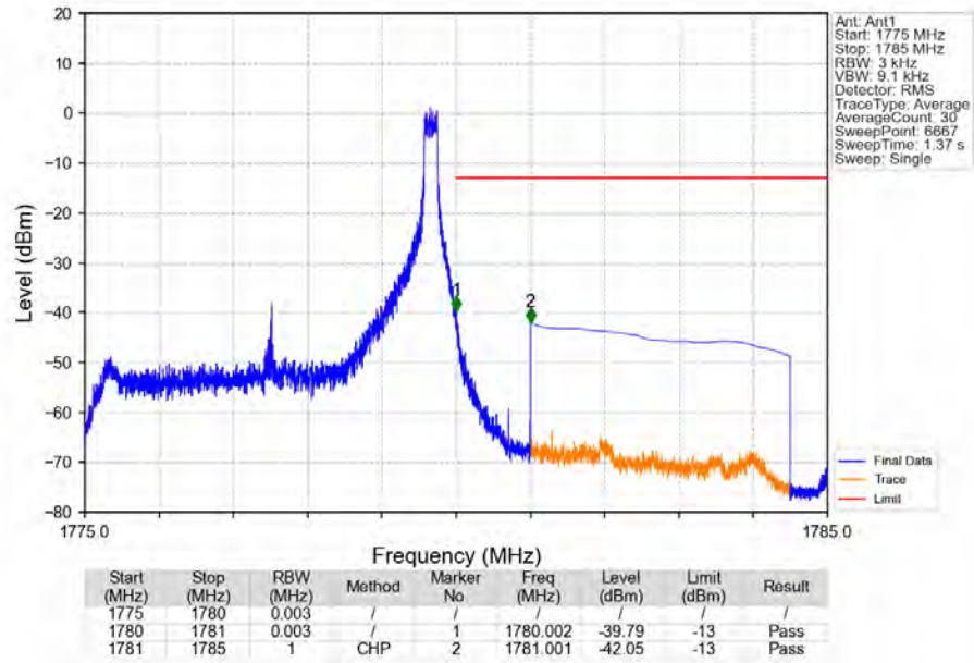
Band66_5MHz_16QAM_HCH_1777.5MHz_RB_1_24_NTNV
