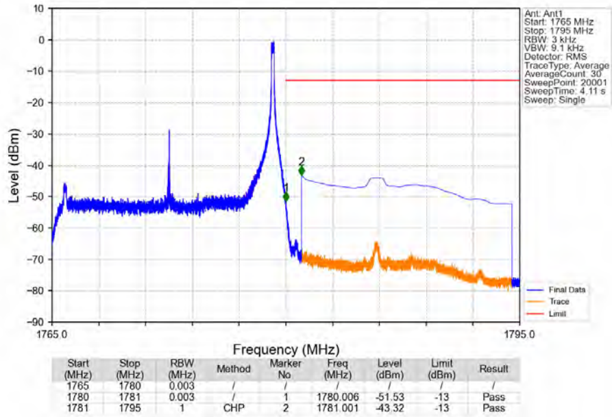
Band66_15MHz_16QAM_HCH_1772.5MHz_RB_1_74_NTNV
