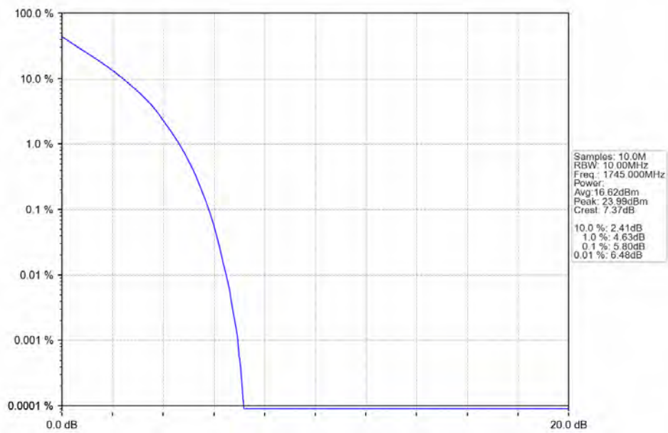
Band66_10MHz_QPSK_MCH_1745MHz_RB_50_0_NTNV
