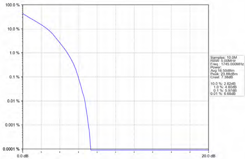
Band66 3MHz QPSK MCH 1745MHz RB 15 0 NTNV
