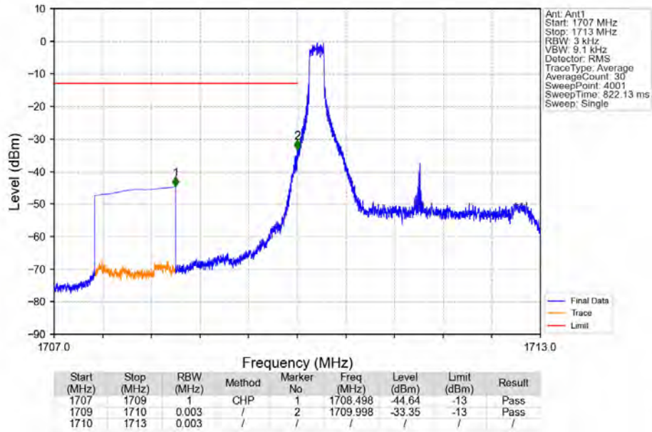
Band66 3MHz QPSK LCH 1711.5MHz RB 1 0 NTNV
