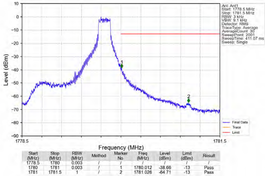
Band66_1.4MHz_16QAM_HCH_1779.3MHz_RB_1_5_NTNV
