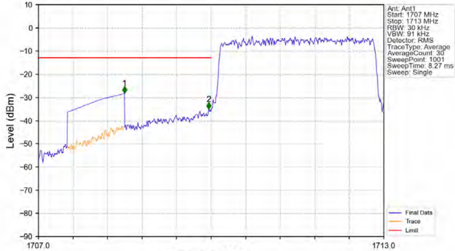
Band66_3MHz_16QAM_LCH_1711.5MHz_RB_15_0_NTNV
