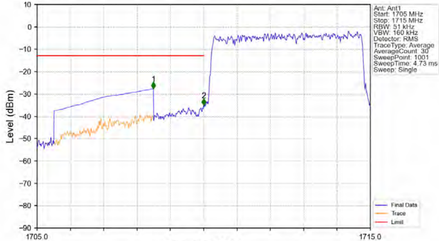
Band66_5MHz_QPSK_LCH_1712.5MHz_RB_25_0_NTNV
