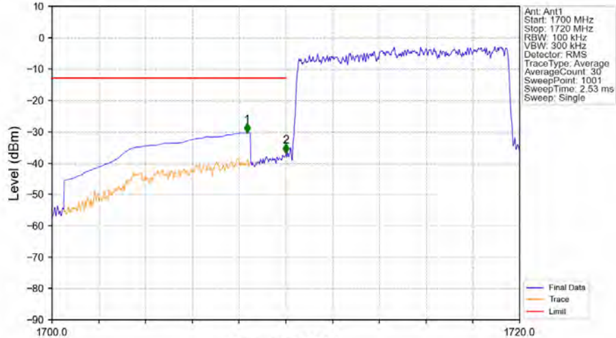
Band66_10MHz_16QAM_LCH_1715MHz_RB_50_0_NTNV
