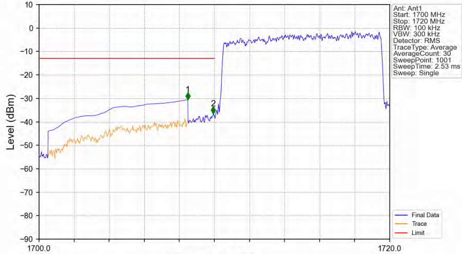
Band66_10MHz_QPSK_LCH_1715MHz_RB_50_0_NTNV
