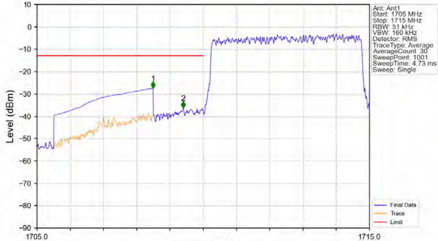
Band66_5MHz_16QAM_LCH_1712.5MHz_RB_25_0_NTNV
