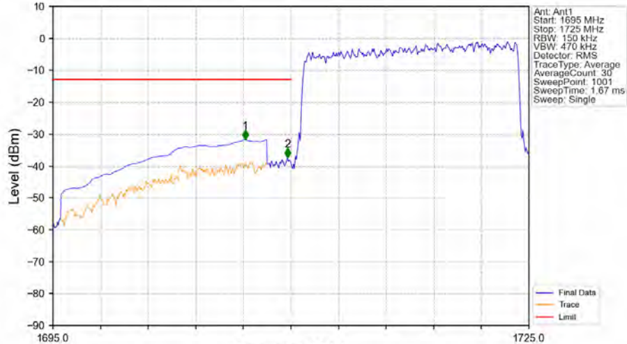
Band66_15MHz_QPSK_LCH_1717.5MHz_RB_75_0_NTNV
