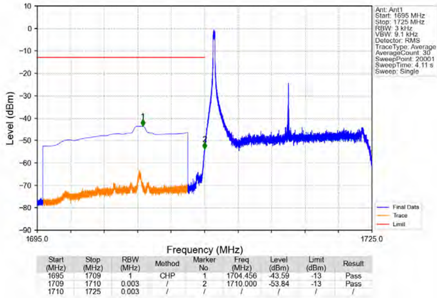
Band66_15MHz_16QAM_LCH_1717.5MHz_RB_1_0_NTNV
