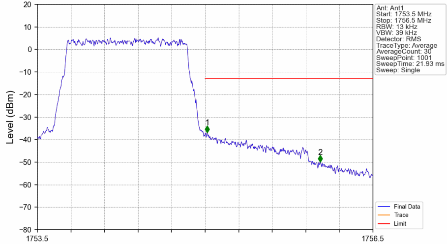
Band4_1.4MHz_QPSK_HCH_1754.3MHz_RB_6_0_NTNV
