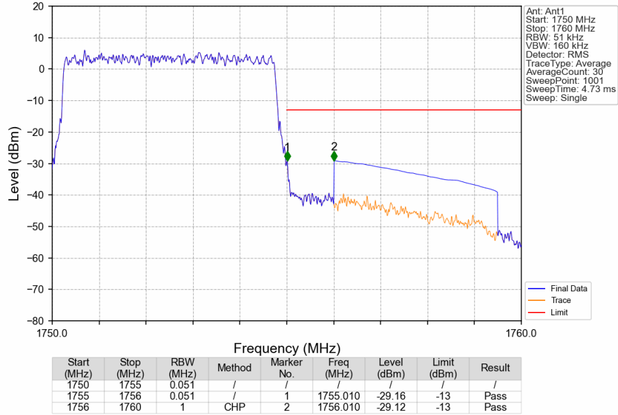
Band4_5MHz_QPSK_HCH_1752.5MHz_RB_25_0_NTNV
