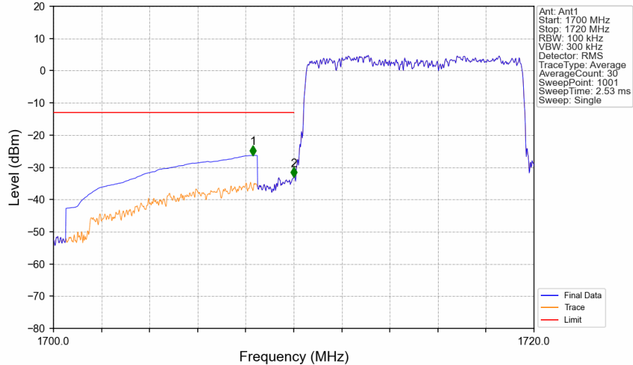
Band4_10MHz_QPSK_LCH_1715MHz_RB_50_0_NTNV
