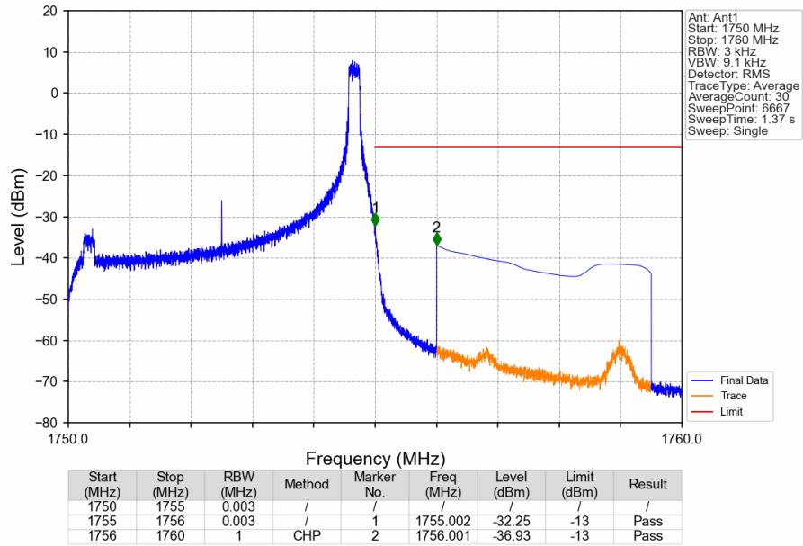
Band4_5MHz_QPSK_HCH_1752.5MHz_RB_1_24_NTNV
