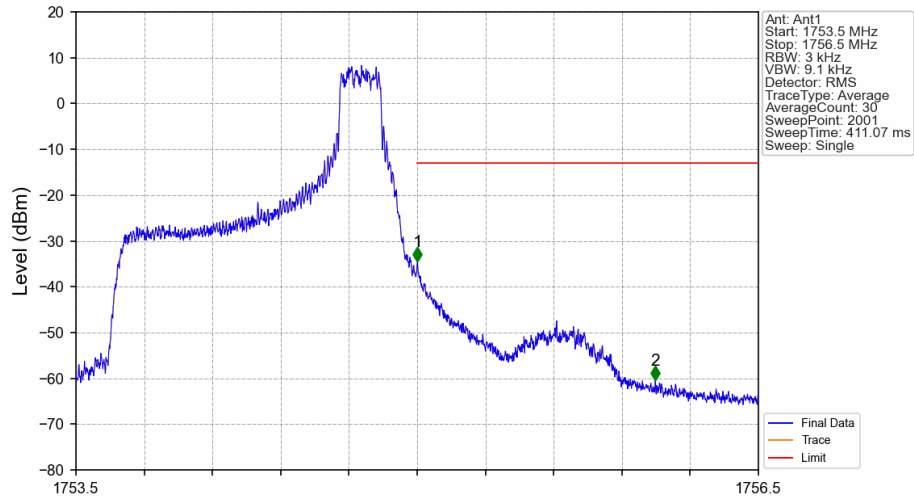
Band4_1.4MHz_QPSK_HCH_1754.3MHz_RB_1_5_NTNV
