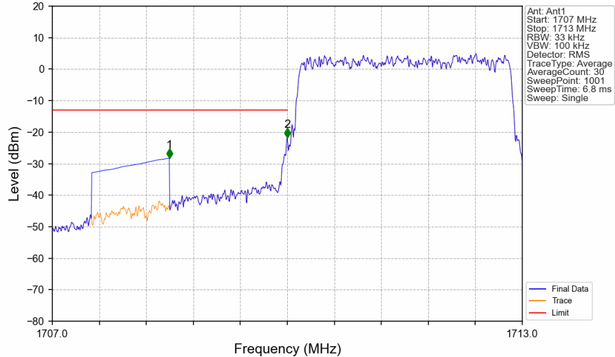
Band4_3MHz_16QAM_LCH_1711.5MHz_RB_15_0_NTNV
