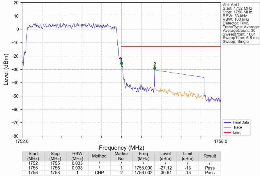
Band4_3MHz_16QAM_HCH_1753.5MHz_RB_15_0_NTNV
