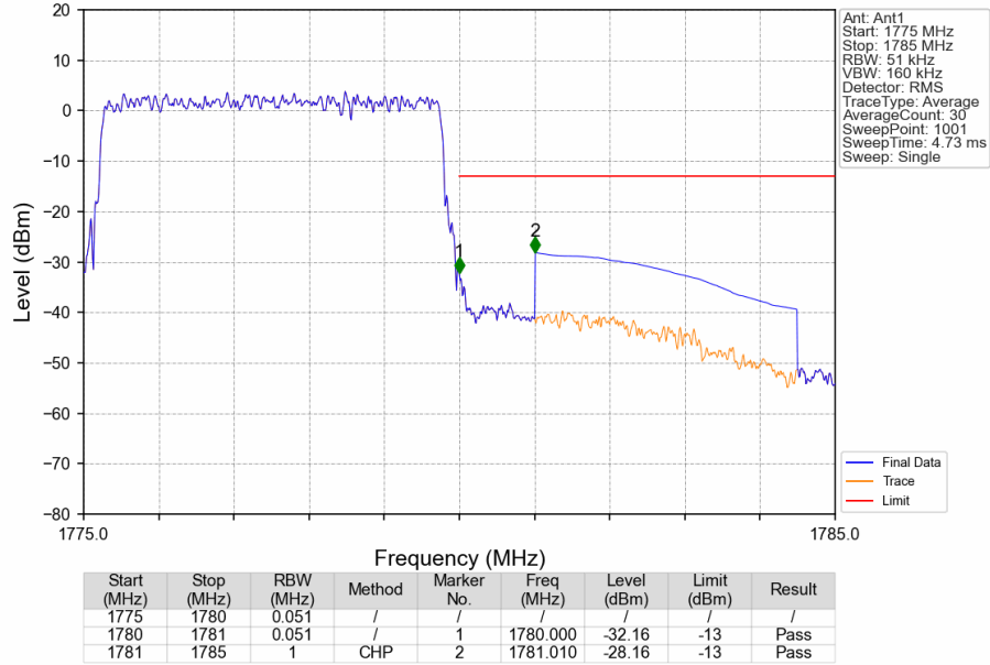
Band66_5MHz_16QAM_HCH_1777.5MHz_RB_25_0_NTNV
