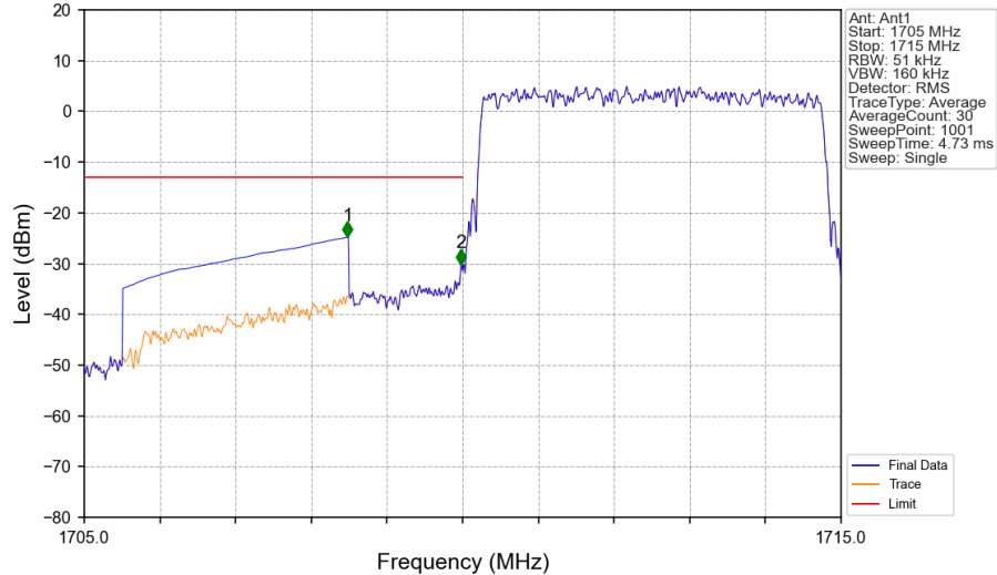
Band66_5MHz_QPSK_LCH_1712.5MHz_RB_25_0_NTNV
