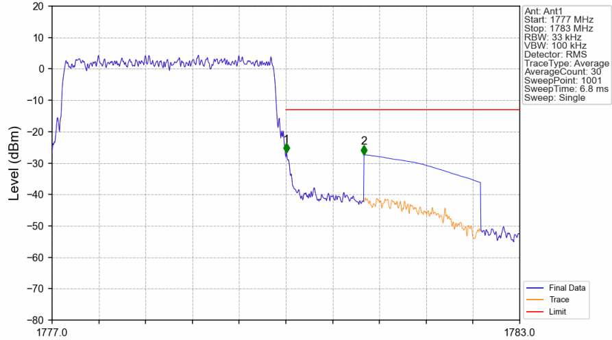
Band66_3MHz_16QAM_HCH_1778.5MHz_RB_15_0_NTNV
