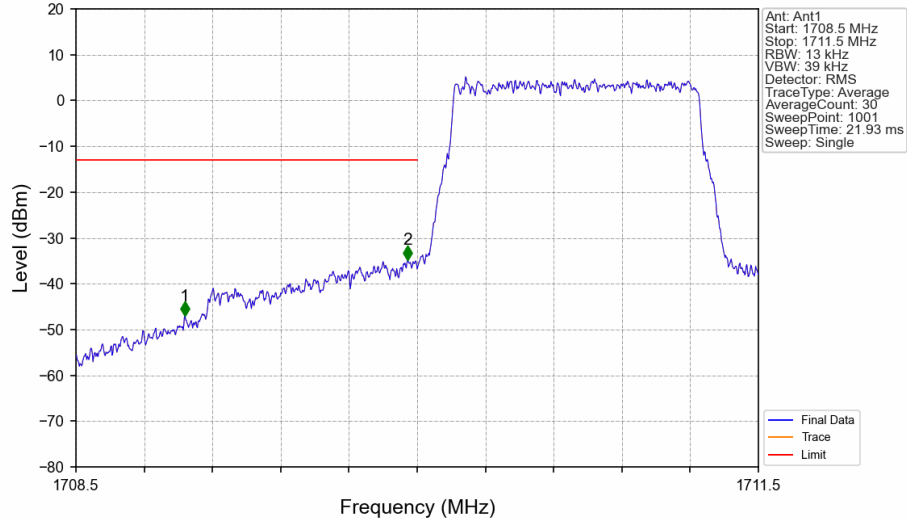
Band66_1.4MHz_QPSK_LCH_1710.7MHz_RB_6_0_NTNV
