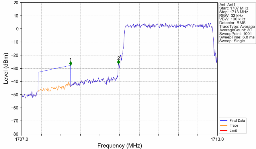
Band66_3MHz_16QAM_LCH_1711.5MHz_RB_15_0_NTNV
