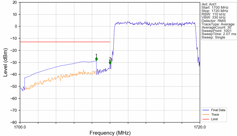
Band66_10MHz_16QAM_LCH_1715MHz_RB_50_0_NTNV
