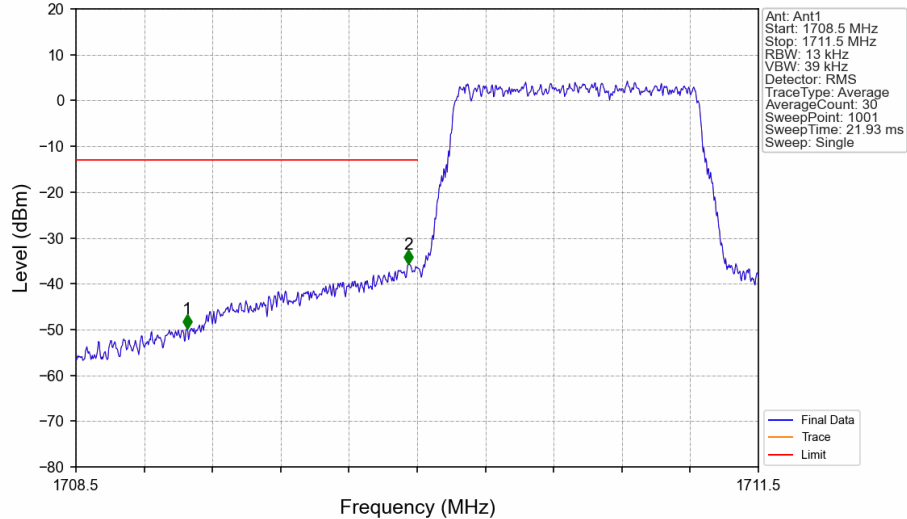
Band66_1.4MHz_16QAM_LCH_1710.7MHz_RB_6_0_NTNV
