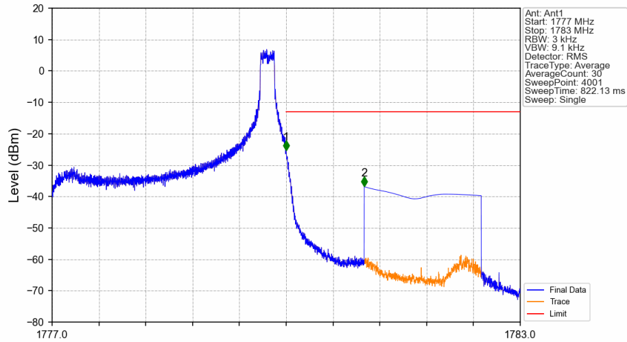
Band66_3MHz_16QAM_HCH_1778.5MHz_RB_1_14_NTNV
