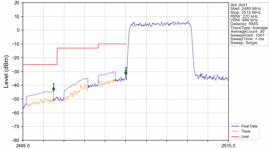
Band7_10MHz_16QAM_LCH_2505MHz_RB_50_0_NTNV
