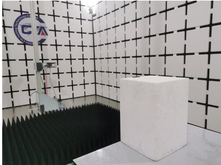
radiation H
