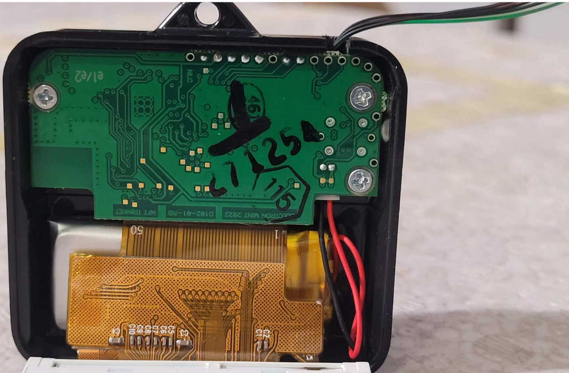
Bottom View of Green PCB
