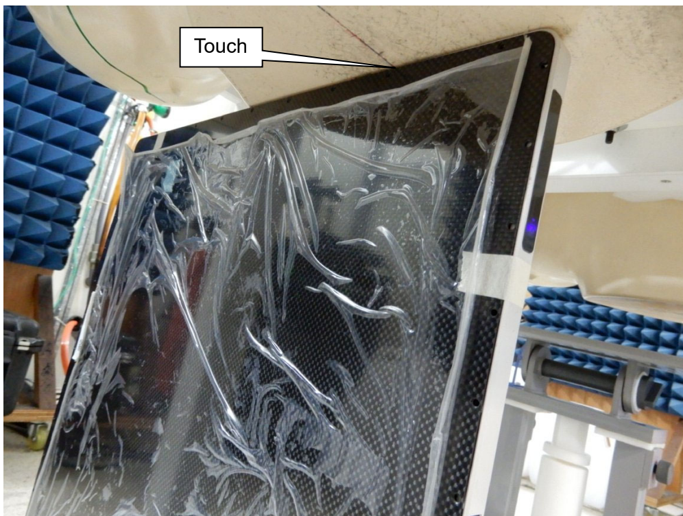
EUT Left-Side – Limb SAR (Main Antenna)
