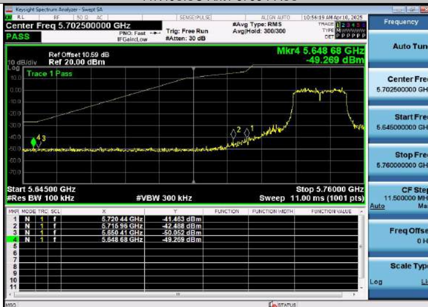
11AC20SISO-Ant1-5745-PASS
