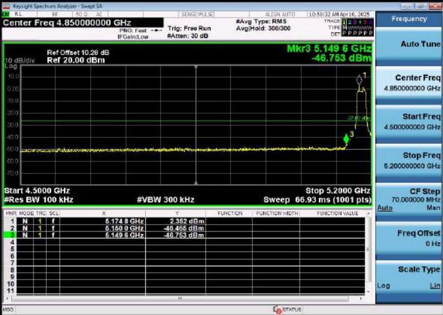
11AC20SISO-Ant1-5180-PASS
