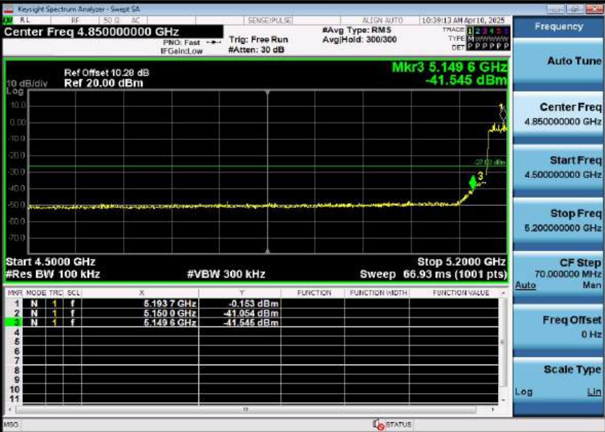
11N40SISO-Ant1-5190-PASS
