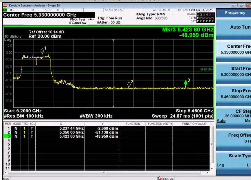
11AC40SISO-Ant1-5230-PASS
