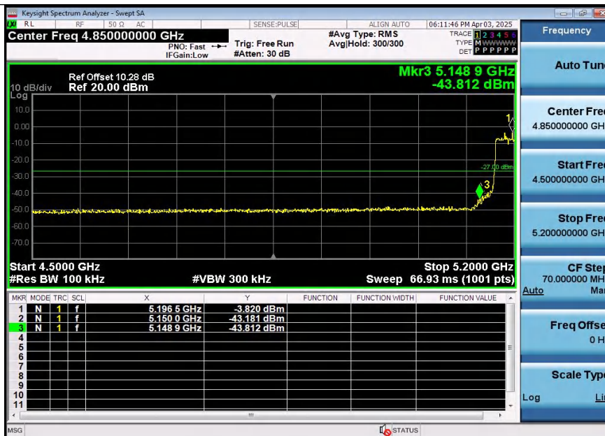
11AC40SISO-Ant1-5190-PASS
