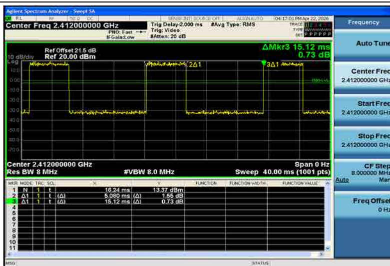
NTNV-11N20SISO-Ant1-2412
