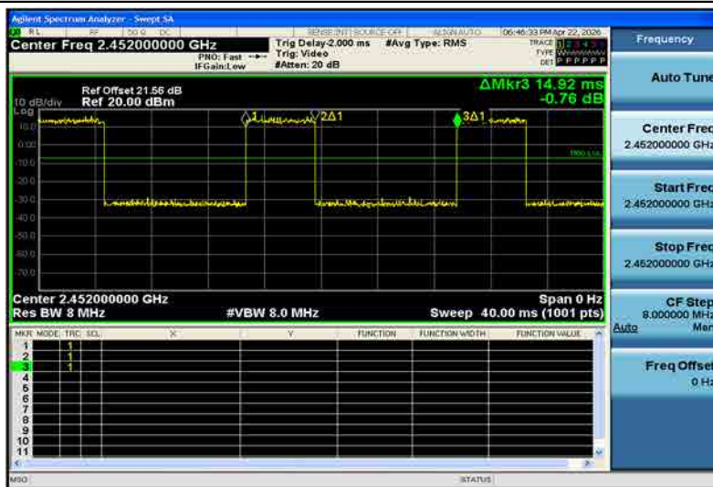
NTNV-11N40SISO-Ant1-2452
