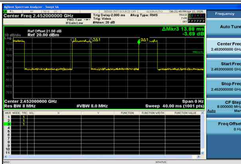
NTNV-11AX40SISO-Ant1-2452
