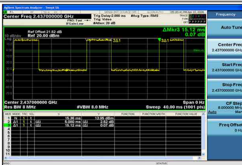
NTNV-11N20SISO-Ant1-2437
