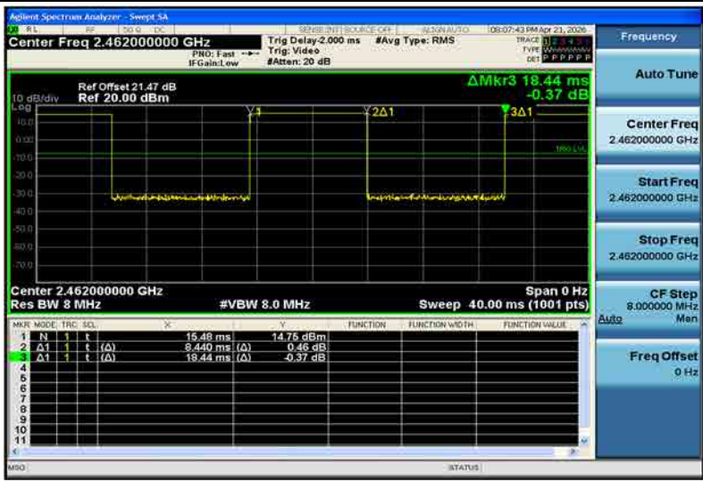
NTNV-11B-Ant1-2462
