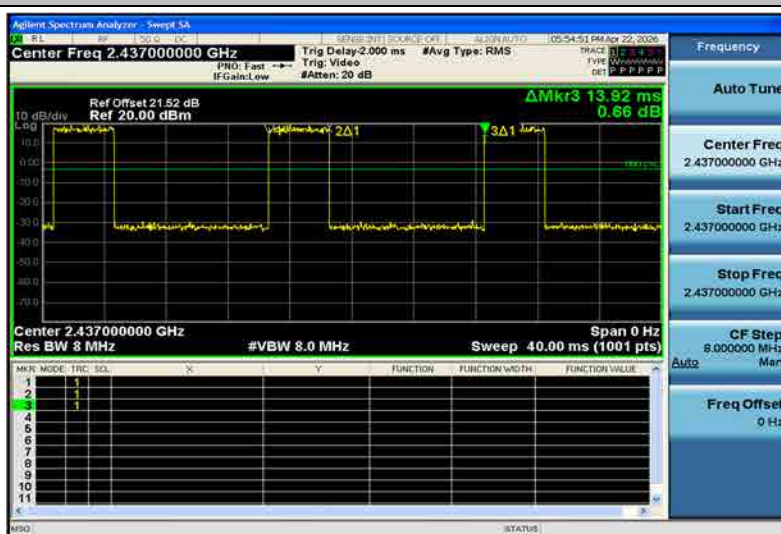
NTNV-11AX20SISO-Ant1-2437
