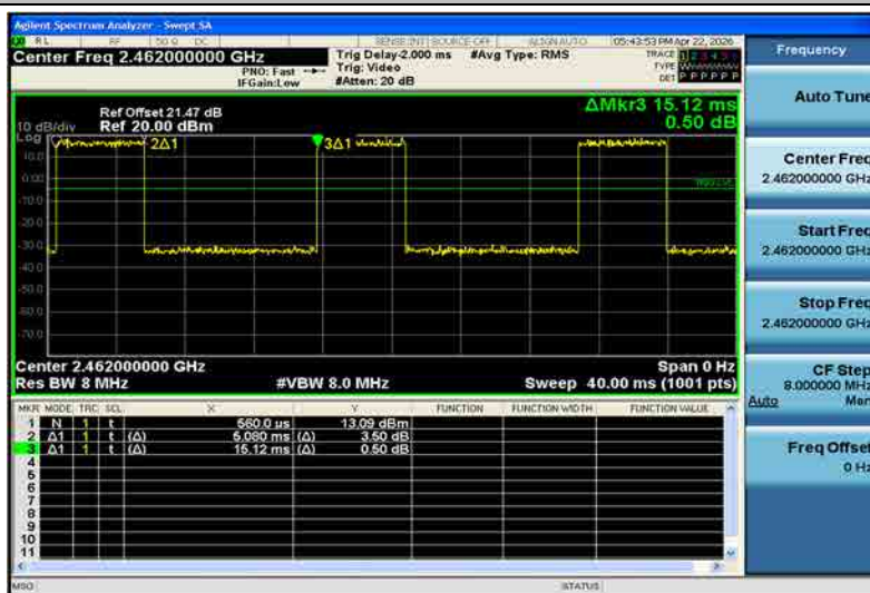
NTNV-11N20SISO-Ant1-2462
