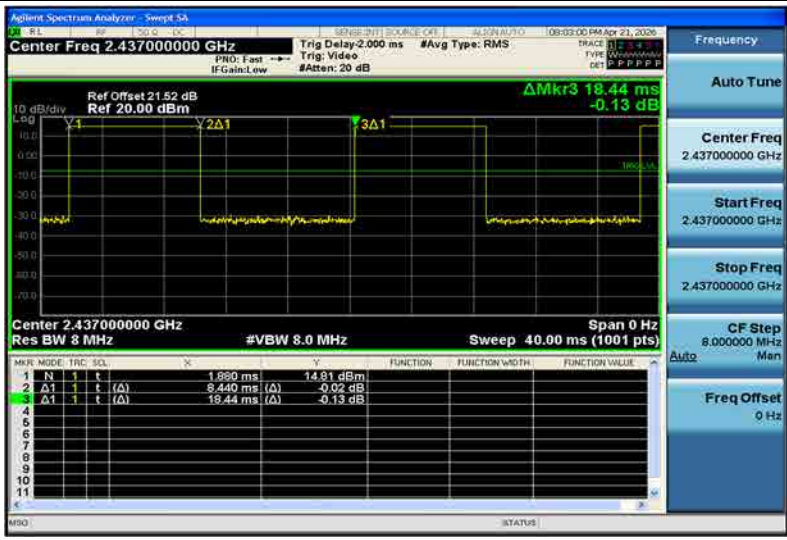
NTNV-11B-Ant1-2437
