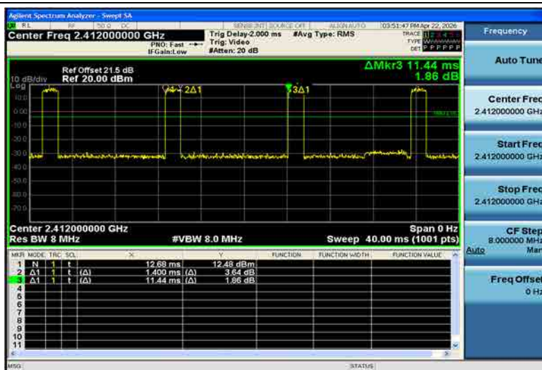
NTNV-11G-Ant1-2412
