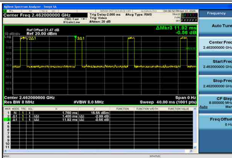
NTNV-11G-Ant1-2462
