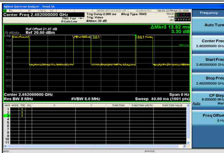
NTNV-11AX20SISO-Ant1-2462
