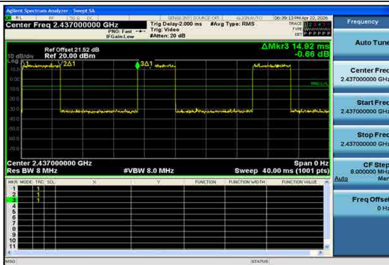
NTNV-11N40SISO-Ant1-2437
