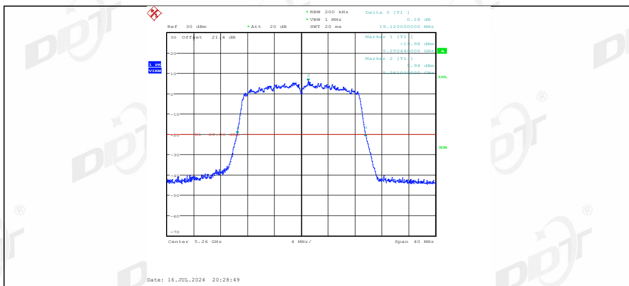
11AC20MIMO Ant2 5260
