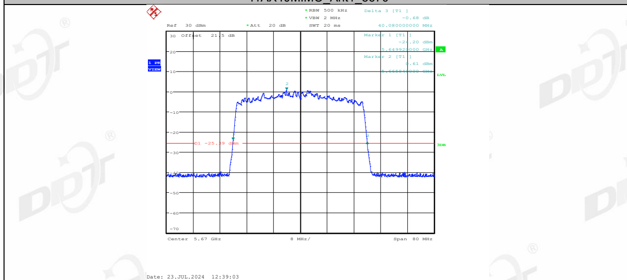
11AX40MIMO Ant2 5670
