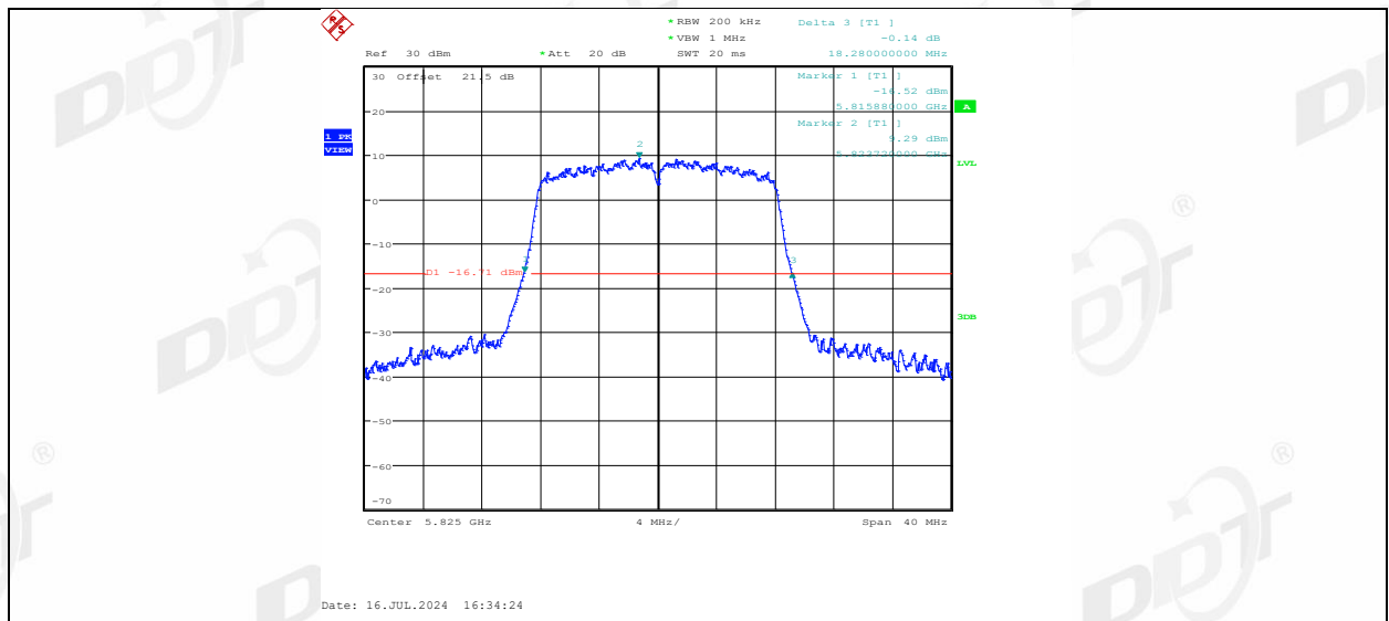
11A Ant2 5825
