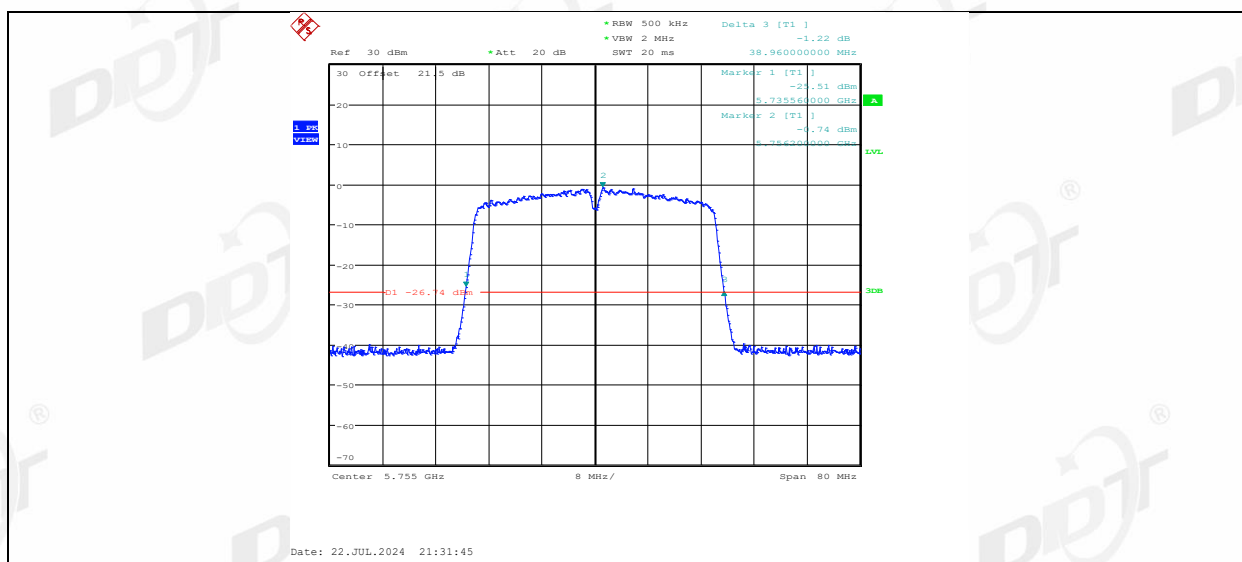
11AC40MIMO Ant2 5755
