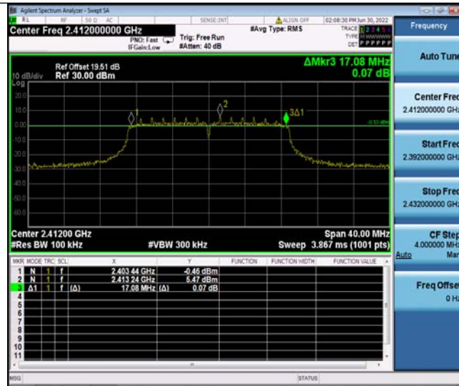
11N20SISO_Ant1_2412
