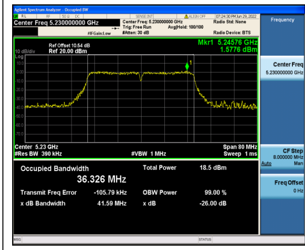
11ac (HT40) CH46
