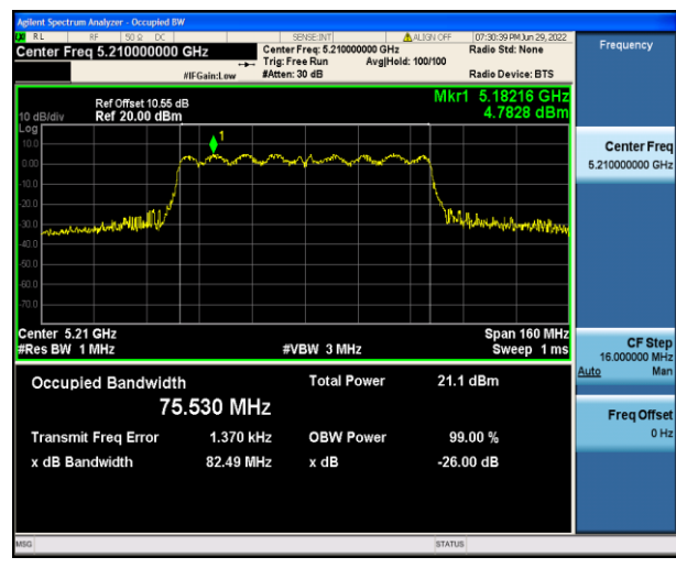
11ac (HT80) CH42
