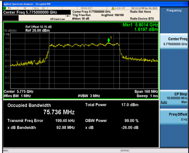
11ac (HT80) CH155
