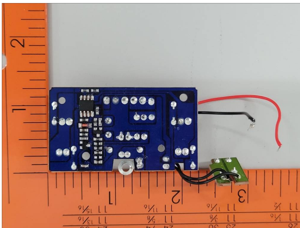
Internal view
