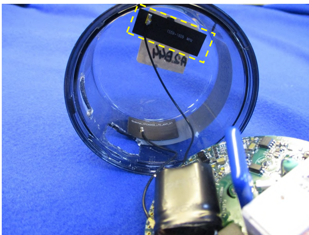
Photograph shows the EUTs GPS antenna (highlighted)
