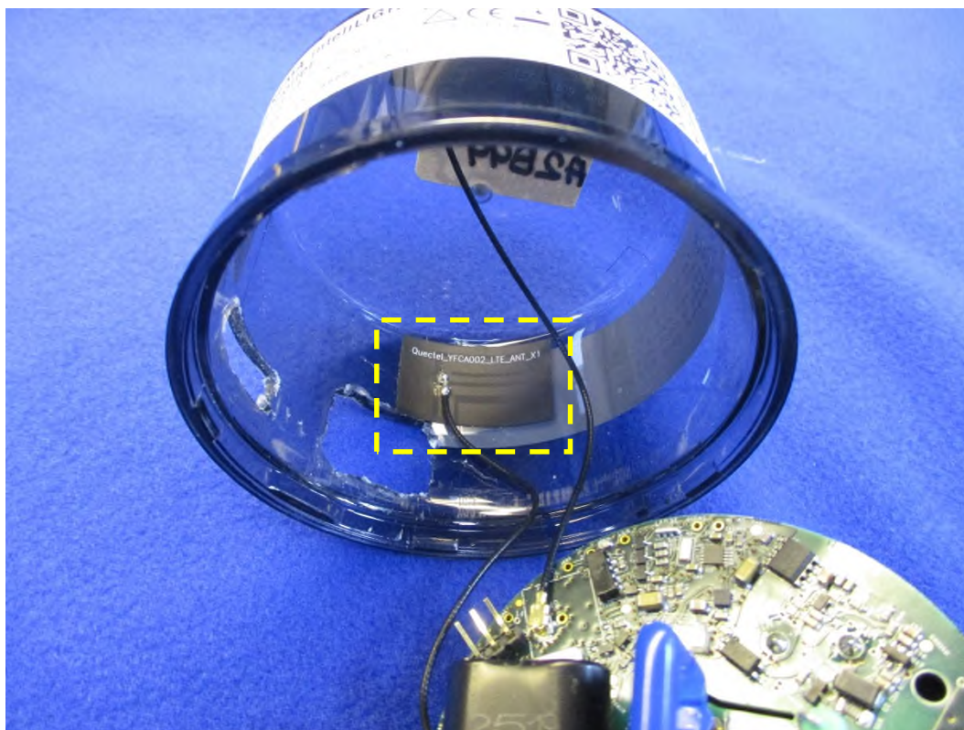
Photograph shows the EUTs cellular antenna (highlighted)
