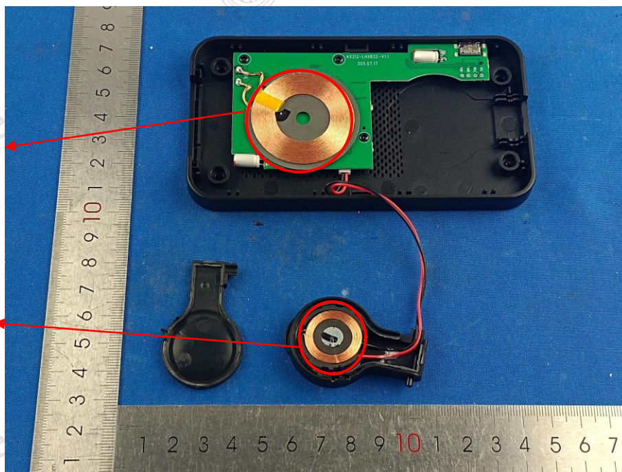
Coil 1(Airpods)
