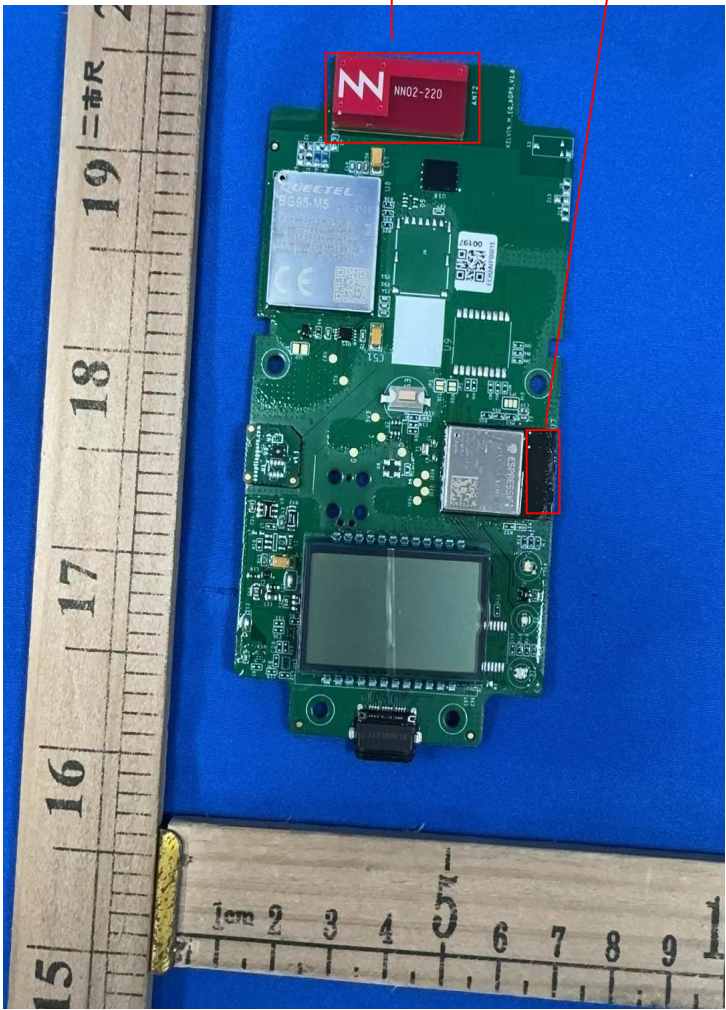
GSM antenna Wi-Fi antenna
