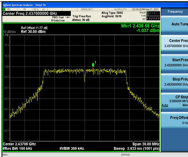
11G-Ant1-2437-0~Reference-PASS
