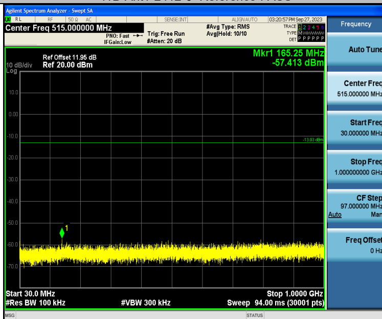
11B-Ant1-2412-0~Reference-PASS
