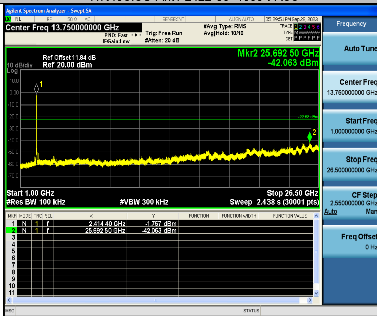
11N40SISO-Ant1-2422-1000~26500-PASS
