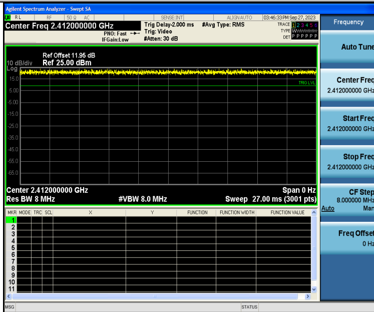
NTNV-11N20SISO-Ant1-2412
