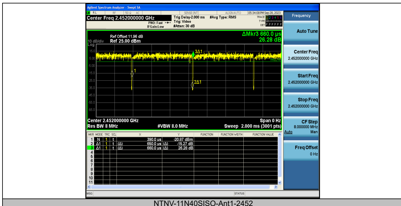
NTNV-11N40SISO-Ant1-2452
