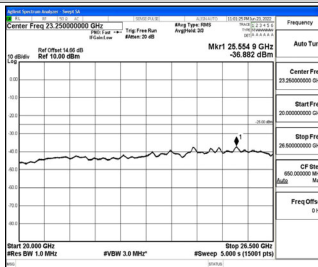
Band7-20MHz-16QAM-21350-1RB#0-Range6:20000~26500MHz
