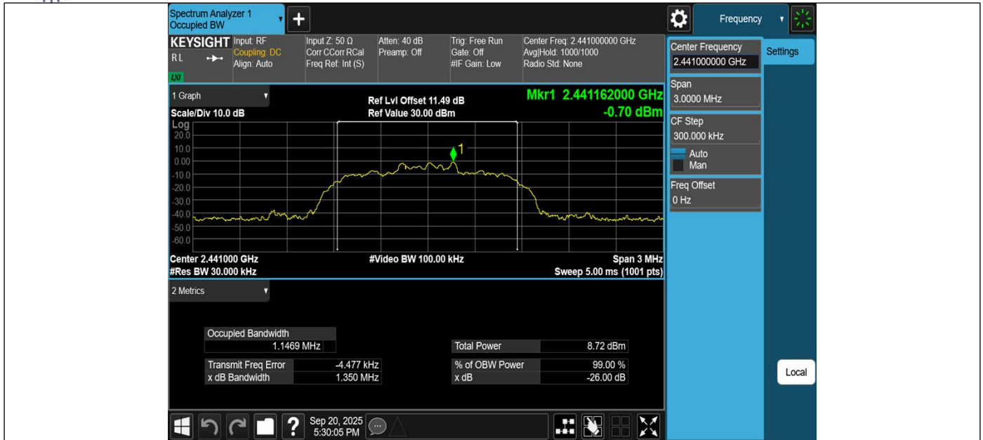
2DH5-Ant1-2441
