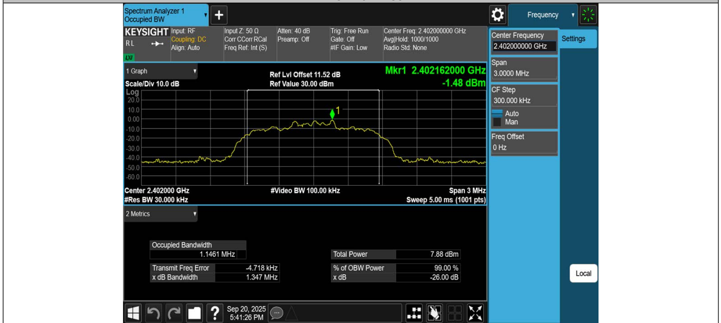
2DH5-Ant1-2402
