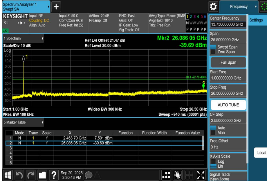
11B-Ant1-2462-1000~26500-PASS
