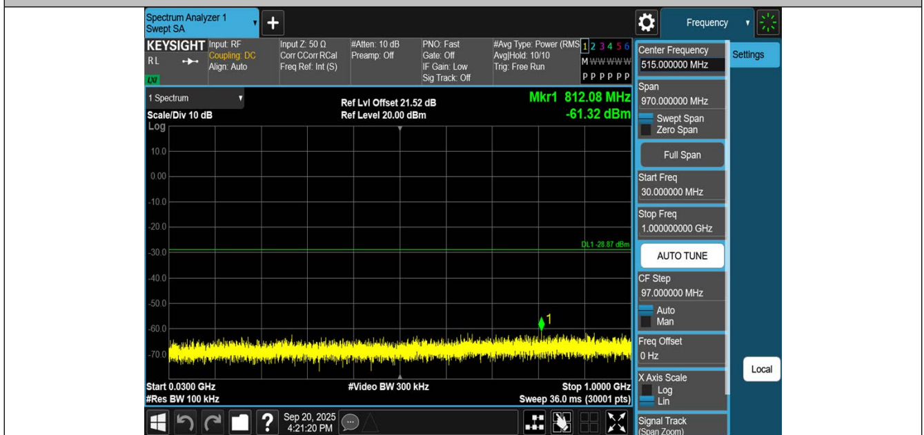
11N40SISO-Ant1-2437-30~1000-PASS
