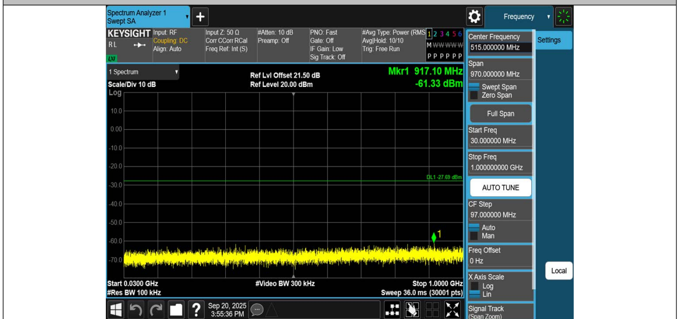
11N20SISO-Ant1-2412-30~1000-PASS
