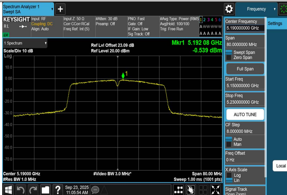
11AC40SISO-Ant1-5190-PASS
