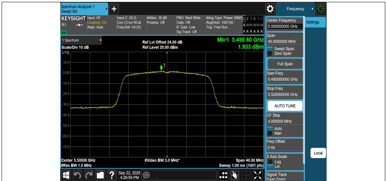
11N20SISO-Ant1-5500-PASS
