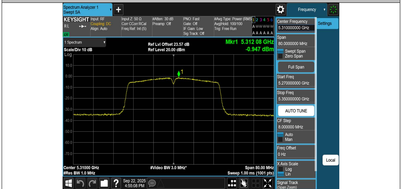
11N40SISO-Ant1-5310-PASS
