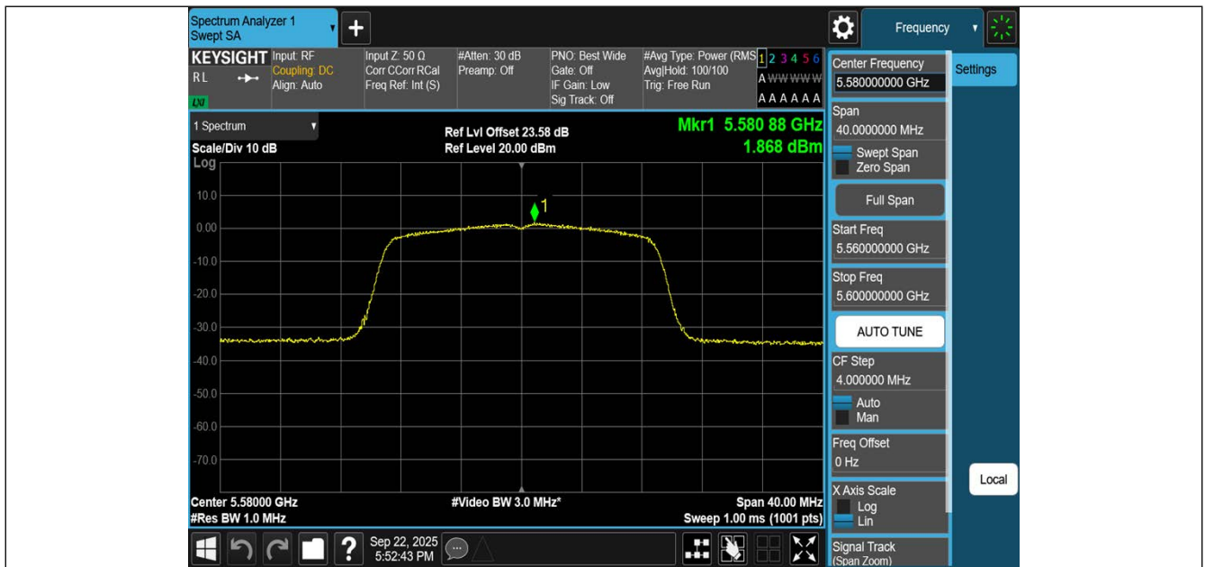
11AC20SISO-Ant1-5580-PASS
