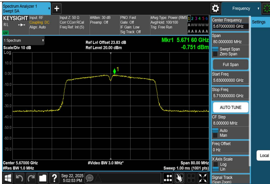
11N40SISO-Ant1-5670-PASS
