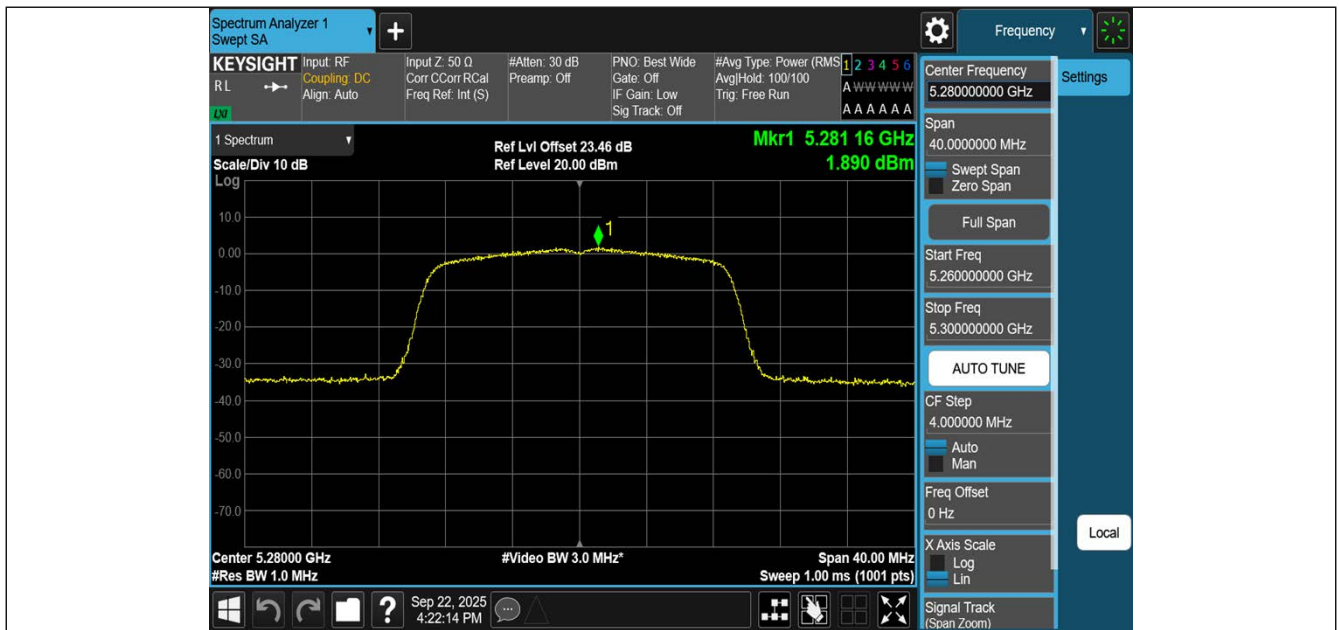
11N20SISO-Ant1-5280-PASS
