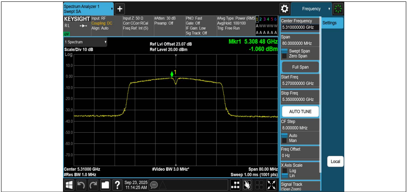
11AC40SISO-Ant1-5310-PASS
