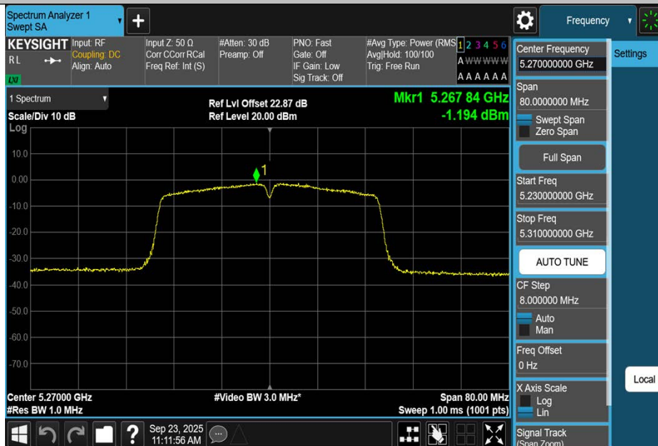
11AC40SISO-Ant1-5270-PASS
