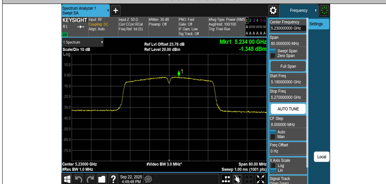
11N40SISO-Ant1-5230-PASS
