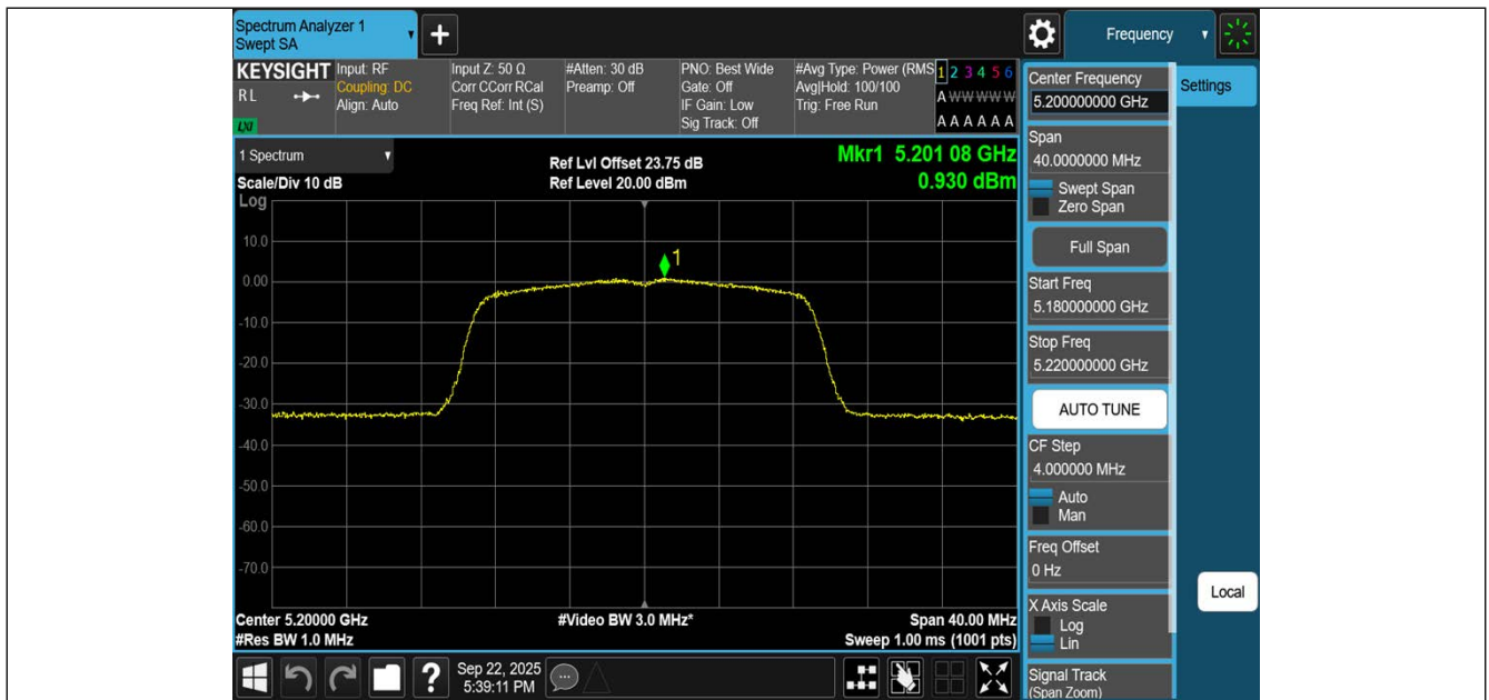
11AC20SISO-Ant1-5200-PASS
