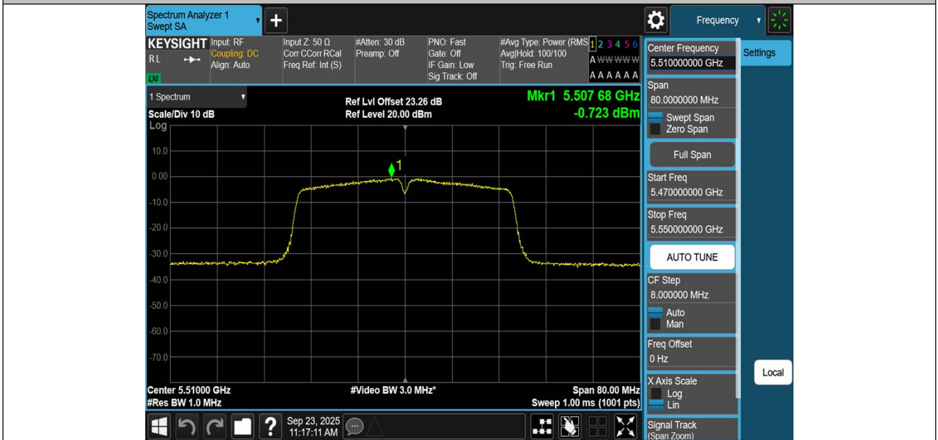
11AC40SISO-Ant1-5510-PASS
