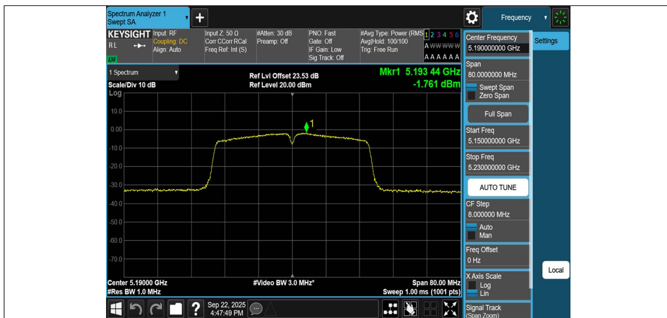
11N40SISO-Ant1-5190-PASS
