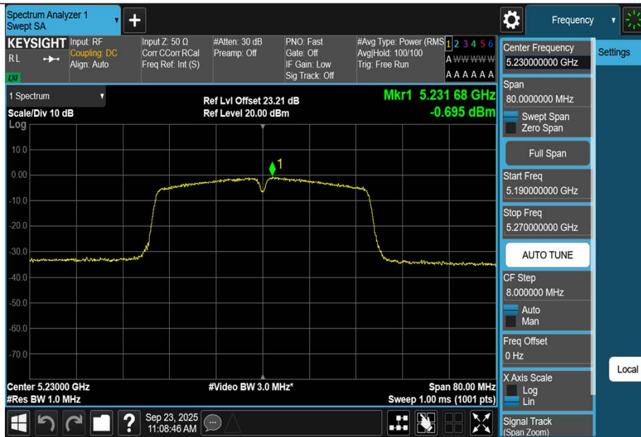
11AC40SISO-Ant1-5230-PASS
