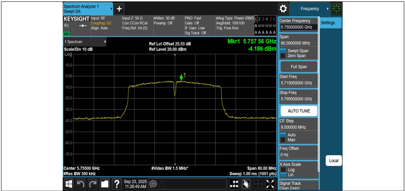
11AC40SISO-Ant1-5755-PASS
