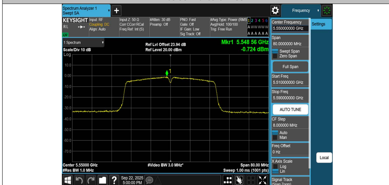
11N40SISO-Ant1-5550-PASS
