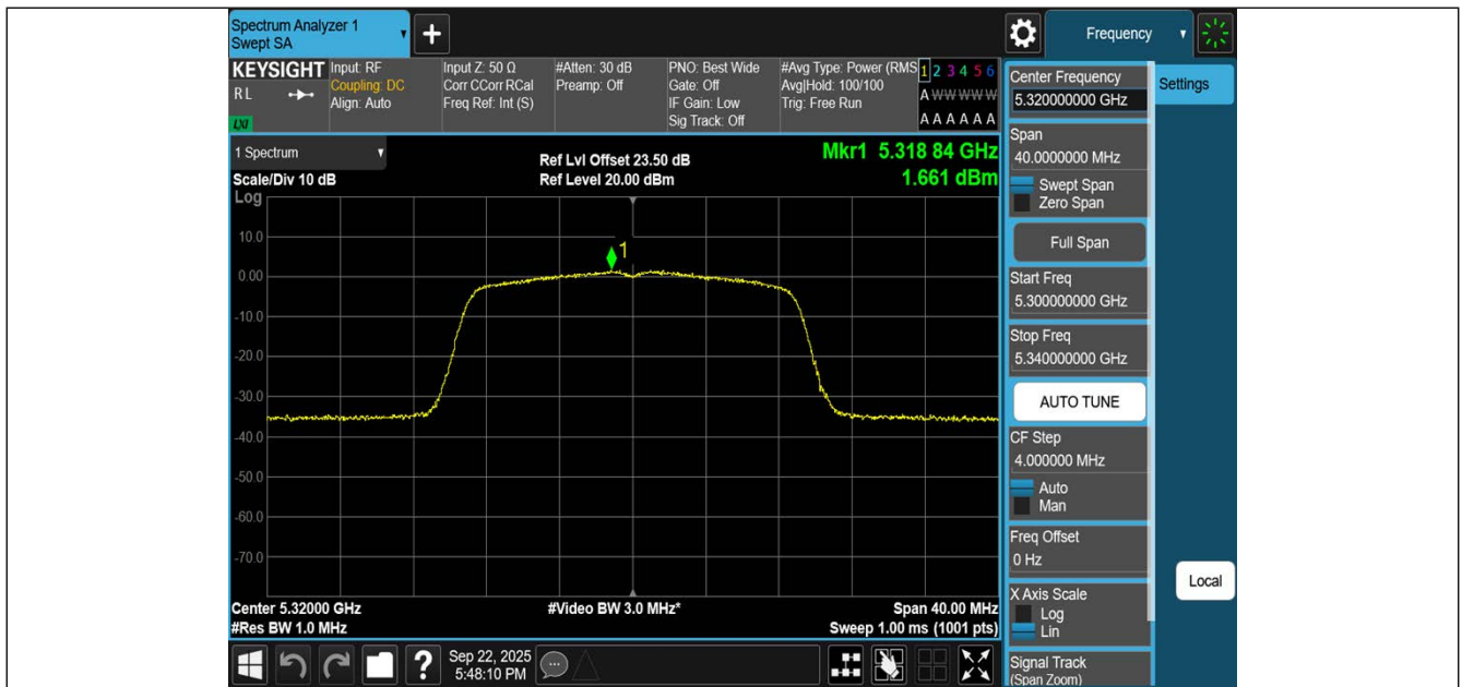
11AC20SISO-Ant1-5320-PASS
