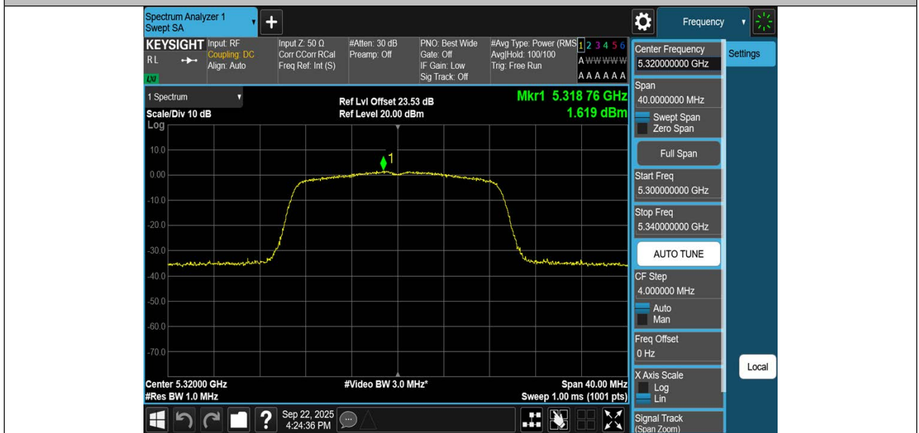
11N20SISO-Ant1-5320-PASS
