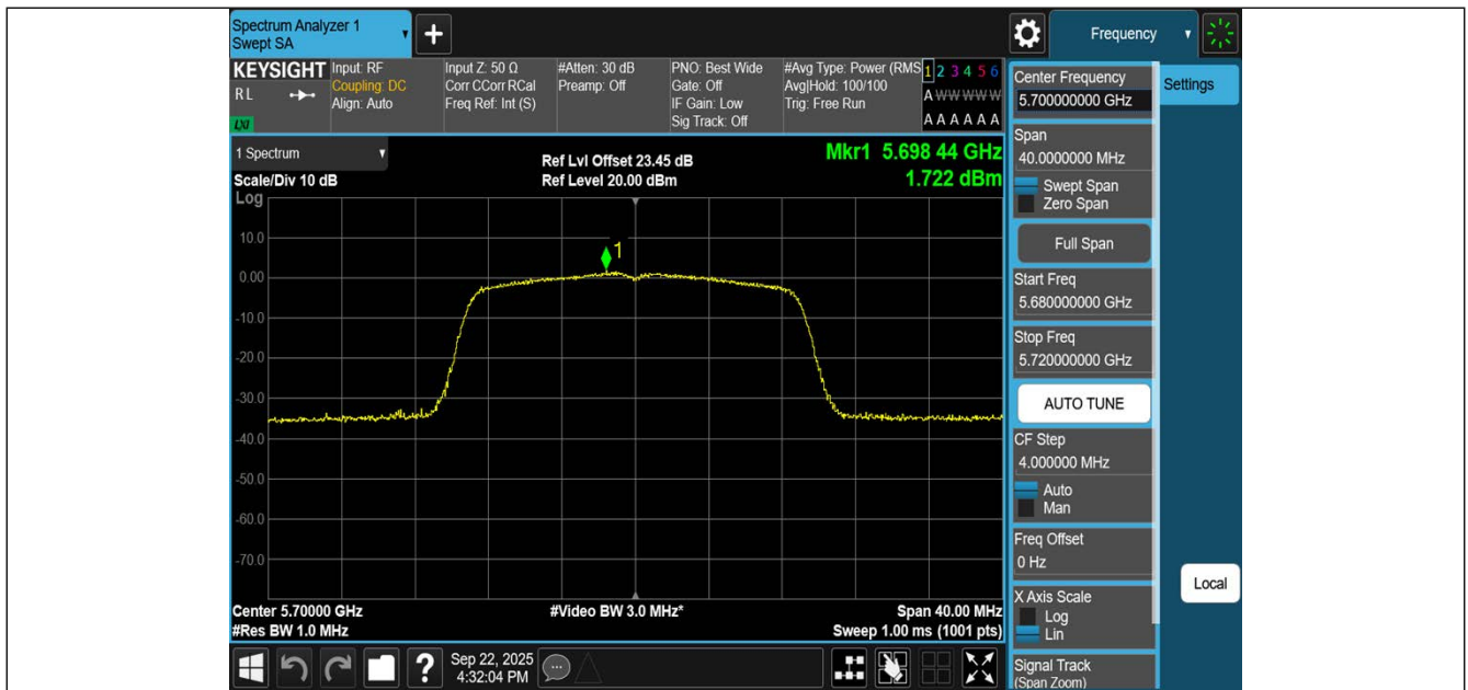
11N20SISO-Ant1-5700-PASS
