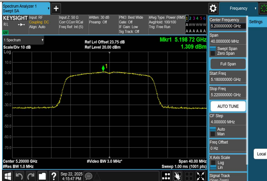
11N20SISO-Ant1-5200-PASS
