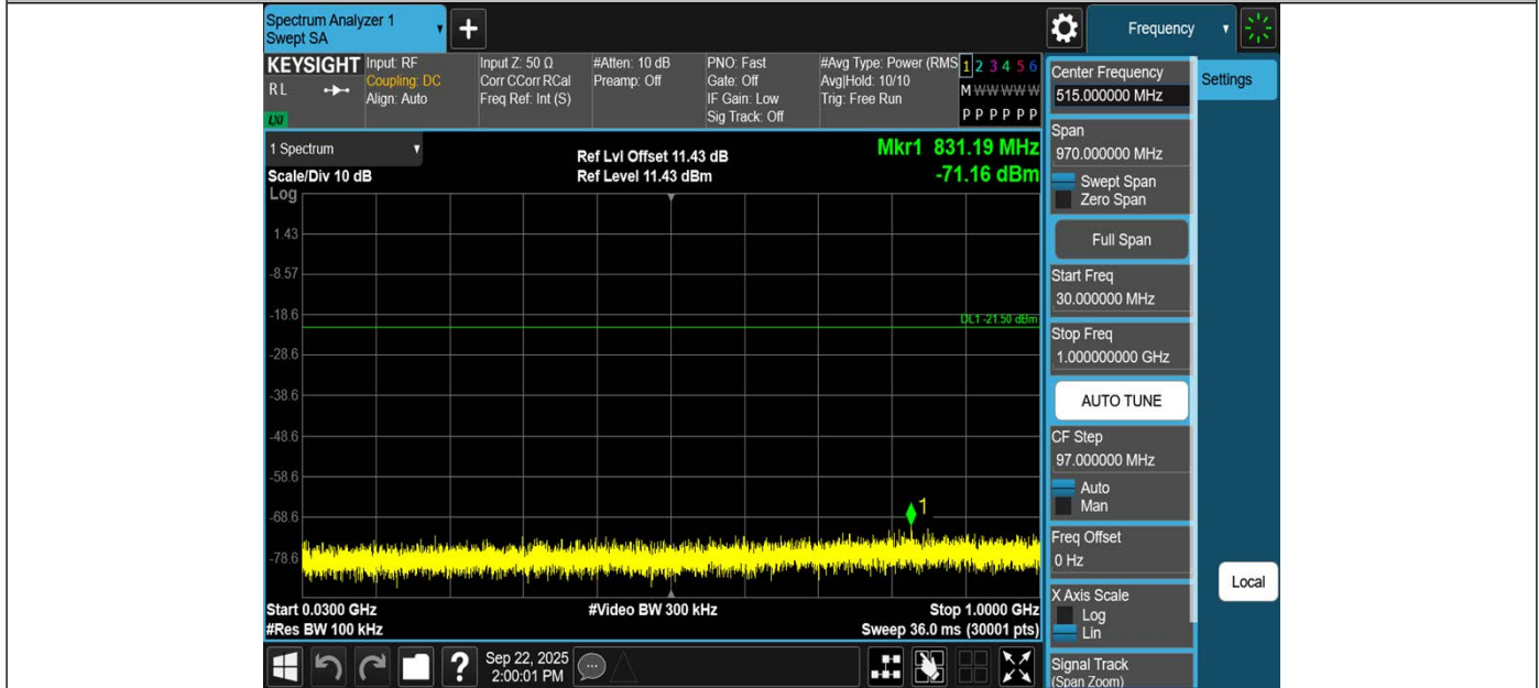
3DH5-Ant1-2480-30~1000-PASS
