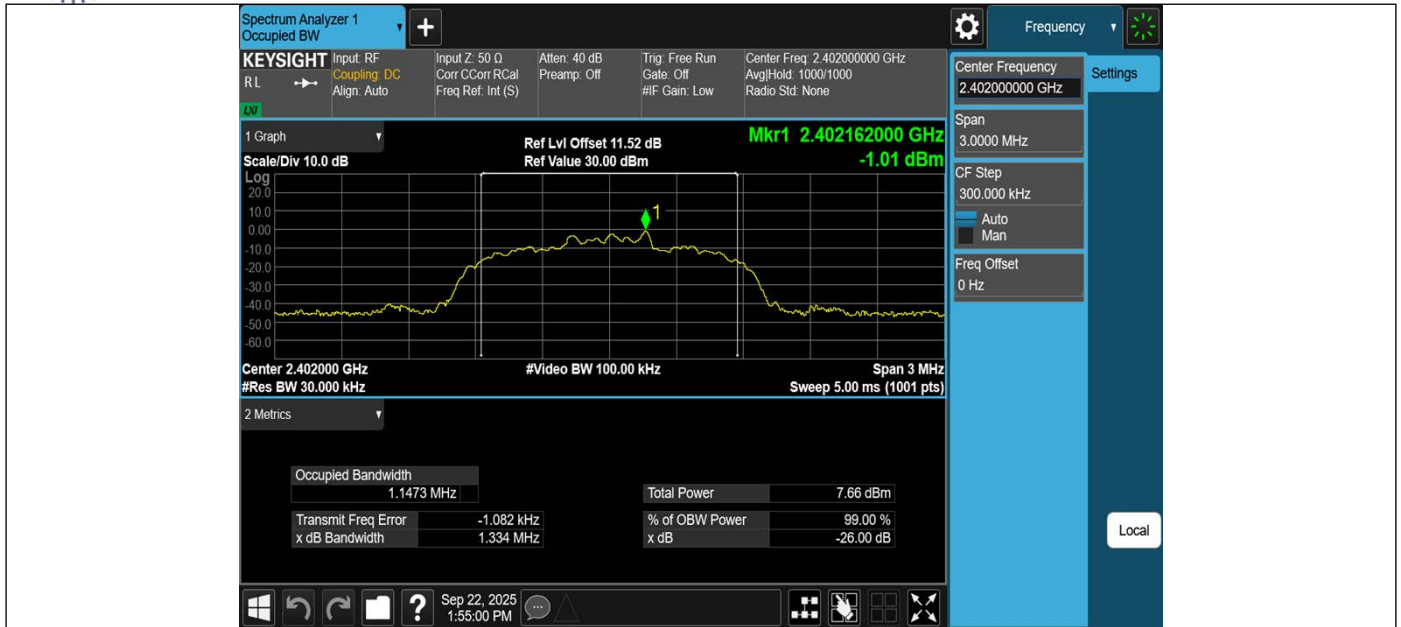
3DH5-Ant1-2402
