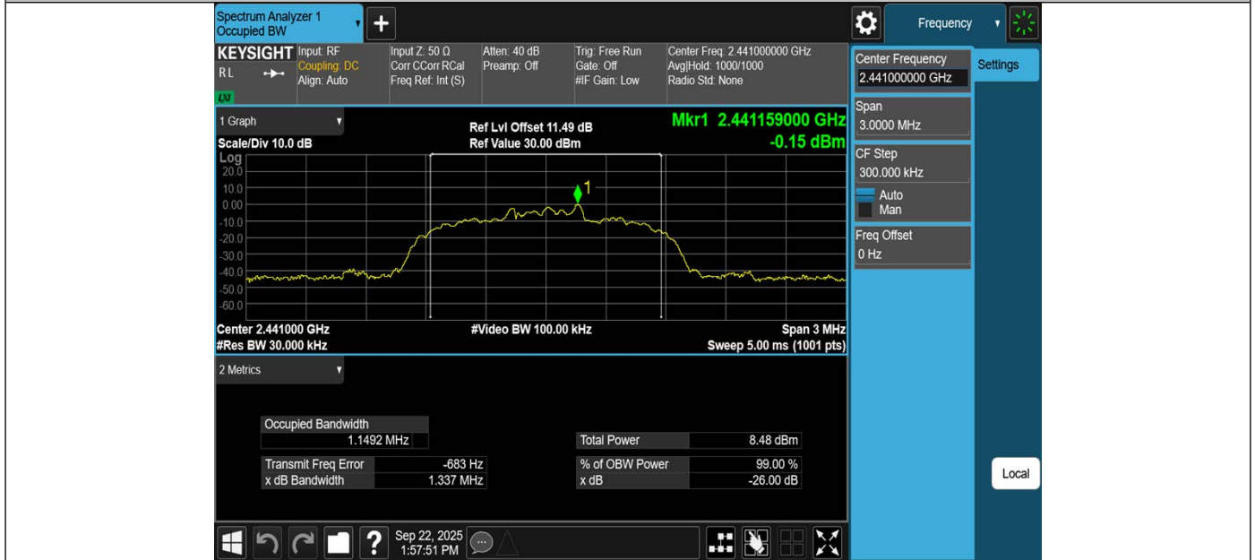
3DH5-Ant1-2441
