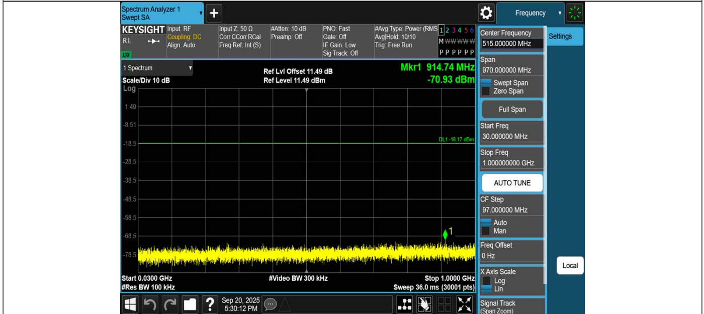
2DH5-Ant1-2441-30~1000-PASS
