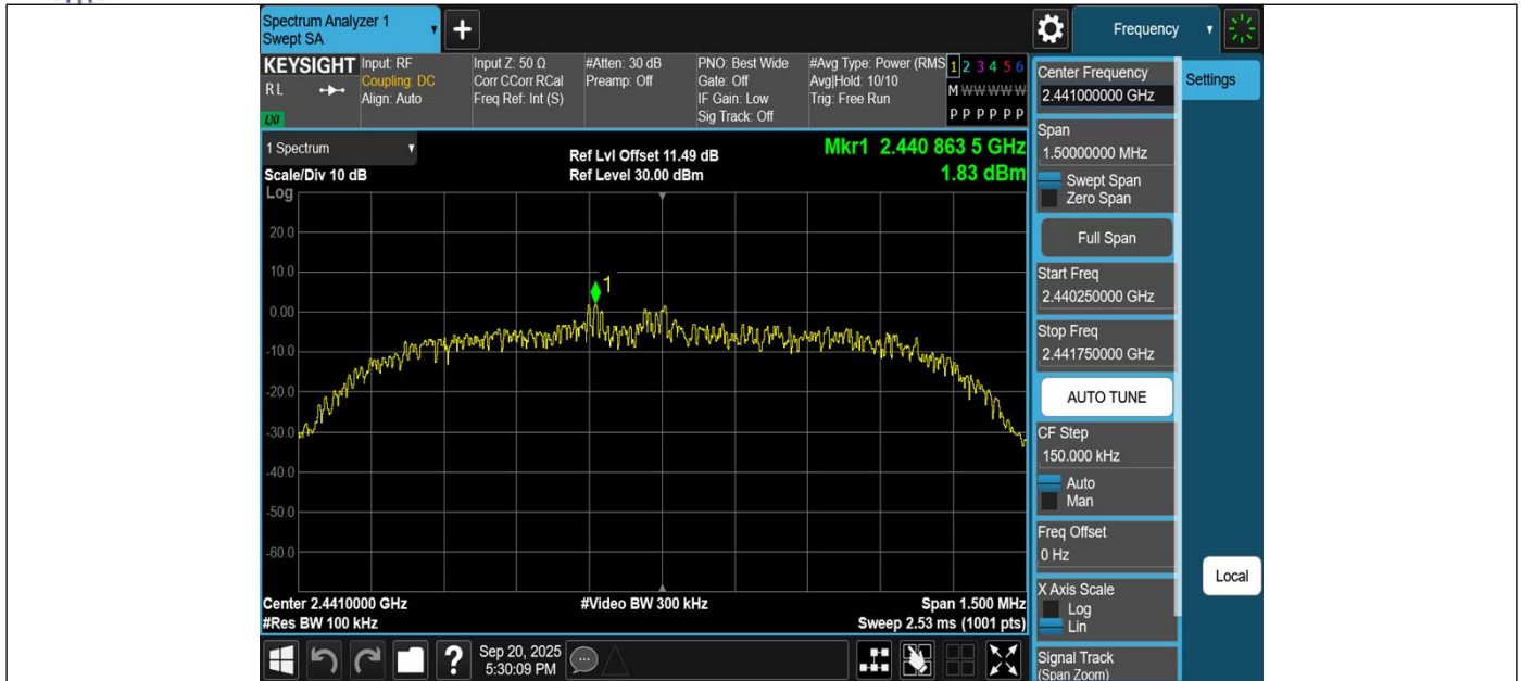
2DH5-Ant1-2441-0~Reference-PASS
