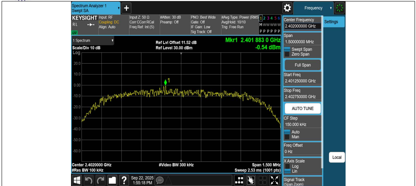
3DH5-Ant1-2402-0~Reference-PASS
