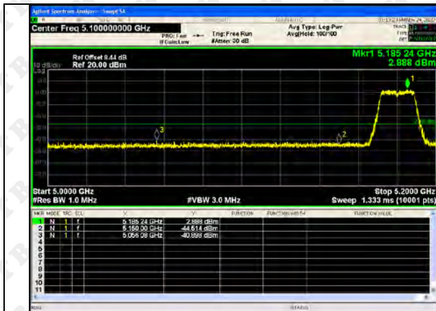
802.11n(HT40)-5190
