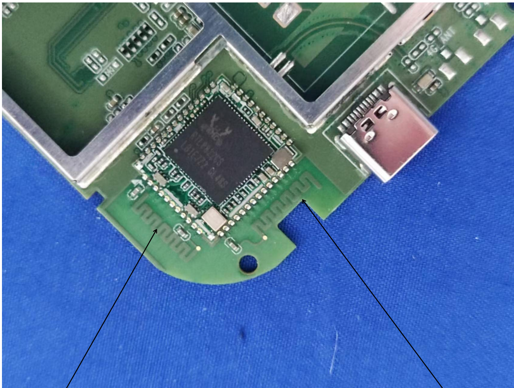
2.4G PCB Antenna
