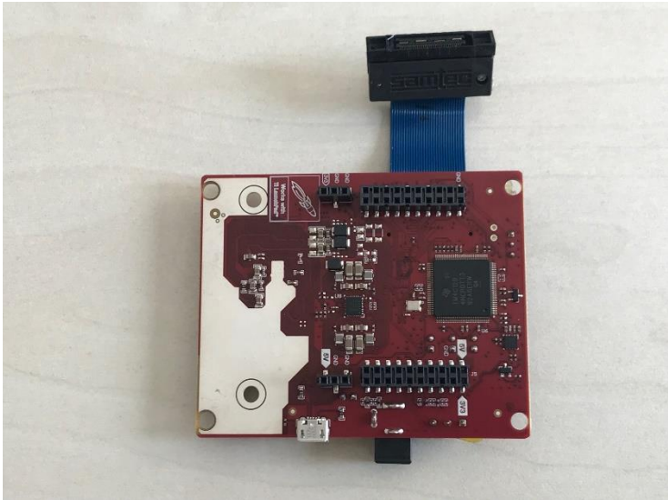
BaseBand back
