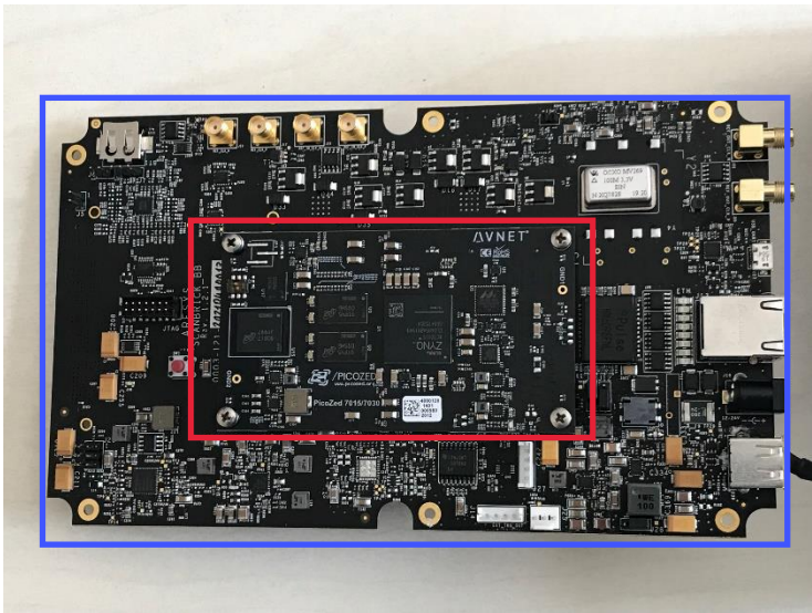
Picozed front
