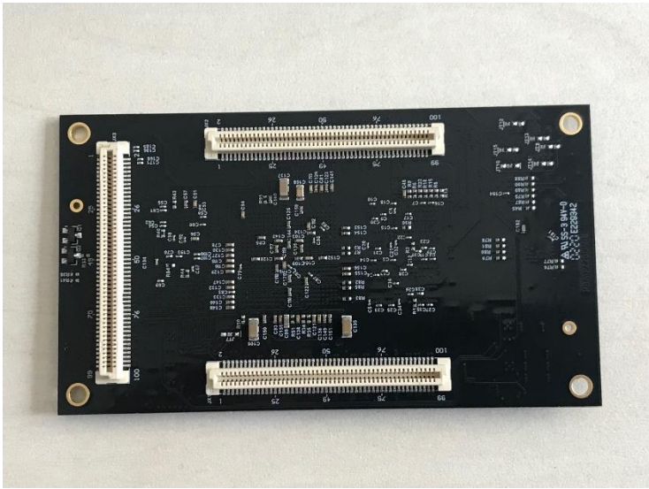
Picozed back
